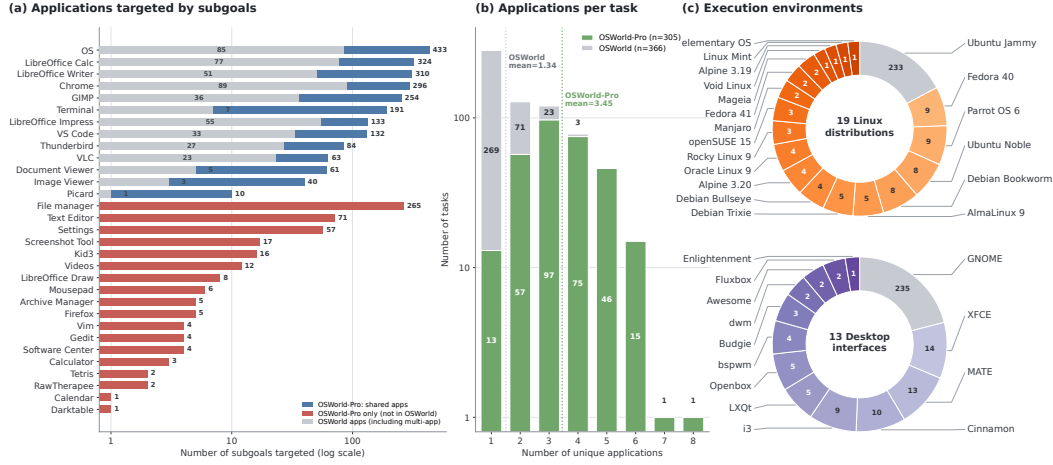
Figure 3: OSWorld-Pro Data Distribution: Compared with OSWorld, OSWorld-Pro covers a wider diversity of applications (31 vs 13), requires coordination between more applications in a single task (mean = 3.45 vs 1.34) and can show robustness of agents in more environments (19 Linux distributions + 13 Graphical interface vs Ubuntu Jammy with GNOME only) .
