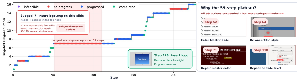
Figure 5: OSWorld-Pro reveals inefficiency of strong models such as Claude Opus 5 Max beyond what outcome-based evaluation alone (e.g. in OSWorld) can show. Opus 5 Max was stuck on multiple subgoals without any progress including once for 59 steps as it performed goal-irrelevant actions.
