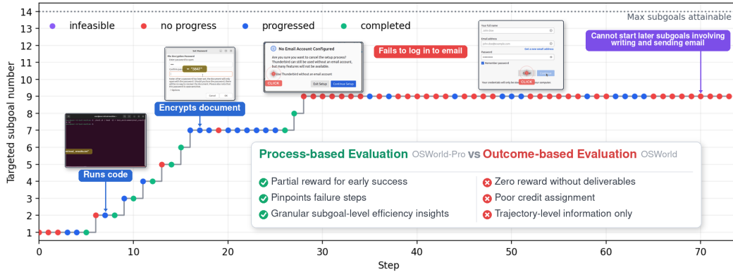
Figure 1: OSWorld-Pro provides partial reward for early success without requiring final deliverables, pinpoints specific failures and offers granular information on progress through sequentially dependent subgoals. Such advantages of Process-based evaluation for Computer Use Agents (CUAs) complements the limitations of outcome-based evaluations such as OSWorld.
