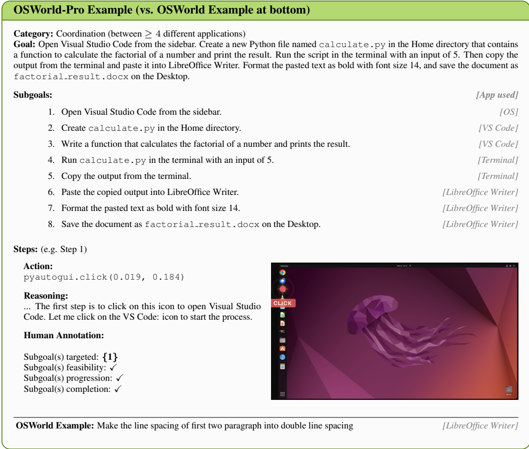
Figure 2: OSWorld-Pro Example compared with OSWorld Example. More examples in § A.
