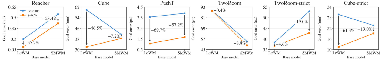
Figure 5: ACA substantially reduces the real planning error across environments, indicating improved alignment between the planning cost and the actual consequences of executed actions.
