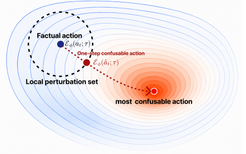
Figure 3: Illustration of the Action Consequence Alignment (ACA) principle.
