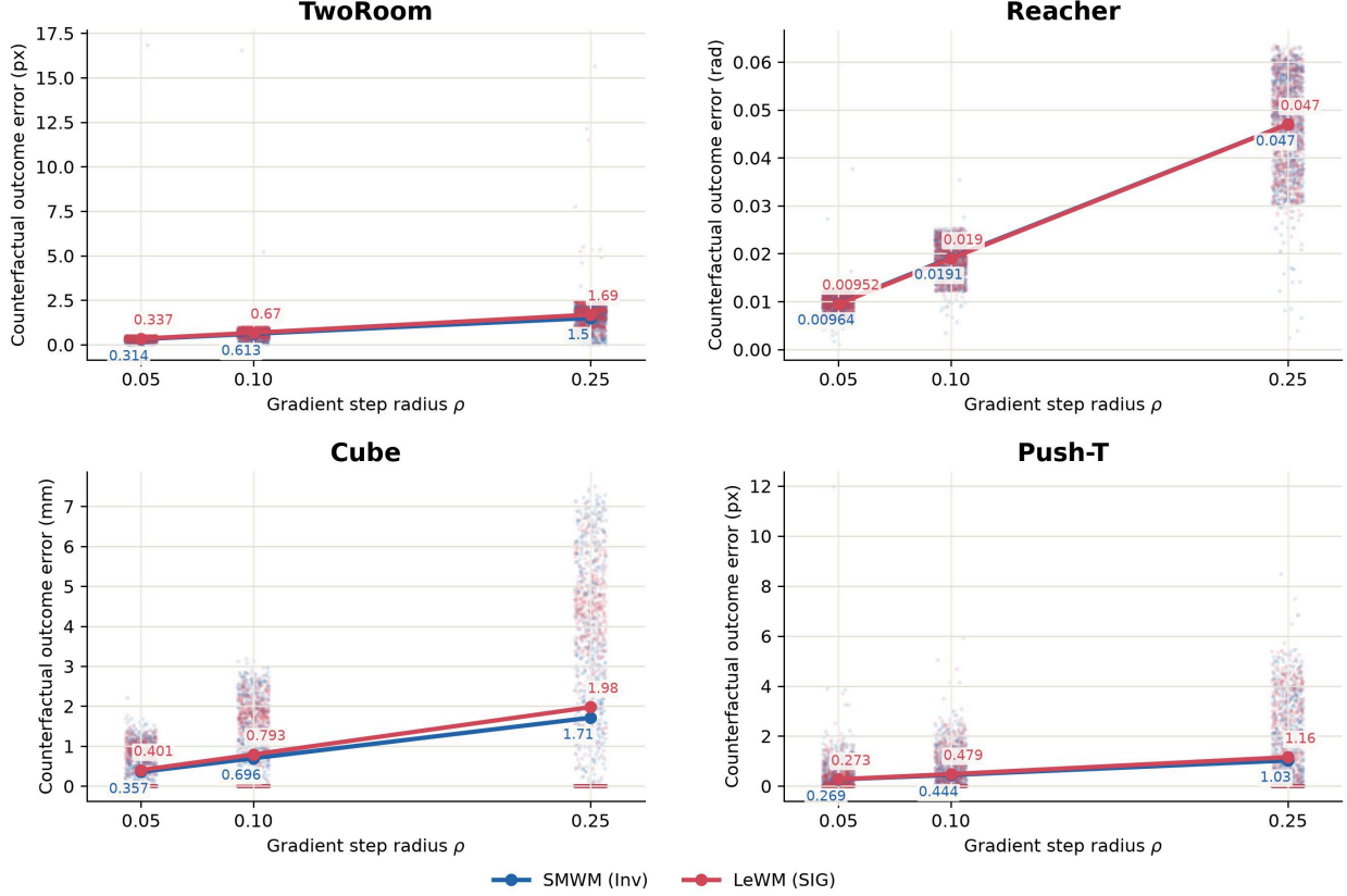
Figure 10: Physical outcome deviations of lower-error counterfactual actions. We execute searched alternatives that receive lower prediction error than the factual actions, starting from the corresponding recorded simulator states. Each model–radius setting contains 1,000 evaluated transitions. Translucent dots show individual outcome deviations from the factual targets, and solid lines connect their means. Blue and red denote SMWM and LeWM, respectively. Outcome deviations are measured using environment-specific simulator state distances, with units indicated on the axes. The alternatives receive lower model errors despite producing nonzero mean deviations from the factual outcomes.
