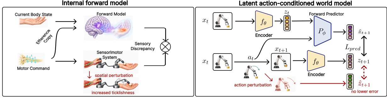
Figure 1: Structural correspondence between biological forward models (left) and latent action-conditioned world models (right). Both use an action signal to predict the resulting consequence and use the discrepancy between predicted and observed outcomes to update the internal model.
