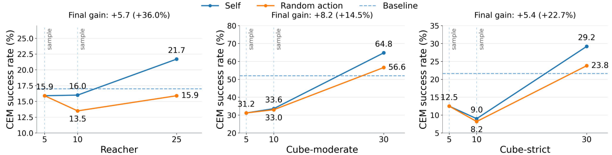
Figure 8: ACA sampling enables better self-improved performance than random sampling.
