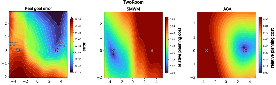
Figure 4: Visualization of planning-cost alignment on TwoRoom, more visualization results is shown in Appendix F.
