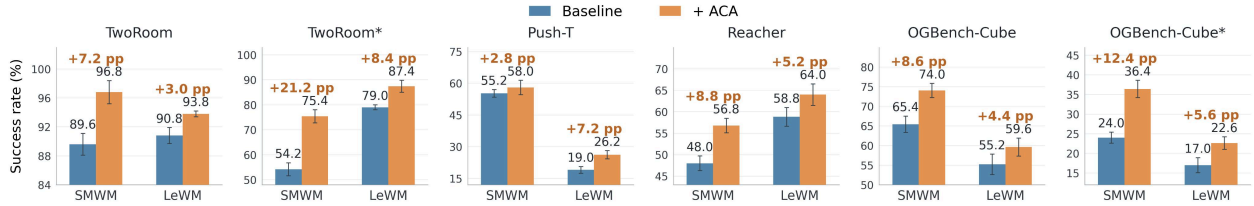
Figure 6: ACA achieves reliable planning under the limited data settings.
