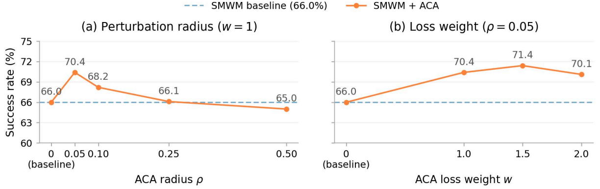
Figure 12: Sensitive Analysis on Reacher
