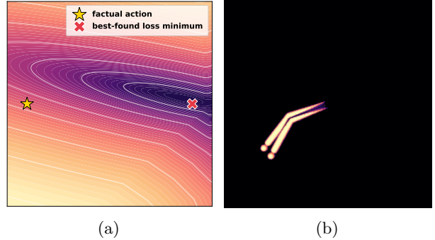
Figure 2: (a) Local action-loss landscape for a fixed Reacher transition. The landscape is a two-dimensional slice of the 10-dimensional five-step action space. (b) Absolute pixel-wise difference between the MuJoCo renders obtained by executing the two action sequences for five steps from the same recorded initial simulator state.
