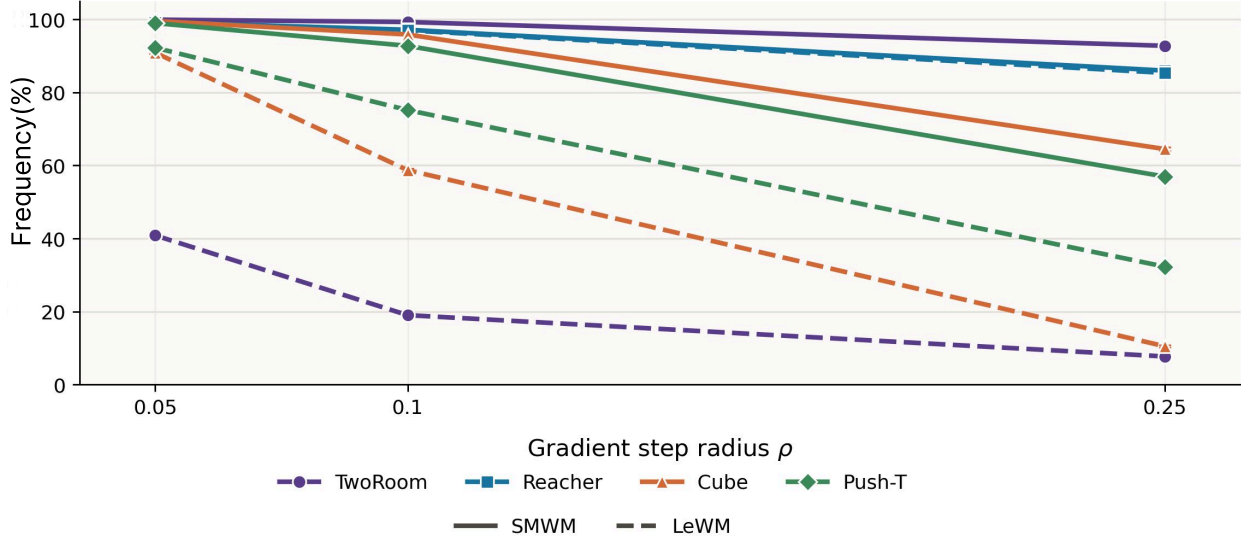
Figure 9: Frequency of lower-error alternatives. Frozen SMWM and LeWM models are evaluated on 10,000 transitions per environment. At each nominal perturbation radius, an alternative action is constructed using one normalized gradient-descent step from the factual action. The plotted frequency measures the fraction of transitions for which this alternative receives lower prediction error against the same observed future.
