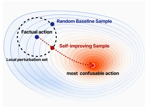
Figure 7: Overview of ACA self-improving sampling method and random sampling baseline.
