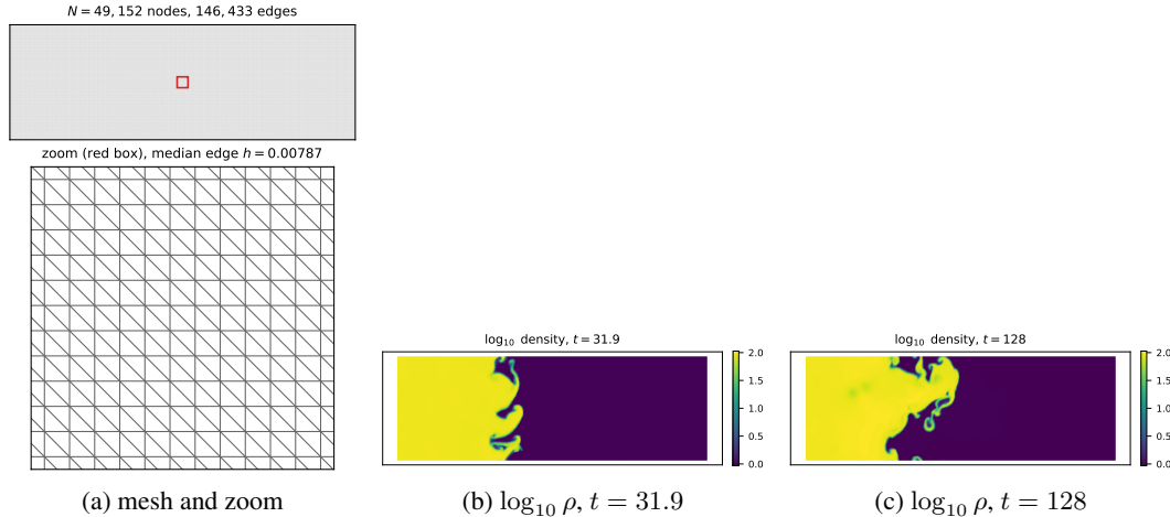
Figure 10: TRL2D: the regular mesh twin with the zoom region marked in red and the zoomed mesh below it (left), and \log_{10} density at two times along a t_{\text{cool}} = 0.18 trajectory. The Well mesh twins are triangulations of the original grids, so grid and mesh tokenisers see exactly the same samples.
