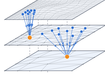
Figure 3: The mesh hierarchy, finest level at the top. Encoder steps gather onto virtual anchors; decoder steps reuse the same edges in reverse.
