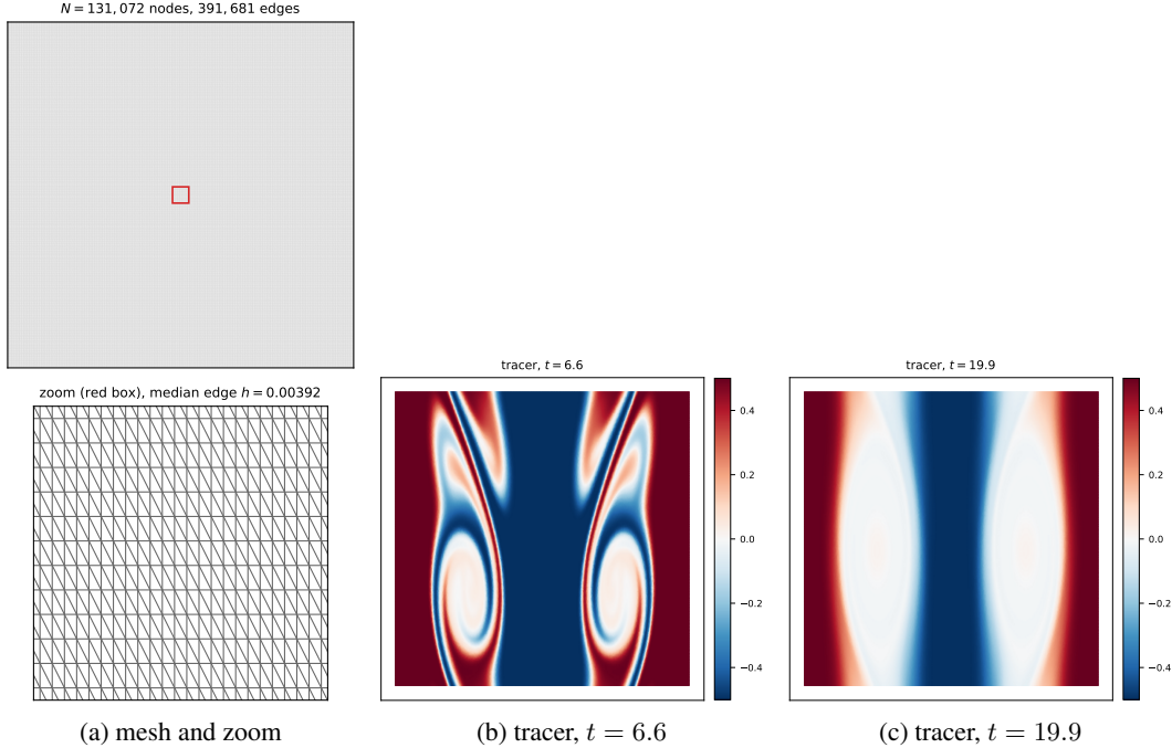
Figure 12: Shear flow: the mesh twin with zoom (left), and the tracer at two times along a Re = 10^4 , Sc = 1 trajectory that develops Kelvin–Helmholtz billows.
