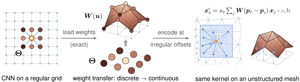
Figure 2: Schematic overview of the MNC layer. MNC loads a pretrained CNN’s weights into a continuous spline and evaluates the same kernel at physical offsets on an unstructured mesh.
