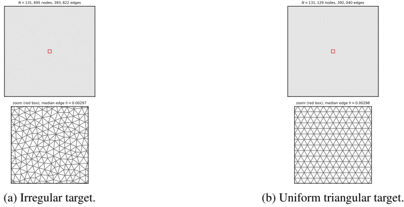
Figure 18: The shear-flow target meshes used for tokeniser transfer. Source-grid fields are resampled onto their nodes.
