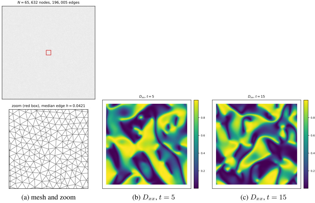
Figure 14: Active matter on the Experiment 1 irregular mesh (65,632 nodes, 196,005 edges, node count matched to the grid): the mesh with the zoom region marked in red (left), and the orientation-tensor component D_{xx} at two times along a \zeta = 9 , \alpha = -3 test trajectory, bilinearly resampled onto the mesh nodes. The concentration is nearly uniform ( 1 \pm 5 \cdot 10^{-4} ), so a tensor channel is shown.
