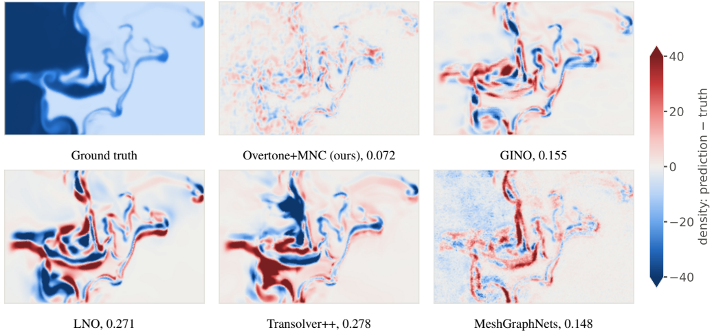
Figure 5: Zero-shot one-step density error on the irregular TRL2D mesh. Numbers are the window’s density VRMSE; predicting no change (persistence) scores 0.308.
