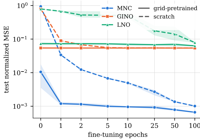
Figure 19: Companion to Figure 17 on the uniform triangular lattice. Solid curves use grid-pretrained weights; dashed curves start from random initialisation. Bands show variation across three seeds. Pretraining is not included in the horizontal-axis mesh-training budget.
