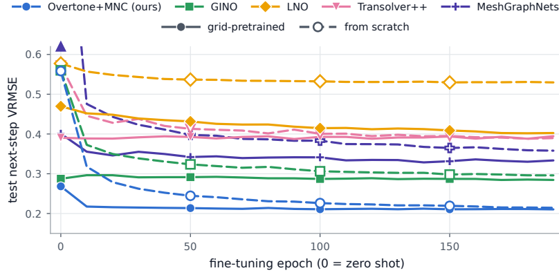
Figure 6: Test next-step VRMSE (mean) on the irregular TRL2D mesh against fine-tuning epoch. Grid-pretrained models are marked in solid lines and randomly initialised ones in dashed lines.
