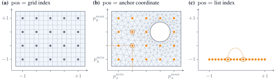
Figure 8: Coordinate rotary position embedding for mesh tokens: only the source of pos changes. (a) On the grid, pos = linspace( -1, 1, \cdot ) along each axis. (b) After retrofitting, pos is the anchor coordinate, rescaled by the outermost anchors (6). The window covered by the hole emits no token. On a lattice this recovers the angles of (a) exactly. (c) The stock axial embedding would place the flat list of anchors along one axis, separating vertical neighbours (ringed) and collapsing the second axis.
