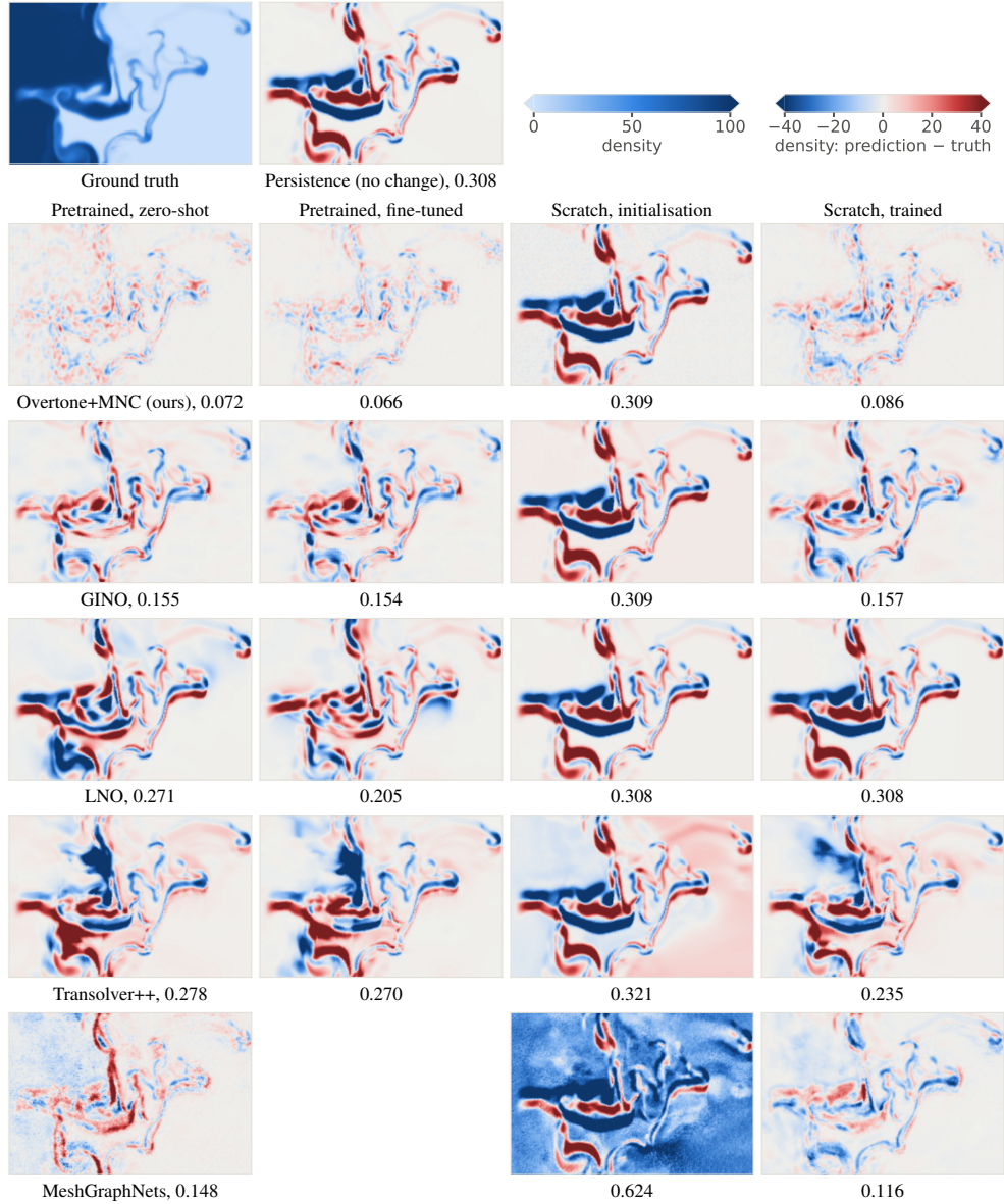
Figure 16: One-step density error (prediction – truth) on the irregular TRL2D mesh, test trajectory 7, frame 79: grid-pretrained models zero-shot and after fine-tuning, and the same architectures trained from scratch, at initialisation and after 20k updates. Numbers are the density VRMSE of this window. The fine-tuned MeshGraphNets panel was not exported for this window.
