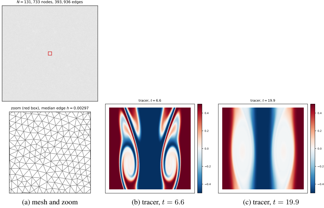
Figure 13: Shear flow on the Experiment 1 irregular mesh (131,733 nodes, 393,936 edges, node count matched to the grid): the same Re = 10^4 , Sc = 1 tracer snapshots as Figure 12, bilinearly resampled onto the mesh nodes (trajectory from the official validation file; Experiment 1 itself uses the trajectory-level resplit of the training files).
