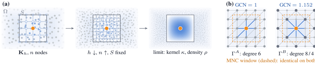
Figure 4: Discretisation invariance of MNC. (a) Refining kernel spacing and mesh together (Proposition 2). In the limit MNC corresponds to the continuous kernel \kappa and the mesh enters only through its sampling density \rho . (b) Two triangulations of the same vertices. The GCN neighbourhood of the origin is shown in blue. On the constant field the degree-normalised GCN returns 1 and 1.152 at the origin (9), whereas the MNC window (dashed) yields identical outputs.
