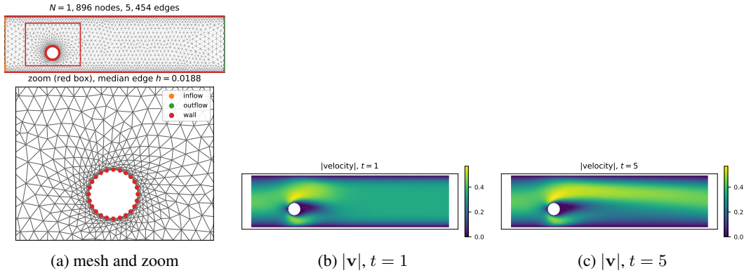
Figure 15: Cylinder flow: one of the per-trajectory meshes, with inflow, outflow and wall nodes marked in the zoom (left), and velocity magnitude at two times.
