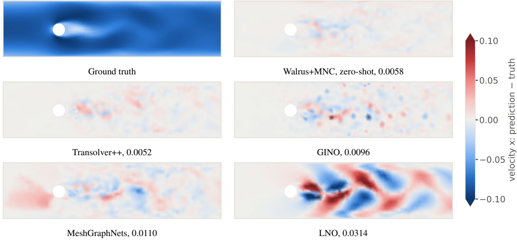
Figure 7: Error in next-step x -velocity prediction on cylinder flow. Numbers are the window's x -velocity VRMSE; predicting no change (persistence) scores 0.0314.
