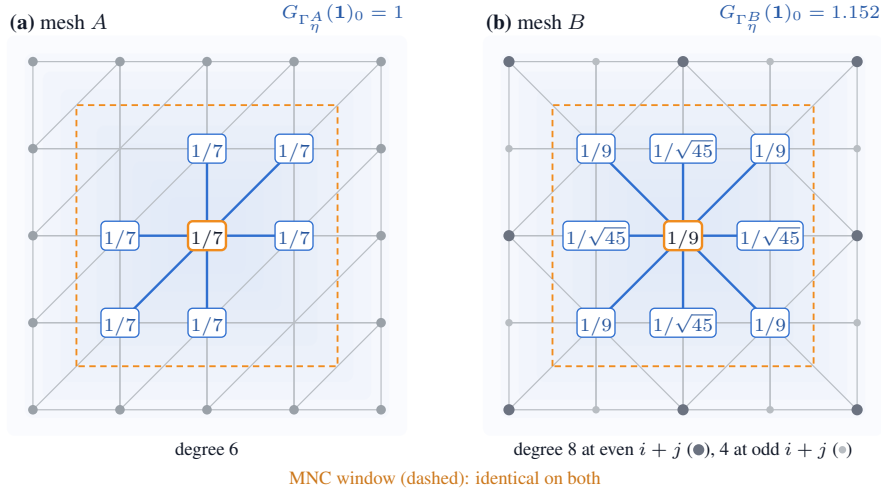
Figure 9: Meshes A and B near the origin. Each vertex in the origin’s GCN neighbourhood (blue) is labelled with its contribution to G_{\Gamma}(\mathbf{1})_0 , the origin’s own label being its self-loop.
