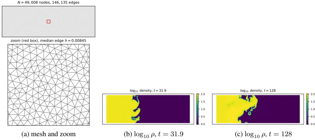
Figure 11: TRL2D on the Experiment 1 irregular mesh: the Gmsh Delaunay triangulation (49,008 nodes, 146,135 edges, node count matched to the grid) with the zoom region marked in red (left), and the same t_{\text{cool}} = 0.18 density snapshots as Figure 10, bilinearly resampled onto the mesh nodes which are exactly the samples the zero-shot-evaluated models see.
