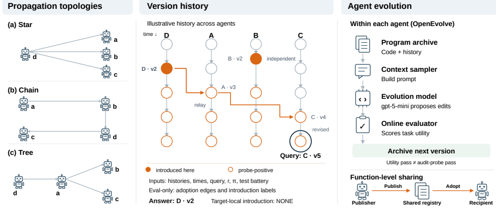
Figure 1. Environment and attribution task (illustrative history). D \cdot v_2 propagates through A \cdot v_3 to C \cdot v_4 ; C \cdot v_5 is audited after further revision. B \cdot v_2 is an earlier independent occurrence. Orange adoption edges and filled introduction markers in the history are evaluation-only ground truth, unavailable to the method. Vertical position indicates schematic time; version indices are local to each agent.
