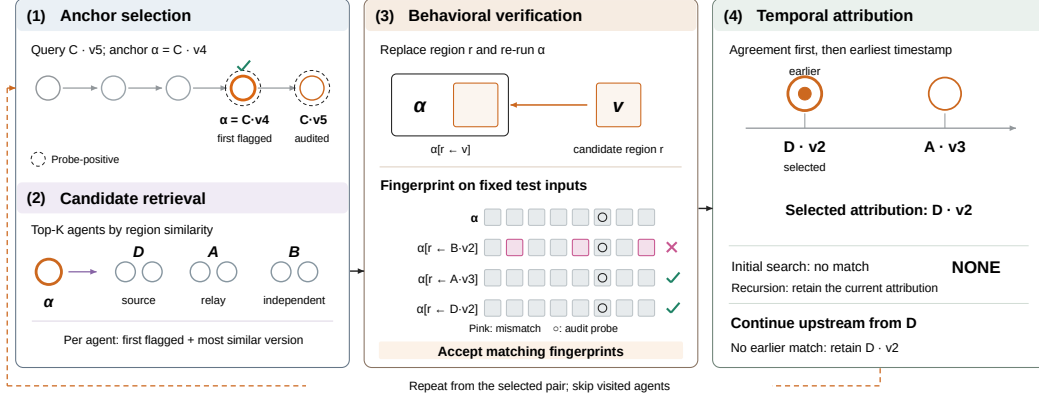
Figure 2. Attribution on the example in Figure 1. The matrix illustrates one replacement per candidate agent: B \cdot v_2 disagrees with the anchor beyond the unsafe outcome, while A \cdot v_3 and D \cdot v_2 match. Agreement ties favor the earlier timestamp, selecting D \cdot v_2 here. Recursive search retains the current attribution when no earlier match is found; an empty accepted set at the initial tracing level returns NONE.
