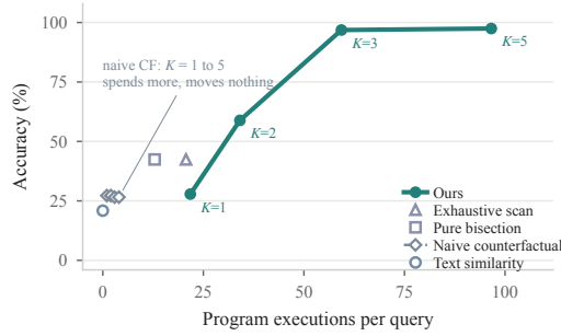
Figure 5. Accuracy and mean program executions per query on the core set. Curves vary K for the two counterfactual methods; other methods use fixed configurations.
