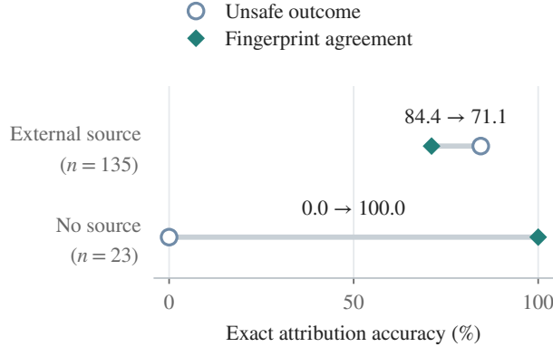
Figure 4. Fingerprint matching versus unsafe-outcome reproduction on external-source and no-source queries. Localization and temporal selection are fixed.
