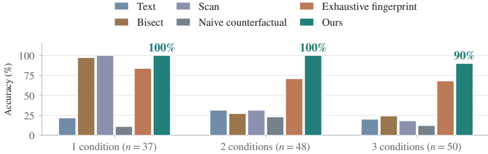
Figure 3. Accuracy on 135 external-source queries, grouped by the number of attribution conditions. Table 2 reports the individual combinations.
