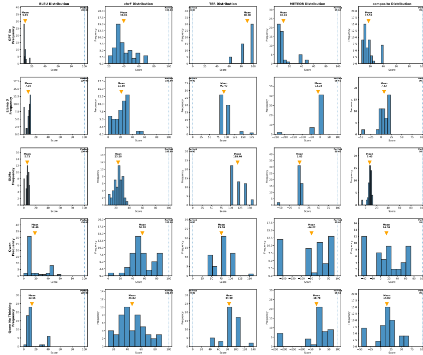
Figure 23: Sentence-level translation quality across five language models (GPT-4o, Llama 3, OLMo, Qwen, and Qwen without thinking) evaluated using BLEU, chrF, TER, METEOR, and a composite score. Each histogram shows the distribution of metric scores over 50 LLM-generated responses to the translation prompt, with each response truncated to its first 41 characters to match the length of the source sentence ("Mary gjyqazkjkx pxmqiMary. pxmqiMary qtojkx"). The orange triangle denotes the model mean, and the dotted vertical line denotes the upper-bound score obtained when the hypothesis exactly matches the reference (BLEU = 100.0, chrF = 100.0, TER = 0.0, METEOR = 99.6, composite = 99.9). Higher values indicate better performance for BLEU, chrF, METEOR, and the composite score, whereas lower values indicate better performance for TER. The composite score is computed as the unweighted mean of BLEU, chrF, METEOR, and (100 - TER) .
