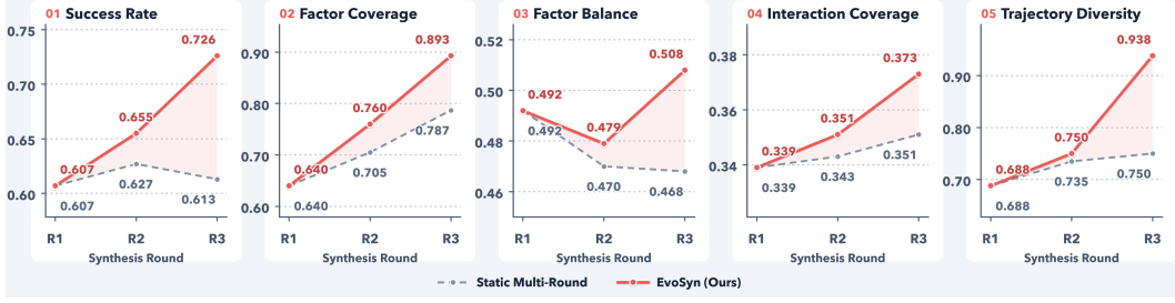
Figure 4: Closed-loop evolution of task performance and synthetic-data quality on CAR-Bench. Unlike static accumulation, EVOSYN progressively improves both downstream success and the structural quality of synthesized experience across successive synthesis rounds.
