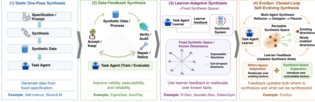
Figure 1: From static synthesis to closed-loop self-evolving agentic synthesis. Existing paradigms improve data quality or adapt within a fixed synthesis space. In contrast, EVOSYN uses learner feedback to revise both the allocation over known factors and the synthesis space itself by introducing new controllable interaction factors.
