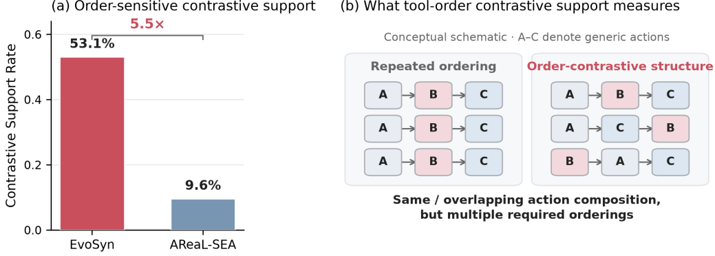
Figure 8: Order-sensitive contrastive structure in synthetic data. Left: On Telecom, EVOSYN exhibits substantially higher tool-order contrastive support than the domain-matched AReal-SEA baseline (53.1% vs. 9.6%, 5.5 \times ). Right: Conceptual illustration of the metric. Repeated use of the same ordering provides little order-level contrast, whereas multiple orderings over the same or overlapping action composition create richer order-sensitive structural variation.
