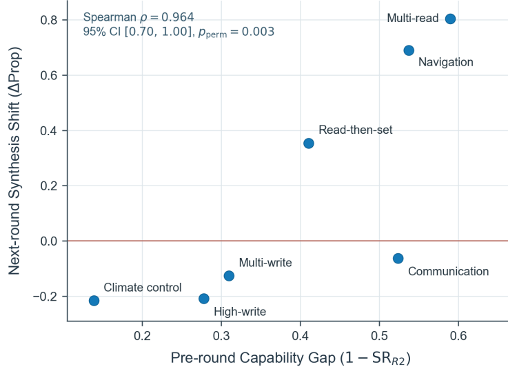
Figure 11: Capability-gap-driven synthesis reallocation on CAR-Bench from R2 to R3. Each point denotes an interaction slice. The pre-round capability gap ( 1 - \text{SR}_{R2} ) is strongly aligned with the subsequent change in synthesis allocation (Spearman \rho = 0.964 , 95% CI [0.70, 1.00] , permutation p = 0.003 ), showing that EVOSYN shifts synthesis effort toward regions where the current learner remains weak.
