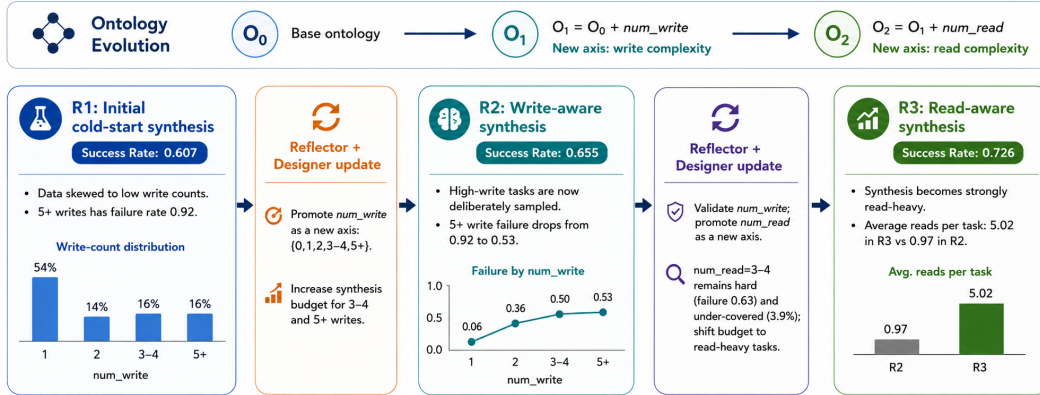
Figure 3: Closed-loop synthesis-space evolution on CAR-Bench. As learner weaknesses shift across rounds, EVOSYN promotes newly discovered interaction factors into explicit generation controls and redirects synthesis toward the evolving capability boundary, progressing from write-intensive execution to increasingly read-intensive decision making.
