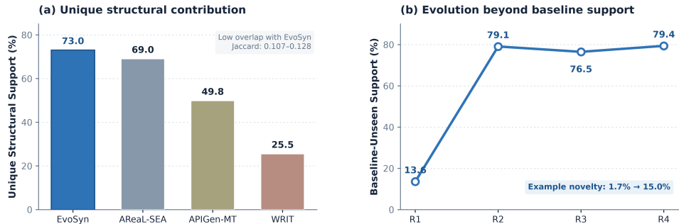
Figure 7: Structural complementarity of EVOSYN relative to domain-matched synthetic-data baselines on Airline. Left: fraction of each method’s distinct decisive interaction support that is absent from the pooled support of all other methods under matched data budgets. EVOSYN provides the largest unique structural contribution. Right: fraction of EVOSYN’s structural support that is absent from the union of all matched baseline corpora across synthesis rounds. Iterative synthesis-space evolution progressively moves generation toward interaction structures not represented by existing synthesis pipelines.
