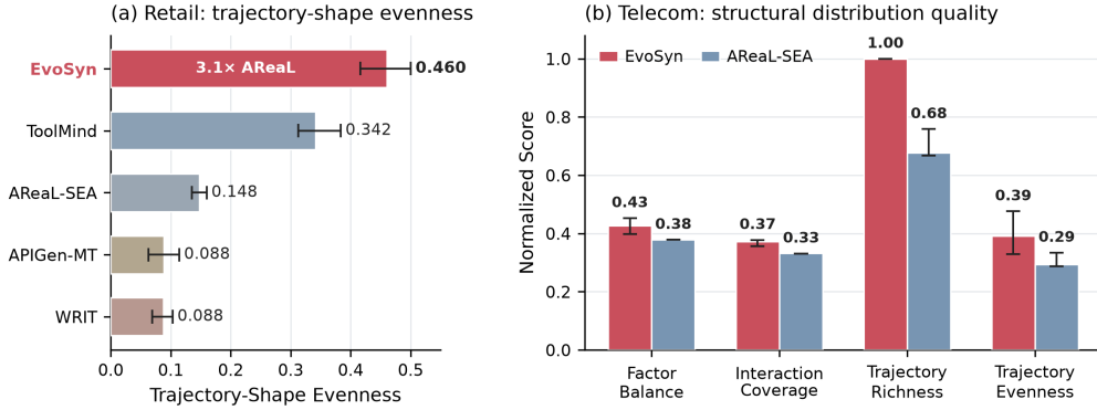
Figure 9: Balanced structural diversity of synthetic agent data. Left: On Retail, EVOSYN achieves the highest trajectory-shape evenness among five domain-matched synthetic corpora under the same data budget, exceeding the strongest competing method by 1.35 \times and AReal-SEA by 3.12 \times . Right: On Telecom, where the compared ground-truth traces have directly comparable decisive-action structure, EVOSYN provides higher factor balance, interaction coverage, trajectory richness, and trajectory evenness than AReal-SEA. Together, these results show that EVOSYN distributes synthesis mass across a broader and more balanced set of interaction structures rather than concentrating on a small number of dominant trajectory patterns.
