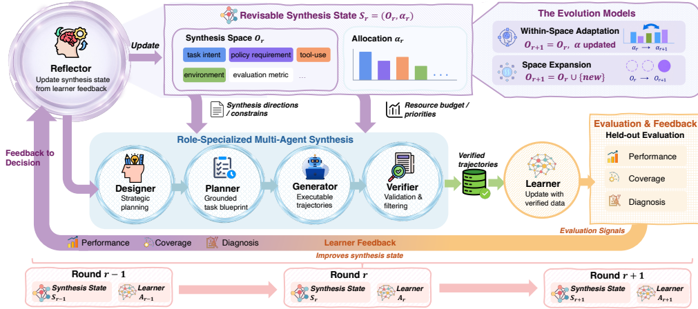
Figure 2: Overview of EVOSYN. Each round instantiates a closed-loop synthesis–learning process in which a revisable synthesis state mediates learner diagnosis and generation control, role-specialized agents realize verified experience, and feedback drives within-space adaptation or synthesis-space expansion to co-evolve synthesis with task-agent learning.
