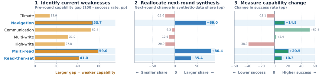
Figure 10: Capability-gap-driven synthesis adaptation on CAR-Bench from R2 to R3. As the learner’s residual weakness shifts toward read-intensive decision making, EVOSYN substantially increases the verified-data share of navigation, multi_read, and read_then_set, all of which subsequently improve after training.
