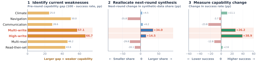
Figure 5: Capability-gap-driven synthesis adaptation on CAR-Bench. The three panels trace the closed-loop transition from pre-round capability gaps to next-round synthesis reallocation and subsequent capability changes, showing how EVOSYN redirects synthesis toward learner weaknesses.
