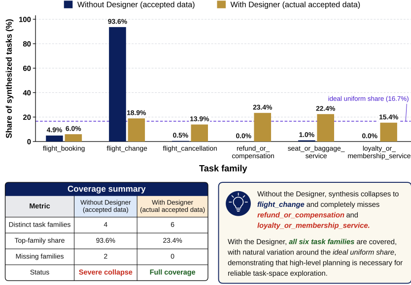
Figure 6: Role of the Designer in task-space exploration on \tau^2 -Bench Airline. A Planner–Generator pipeline without explicit high-level allocation collapses toward flight_change , whereas introducing the Designer separates global synthesis allocation from local task construction and restores coverage across all six task families.
