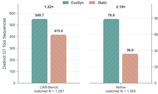
Figure 12: Size-matched structural support at the final synthesis round. The cumulative EVOSYN pool is subsampled to match the number of accepted examples in the Static baseline, and structural support is measured by the number of distinct ground-truth tool-call sequences. After controlling for data volume, EVOSYN still covers 1.32\times more interaction sequences on CAR-Bench and 2.19\times more on Airline.
