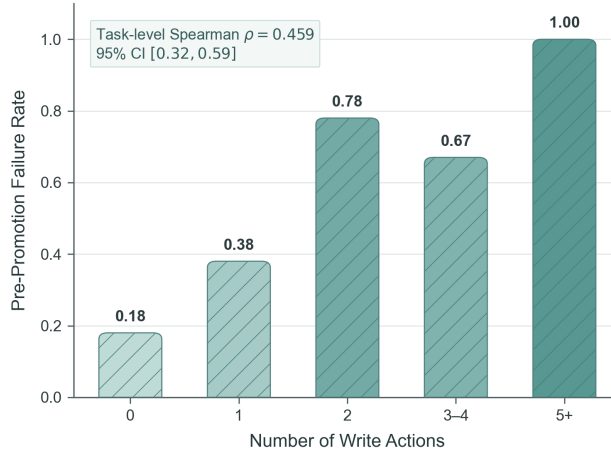
Figure 13: Pre-promotion learner failure rate across num_write buckets on Airline. Tasks requiring more state-changing write actions are substantially more failure-prone before num_write is introduced as an explicit synthesis coordinate, with a positive task-level association between write complexity and learner failure (Spearman \rho = 0.459 , 95% CI [0.32, 0.59]).
