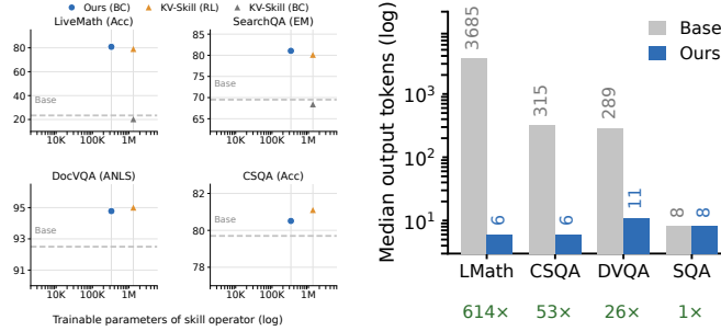
Figure 3: Left: accuracy versus trainable parameters per task. DecSteer (BC) at 0.33M reaches or exceeds every KV-Skill variant at 1.33M, while KV-Skill’s own BC control (same signal, same examples) stays at the base. Right: median generated tokens, base versus DecSteer. LiveMath drops from 3,685 to 6 tokens (36 \times wall-clock), DocVQA from 289 to 11 (10.3 \times ), with accuracy unchanged or higher; SearchQA already answers directly.
