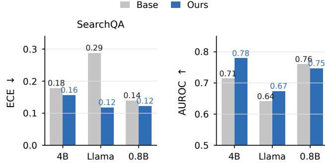
Figure 9: SearchQA calibration before and after skill injection: ECE (left) and answer-ranking AUROC (right) across the three backbones.
