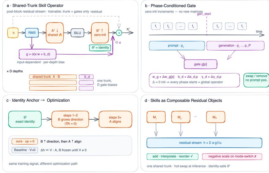
Figure 2: Overview. a : A shared low-rank backbone is injected at D=8 depths with per-depth input-dependent gate g ; the operator is identity at initialization. b : The gate can be phase-conditioned on prompt vs. generation via zero-init increments. c : The identity anchor steers optimization: with up=0 , the output projection gets gradient from step one, while baselines V=0 keeps both large matrices frozen until V moves. d : Trained skills act as composable residual objects.
