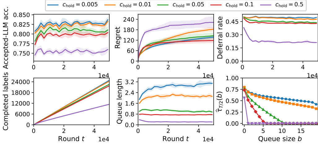
Figure 10: Effect of the holding cost on KL-PBD. We vary c_{\text{hold}} \in \{0.005, 0.01, 0.05, 0.1, 0.5\} with T = 50,000 , \mu = 0.5 , B = 20 , c_e = 2 , and c_{\text{exp}} = 0.25 . From the upper-left to the lower-right, the panels show accepted-LLM accuracy, cumulative regret, empirical deferral rate, cumulative completed expert labels, average queue size, and the deferral threshold \hat{\tau}_{T/2}(b) at t = T/2 as a function of queue size b .
