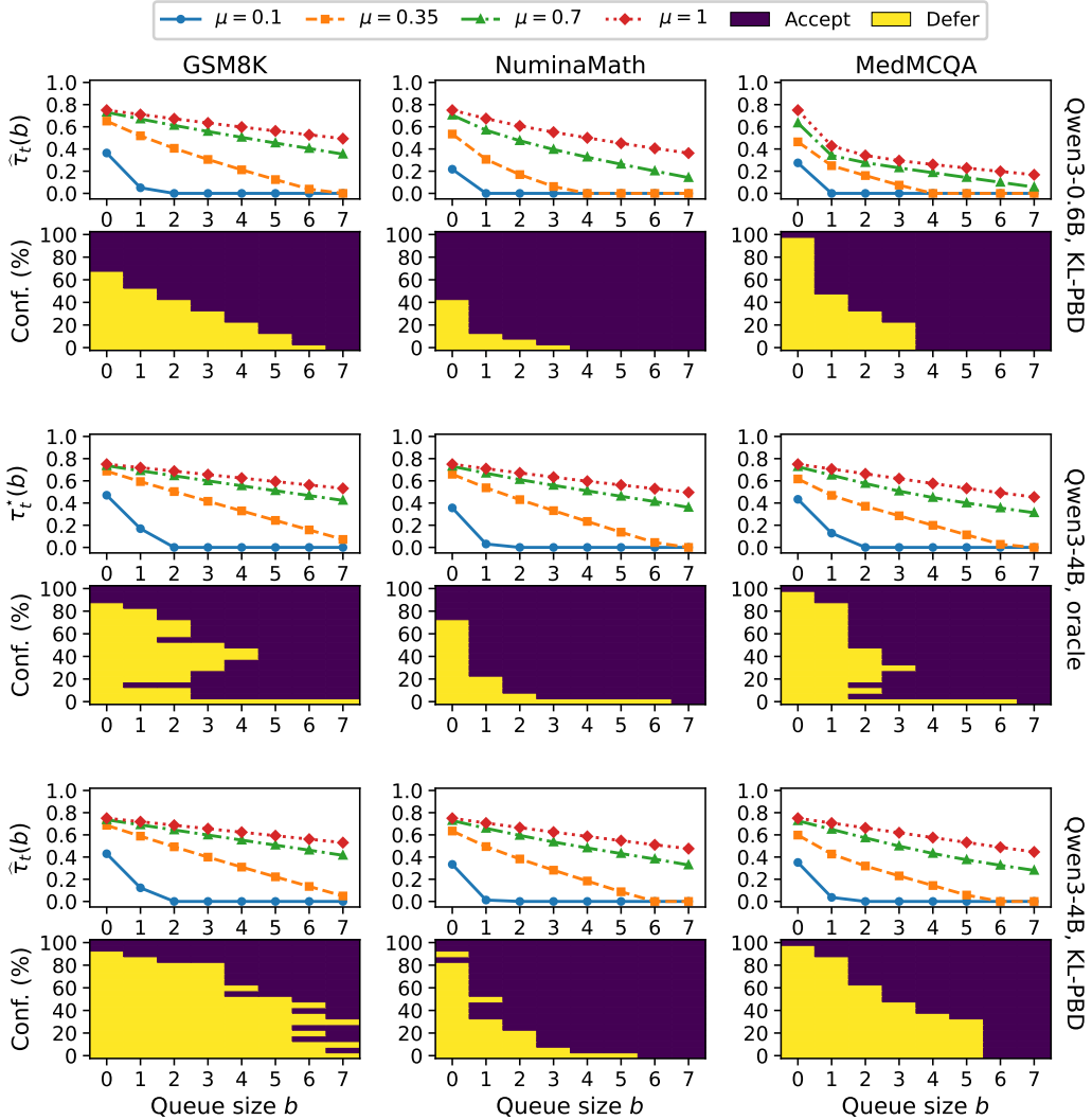
Figure 15: Thresholds for varying \mu and decisions for \mu = 0.35 at t = T/2 : KL-PBD for Qwen3-0.6B (top), oracle (middle) and KL-PBD (bottom) for Qwen3-4B, one run per \mu .
