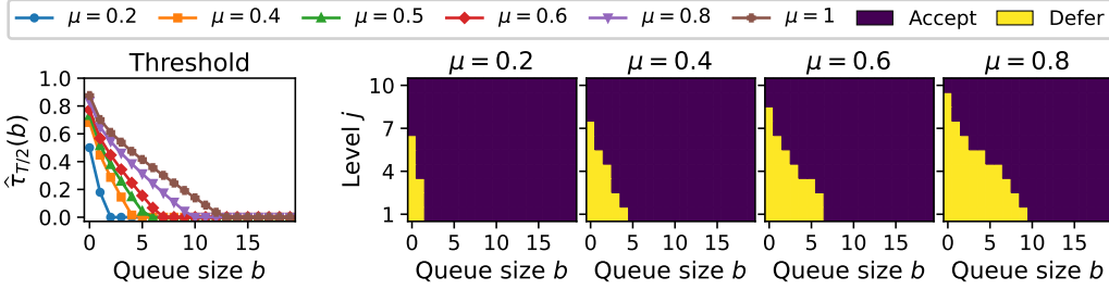
Figure 8: KL-PBD threshold \hat{\tau}_{T/2}(b) as a function of queue size b , averaged over the runs (left), and learned KL-PBD decisions, most frequent over the runs (right), at t = T/2 for different service rates \mu .
