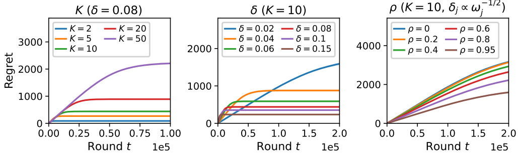
Figure 7: Regret of KL-PBD on the two-point instance for different K with \delta = 0.08 (left, shown up to t = 10^5 ) and different \delta with K = 10 (center), and for different arrival distributions with K = 10 and h_j^* = 0.5 + \sqrt{\phi(T)/(2\omega_j T)} (right). 95% confidence intervals over 100 runs are displayed as bands but are too small to be visible.
