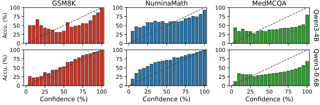
Figure 2: Conditional accuracy of the self-consistency score (dashed line: perfect calibration).
