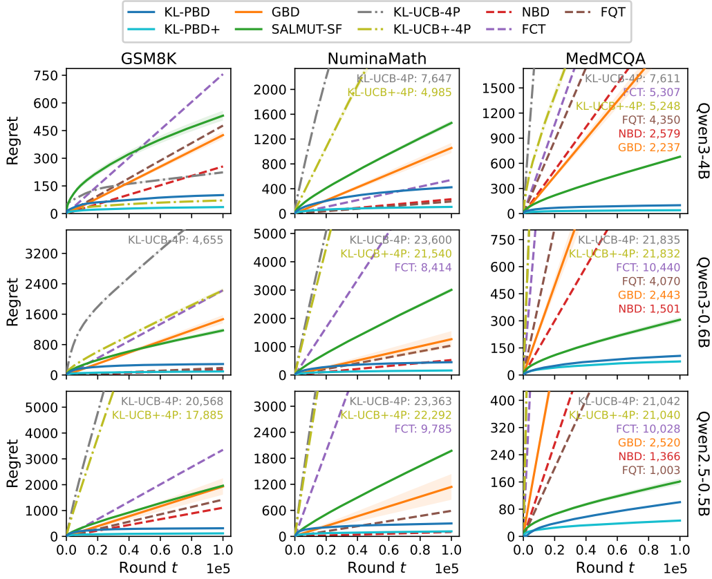
Figure 12: Regret of all algorithms, T = 10^5 , 100 runs. Truncated curves are listed with their final regret.
