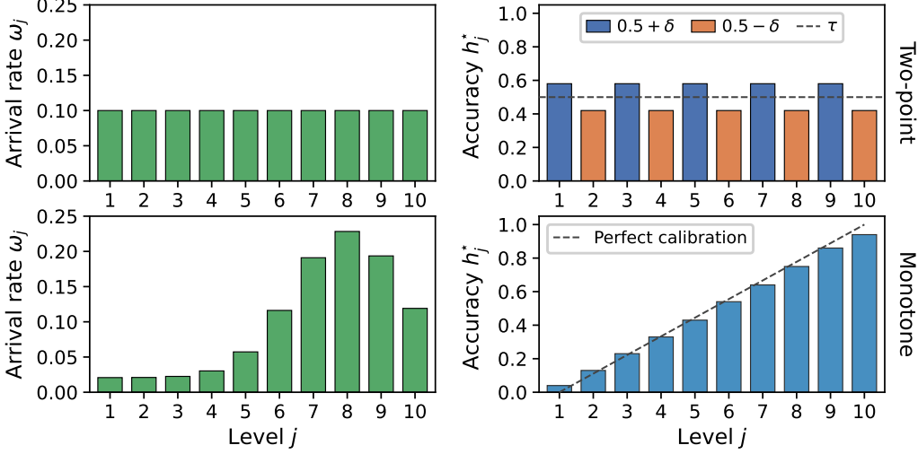
Figure 5: Top: two-point instance with \delta = 0.08 . Bottom: monotone instance (dashed line: perfect calibration, i.e., h_j^* = p_j with p_j = (j - 1)/9 ).
