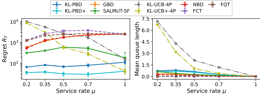
Figure 14: Service-rate sweep, T = 5 \cdot 10^4 , 24 runs: final regret (left) and mean queue length (right).
