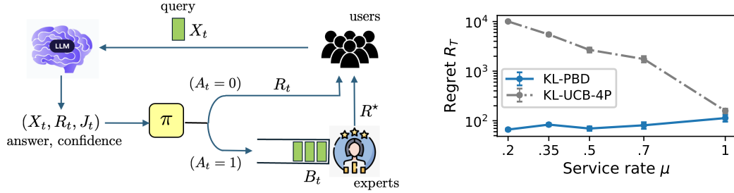
Figure 1: Left: expert-aided LLM system with deferral policy \pi and delayed feedback from completed expert reviews. Right: regret after T = 5 \times 10^4 queries on MedMCQA with Qwen3-4B against the expert service rate \mu , comparing the queue-aware KL-PBD with the queue-unaware KL-UCB-4P. For \mu = 1 , deferred queries are served before the next round and the queue does not build up, so queue awareness provides no benefit. For \mu < 1 , deferred queries accumulate and create congestion, making queue-aware deferral essential for low regret. Details in Appendix H.3.
