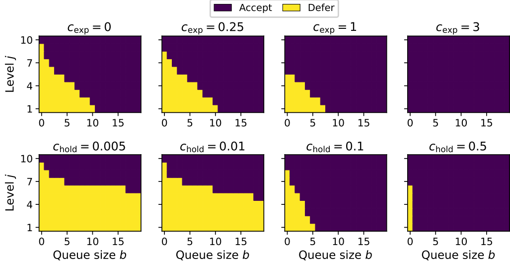
Figure 11: Learned KL-PBD decisions for varying c_{\text{exp}} and c_{\text{hold}} , for t = T/2 (most frequent decision over the runs).
