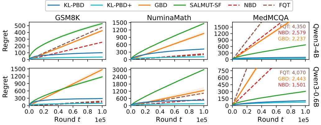
Figure 3: Regret averaged over 100 runs. Curves leaving the frame are listed with their final regret.
