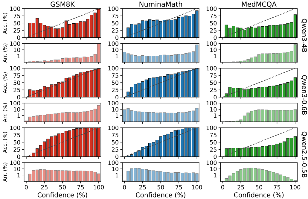
Figure 6: Conditional accuracy (top) and arrival rates (bottom) of the self-consistency score. The dashed line represents a perfectly calibrated score.
