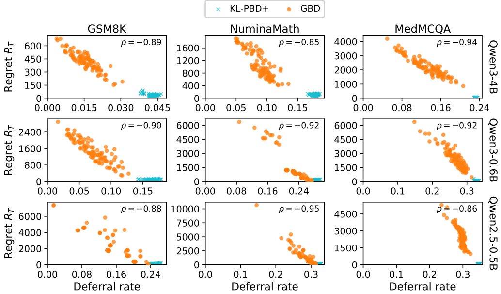
Figure 16: Final regret against average deferral rate, one point per run, T = 10^5 , and \rho the correlation for GBD.
