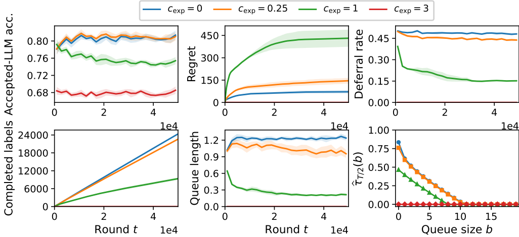
Figure 9: Effect of the expert-review cost on finite-horizon KL-PBD. We vary c_{\text{exp}} \in \{0, 0.25, 1, 3\} , with T = 50,000 , \mu = 0.5 , \bar{B} = 20 , c_e = 2 , and c_{\text{hold}} = 0.05 . From the upper-left to the lower-right, the panels show accepted-LLM accuracy, cumulative regret, empirical deferral rate, cumulative completed expert labels, average queue size, and the deferral threshold \hat{\tau}_{T/2}(b) at t = T/2 as a function of queue size b .
