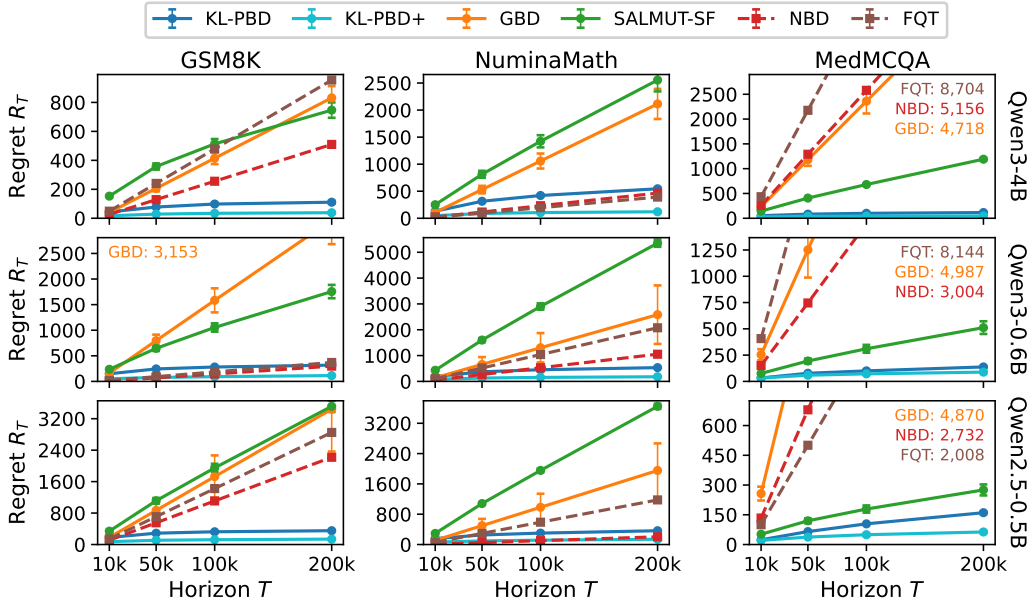
Figure 13: Final regret versus horizon T , 24 runs per point. Truncated curves are listed with their final regret.
