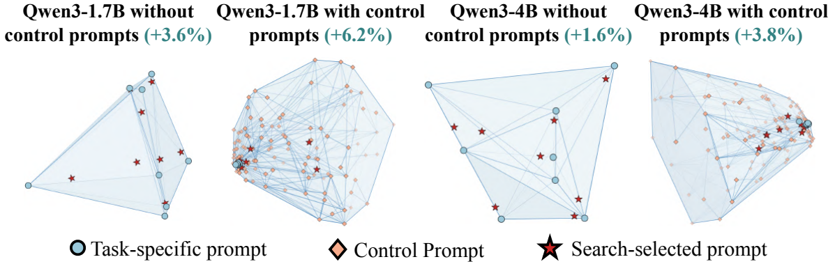
Figure 5 Visualization of the learned anchored prompt space with and without non-vertex control prompts on Qwen3-1.7B and Qwen3-4B. The values in green indicate the cumulative performance improvement over the eight tasks after space search.
