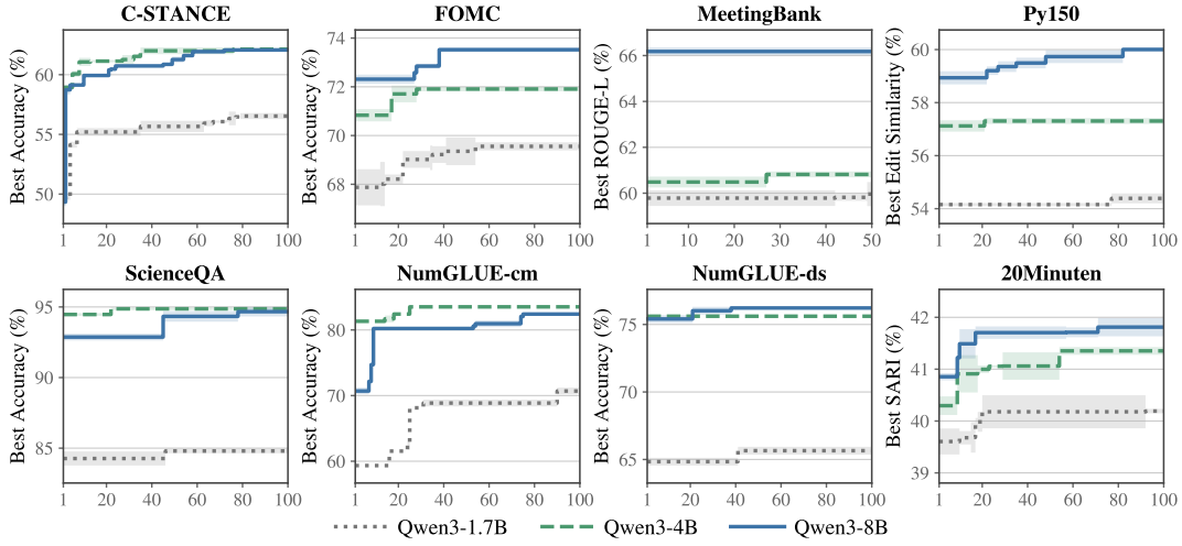
Figure 6 Bayesian optimization convergence across eight TRACE tasks and three Qwen3 model scales. Curves report the best validation performance observed so far over successive evaluations.
