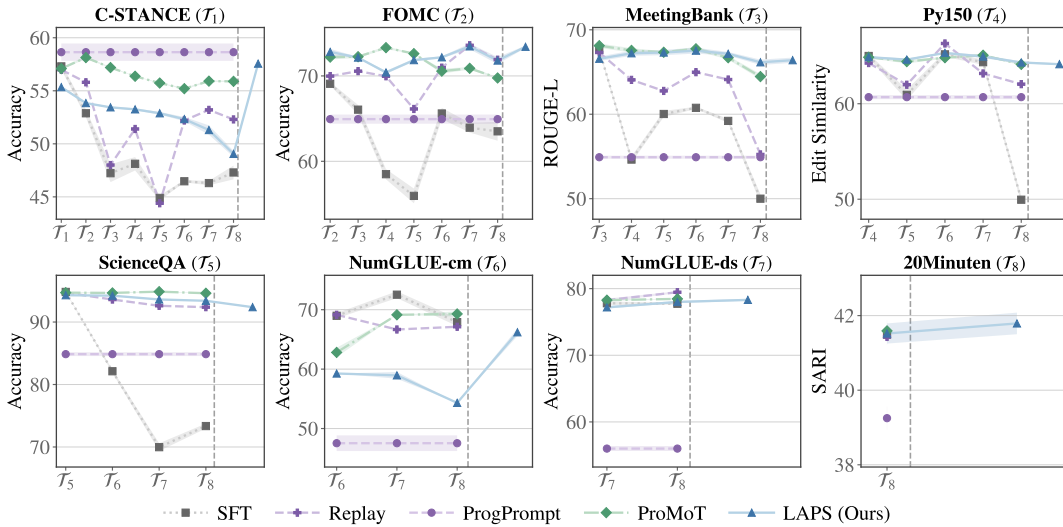
Figure 8 Task-wise continual adaptation trajectories on TRACE with Qwen3-8B.
