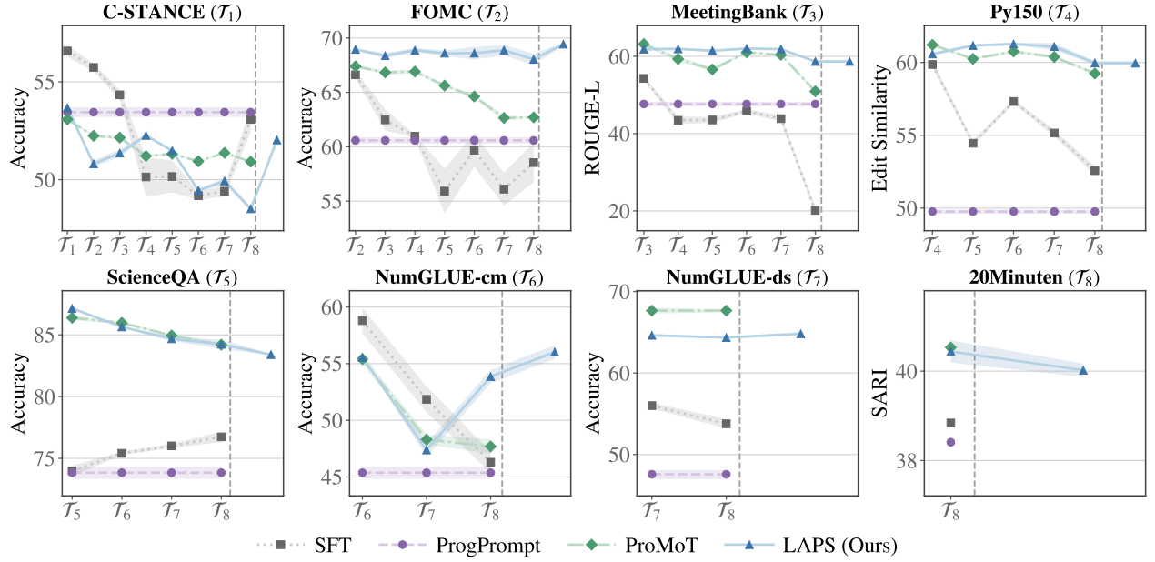
Figure 2 Task-wise continual adaptation trajectories with Qwen3-1.7B. Each panel tracks one task after it is learned, and later points show its performance after subsequent adaptation stages. Drops indicate forgetting as the model learns new tasks. The gray dashed line marks the transition from sequential adaptation to the validation-guided prompt selection introduced in LAPS.
