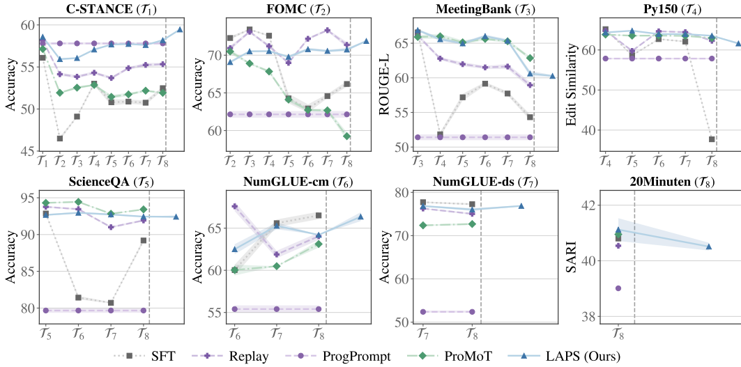
Figure 7 Task-wise continual adaptation trajectories on TRACE with Qwen3-4B.
