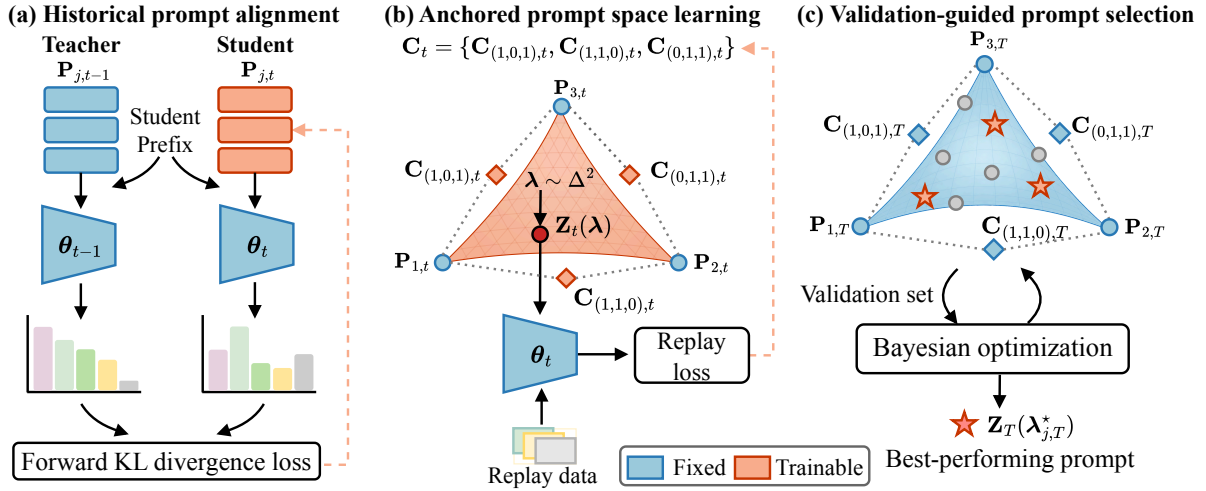
Figure 1 Overview of LAPS. (a) After adapting to the current task \mathcal{T}_t , LAPS aligns each historical prompt \mathbf{P}_{j,t-1} to the updated model, producing \mathbf{P}_{j,t} through on-policy self-distillation. (b) The aligned prompts \{\mathbf{P}_{j,t}\}_{j \leq t} are fixed as simplex anchors, while non-vertex Bézier control prompts \mathbf{C}_{\alpha,t} are trained with cross-task replay losses to shape the space between anchors. (c) With the final model fixed, Bayesian optimization searches validation scores over simplex coordinates \lambda and returns the selected soft prompt \mathbf{Z}_T(\lambda_{j,T}^*) for each observed task.
