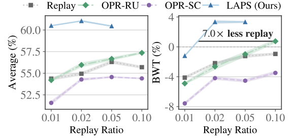
Figure 4 Average performance and BWT across replay ratios on Qwen3-1.7B.
