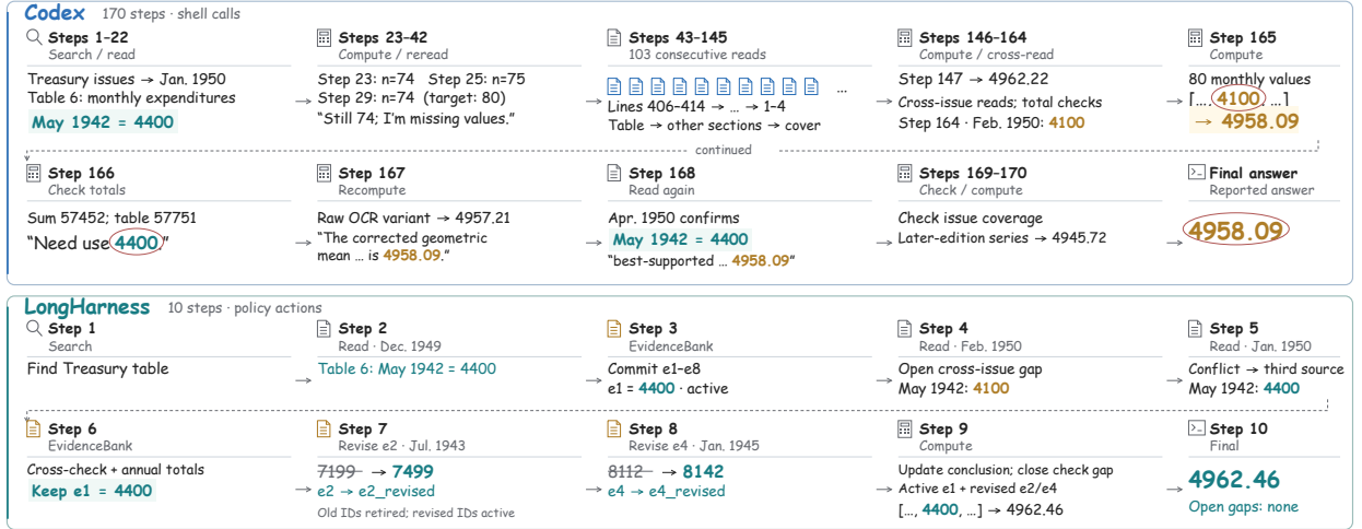
Figure 4 Evidence lifecycle comparison with GLM-5.3-Flash on OfficeQA Pro V1. For the geometric mean of 80 monthly Treasury expenditures, Codex continues searching and omits a recognized correction; LONGHARNES updates its evidence and returns the reference answer, 4962.46 million dollars. Circles mark Codex’s incorrect input, correction, and final answer.
