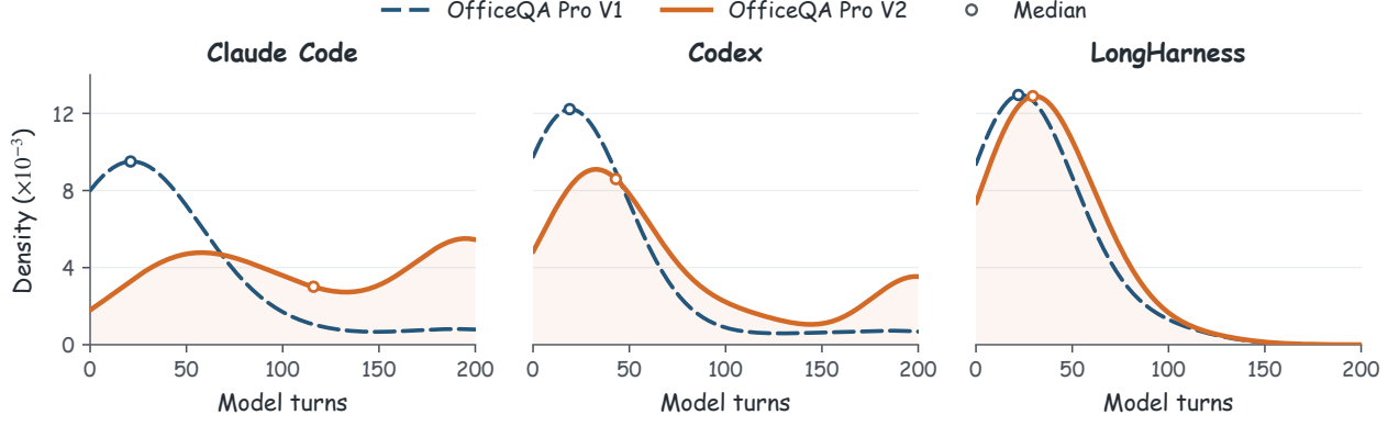
Figure 3 Distributions of model turns per question on OfficeQA Pro V1 and V2 with GLM-5.3-Flash. Each panel compares the two versions for one harness. Curves show kernel density estimates, and circles indicate medians.
