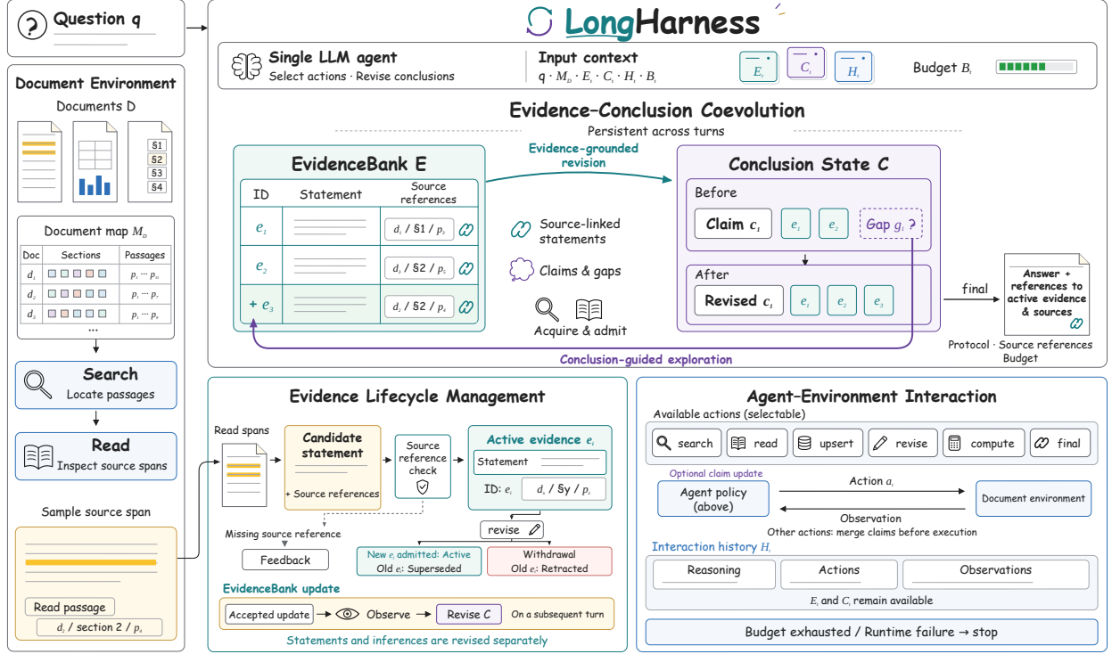
Figure 2 Overview of LONGHARNESS. A single agent maintains an EVIDENCEBANK and a CONCLUSION STATE while interacting with external documents. Evidence–Conclusion Coevolution uses unresolved conclusions to guide exploration and accepted evidence to revise those conclusions, while Evidence Lifecycle Management governs which statements remain active and preserves their source references throughout the interaction.
