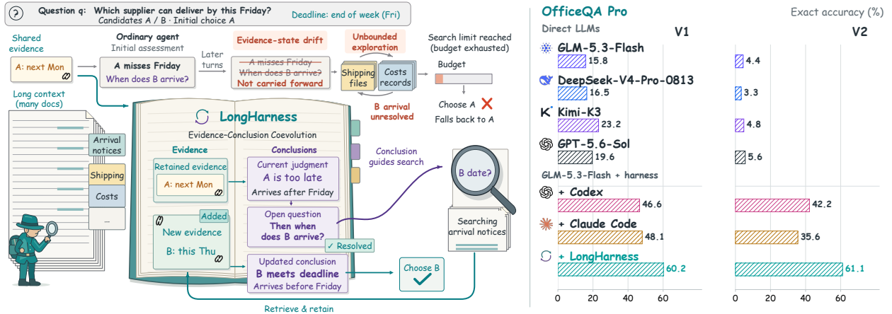
Figure 1 Evidence lifecycle management for corpus-level long-context reasoning. The left panel illustrates how an agent loses an earlier constraint and continues searching, while LONGHARNESS retains the evidence, uses an unresolved conclusion to guide retrieval, and revises its decision when new evidence arrives. The right panel compares exact accuracy (%) on OfficeQA Pro V1 and V2 for direct models and agent harnesses using GLM-5.3-Flash.
