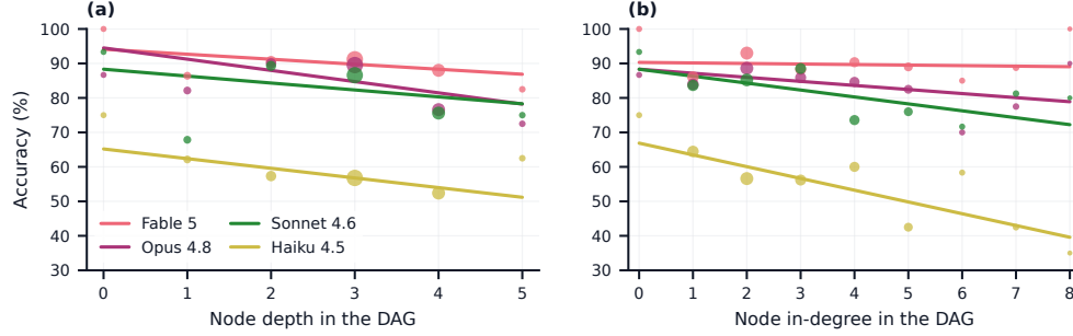
Figure 4: Accuracy by position in the dependency DAG. Accuracy a_r of requests 8–10 as a function of (a) the request’s depth in the DAG and (b) its in-degree. Markers show the mean accuracy per value (area \propto number of requests); lines are least-squares fits over all requests.
