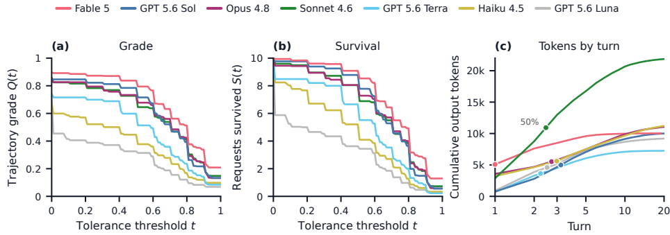
Figure 3: Performance across tolerance levels and output length. (a, b) Tolerance sweeps for the closed-source models (open-source models in App. G): delivered functionality Q(t) and request survival S(t) as a function of tolerance t ; the area under each curve gives the Grade and Survival in Table 2. Curves show the run mean across three runs. (c) Cumulative output tokens per request by agent turn; dots mark where each model reaches half of its total.
