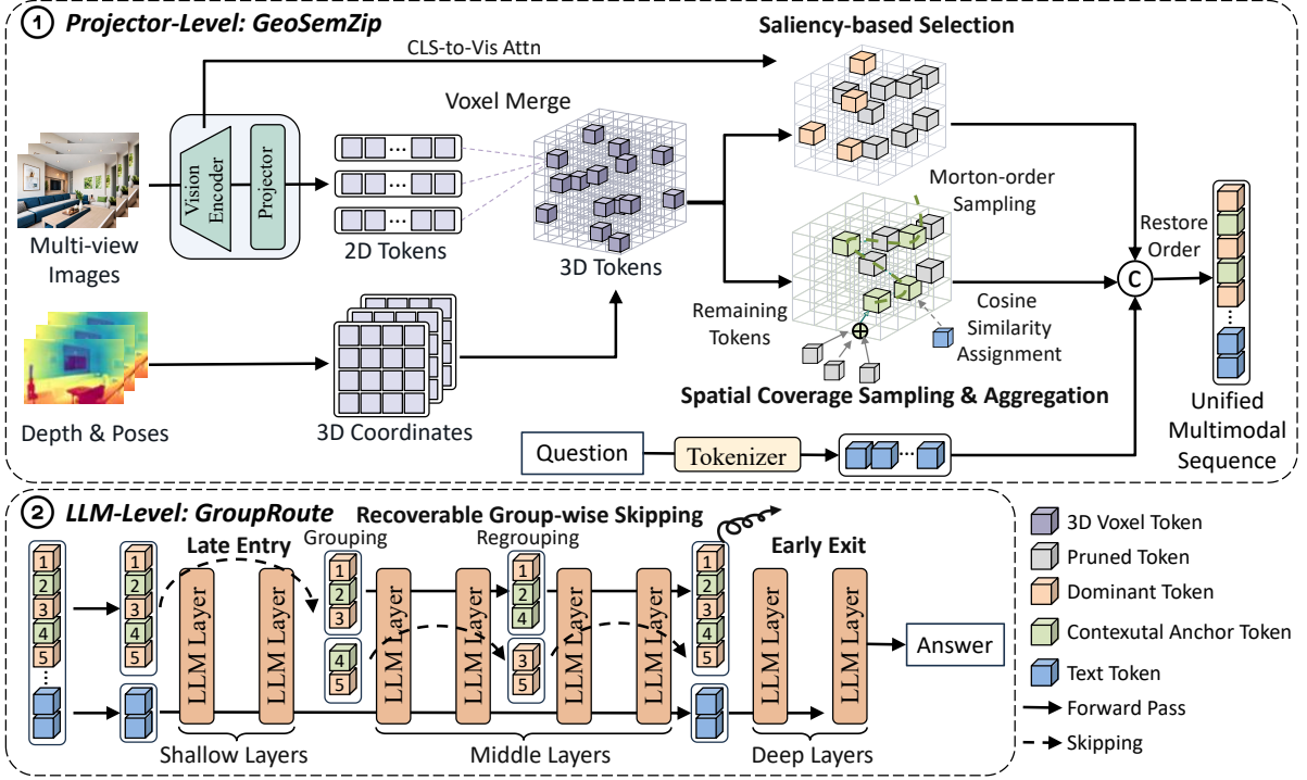
Figure 3: Overview of GeoGR. (1) Projector-level Compression: GeoSemZip consolidates cross-view observations into 3D voxel tokens using depth and camera poses. Saliency-based selection preserves dominant tokens, while Morton-order sampling selects contextual anchors that aggregate unselected voxel features by cosine similarity. The compressed visual tokens are combined with text tokens to form the LLM input. (2) LLM-level Compression: GroupRoute confines visual computation to an intermediate-layer window through Late Entry and Early Exit. Within this window, Recoverable Group-wise Skipping routes query-conditioned token groups through or around complete LLM layers. Skipped tokens retain their hidden states and can resume computation after regrouping at subsequent anchor layers. Text tokens remain active throughout the LLM.
