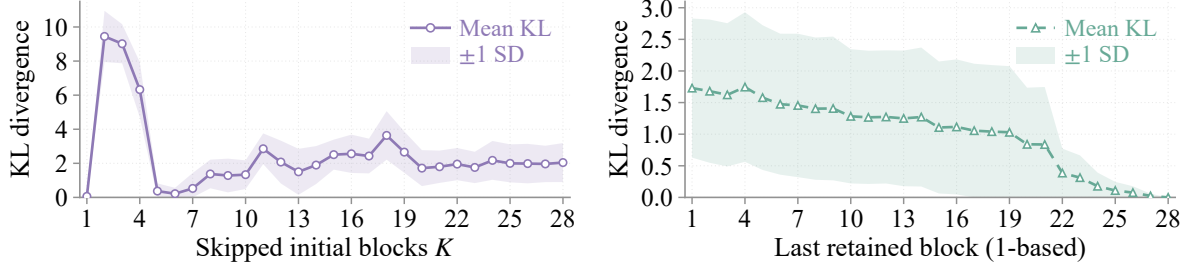
Figure 4: Visual-window diagnosis for LLaVA-OneVision on 256 ScanQA examples: Late Entry (left) and Early Exit (right). Lines show mean next-token KL divergence relative to full visual computation; shading indicates \pm 1 standard deviation, with the lower bound clipped at zero.
