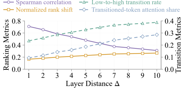
Figure 2: Cross-layer stability of visual token rankings. Ranking stability decreases with layer distance, while initially low-ranked tokens increasingly enter the top half and account for a growing share of its attention.
