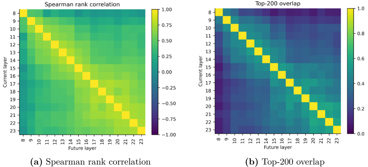
Figure 5: Layer-pair stability of visual-token relevance on ScanQA. For LLaVA-OneVision decoder layers 8–23, (a) gives Spearman correlation between complete visual-token rankings, and (b) gives the fraction shared by the two layers’ top-200 sets.
