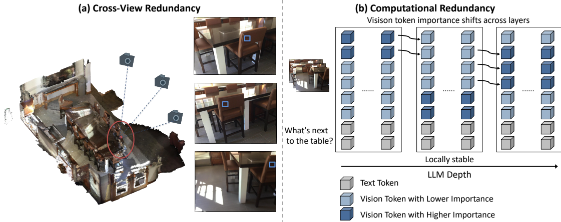
Figure 1: Redundancy in multi-view 3D VLMs. (a) Overlapping views repeatedly observe the same 3D region (blue boxes). (b) For the same question, visual token importance remains locally stable but shifts across more distant layers. See Section 3 for quantitative analysis.
