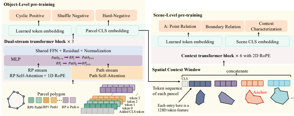
Figure 7: Vector encoder architecture and geometry pretraining. The object encoder processes alternating reference-point and path elements with separate attention streams and endpoint-conditioned cross-stream interaction. The resulting element sequences are then concatenated into a spatial context window and processed by the scene encoder with 2D positional encoding.
