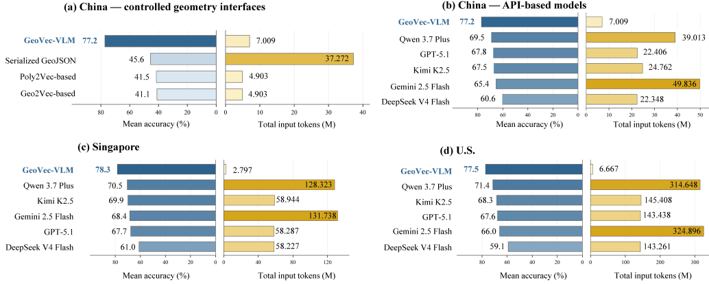
Figure 13: Total input-token consumption and spatial reasoning accuracy across evaluation sets. Token counts include the complete model input, including visual inputs, language instructions, and geometry when present. For API models, counts are those reported by the corresponding model interface. China and U.S. each contain 10,800 evaluated questions, while Singapore contains 3,600. Geo2Vec and Poly2Vec are evaluated only in the controlled China setting, consistent with Table 2.
