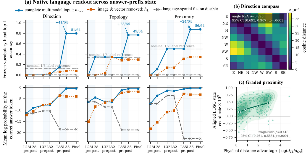
Figure 12: Spatial information enters and structures the language path. (a) Vocabulary-head readout of the answer-prefix state around language-spatial fusion. With multimodal inputs, top-1 accuracy rises sharply after the language states read the spatial memory; removing this fusion suppresses the transition. (b) Pairwise distances between direction-conditioned language states increase with physical angular separation. (c) Proximity-state variation tracks the physical distance advantage between candidates.
