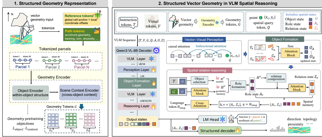
Figure 2: Architecture of GeoVec-VLM. The geometry encoder preserves within-object structure and scene-level metric structure in geometry tokens. Inside the VLM, geometry tokens interact with visual and spatial-query tokens, are organized into object states, and form query-conditioned role and relation states used by the language generation path. Structured decoders provide spatial supervision during training.
