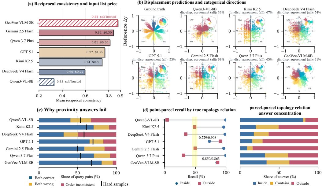
Figure 3: Task accuracy can conceal geometrically inconsistent spatial behavior. (a) Mean reciprocal consistency over direction, comparative proximity, and topology. Because repeated errors can remain reciprocally consistent, panels (b–d) examine task-specific geometric constraints. (b) Categorical direction predictions are compared with the directions implied by predicted horizontal and vertical displacements. Polar histograms show the corresponding answer distributions. (c) Proximity is evaluated under candidate-order reversal, which preserves the physically closer parcel. Black ticks indicate hard-sample accuracy. (d) Point–parcel class-conditional recall and parcel–parcel prediction frequencies reveal query-dependent topology bias.
