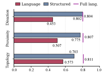
Figure 5: Language and structured readouts without O/A/Z, attached directly to G .
