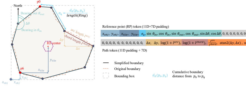
Figure 6: Reference-point and path feature construction. Left: boundary simplification and the geometric features extracted for reference-point and path elements. Right: the features are packed into a shared 18-dimensional feature representation, where reference-point and path features occupy complementary channels and inactive channels are zero-padded. The complete feature definitions are summarized in Table 4.
