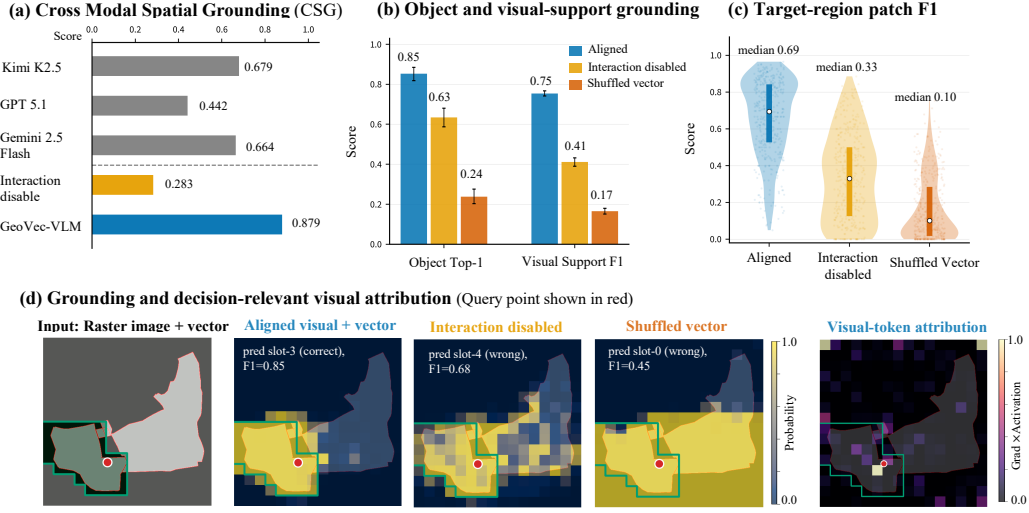
Figure 4: Vector-visual alignment supports cross-modal grounding. (a) CSG requires mapping image-only query points to their corresponding vector parcels. (b–c) Grounding signals weaken when vector-visual interaction is disabled, and further deteriorate after shuffling vector geometry. (d) With aligned inputs, visual support and decision-relevant attribution focus on the corresponding parcel. The final panel shows positive Gradient \times Activation for the gold grounding margin.
