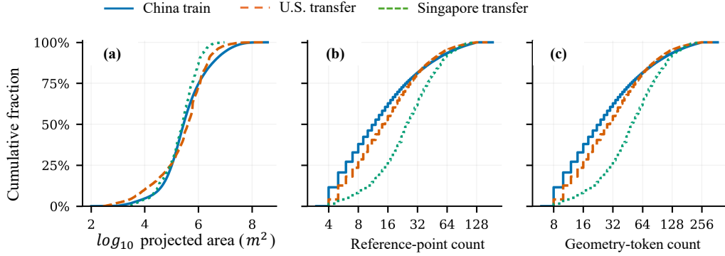
Figure 9: Geometry distribution shifts between training and transfer geographies. Empirical cumulative distributions of (a) projected polygon area, (b) retained reference-point count, and (c) geometry-token sequence length for L4 polygons in the China training regions and the U.S. and Singapore transfer geographies. Transfer distributions are computed over the polygons in the reported evaluation regions.
