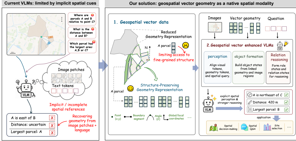
Figure 1: Motivation and overview of GeoVec-VLM. Current VLMs infer spatial relations from raster images and language, where metric geometry and spatial relations are only implicitly represented. GeoVec-VLM introduces geospatial vector data as a native spatial modality, preserves its geometric structure during representation, and integrates it with visual and language information for spatial perception and reasoning.
