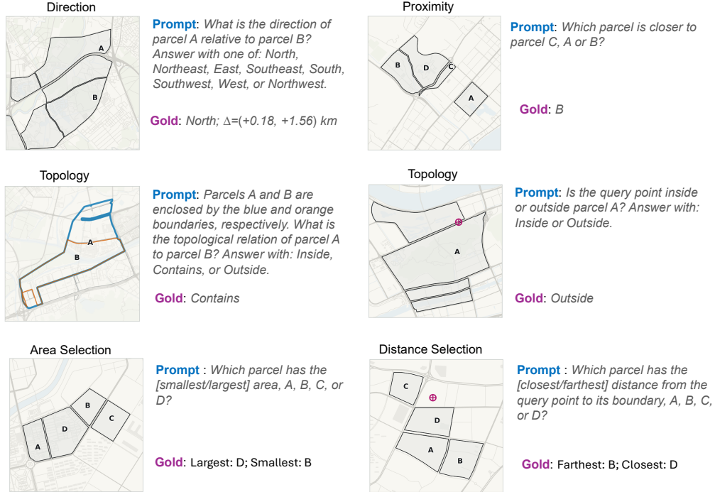
Figure 10: Representative examples from the benchmark. Each panel shows the visual input, one prompt realization, and the target answer.
