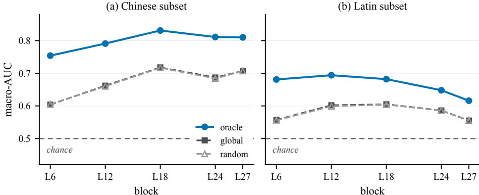
Figure 5: Glyph identity is more accessible at the correct locations. Glyph-identity macro-AUC on SQUINTCTRL-GLYPH by encoder block under the three poolings of §3.2. RANDOM uses the same number of tokens as ORACLE but remains close to GLOBAL across depth and script.
