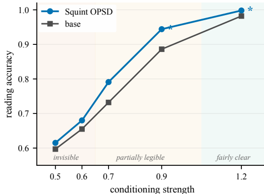
Figure 7: Recoverability versus hiding strength. Reading accuracy for the base model and SQUINT OPSD as conditioning strength varies, over the same 200 scenes. Stars mark strength levels at which the 95% CI of the paired base-vs-SQUINT OPSD difference excludes zero (paired bootstrap, 100 resamples); unmarked levels are not significant at this threshold, and 0.7 is borderline and is left unmarked. The method provides its clearest benefit in the partially recoverable regime; the two ends saturate for different reasons.
