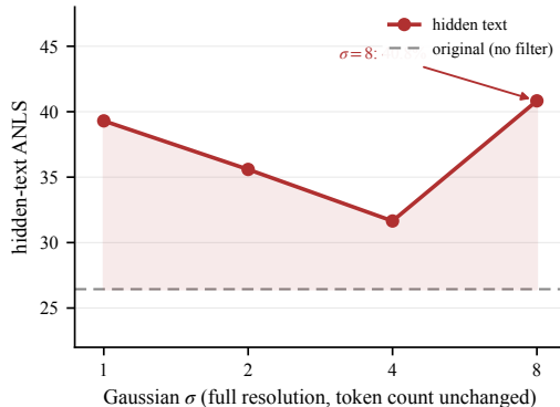
Figure 6: Frequency at constant token count. Hidden-text reading ANLS on all 1076 SQUINT-BENCH images under Gaussian low-pass filtering. The dashed line is the unfiltered input; the visual-token count is unchanged throughout the sweep.
