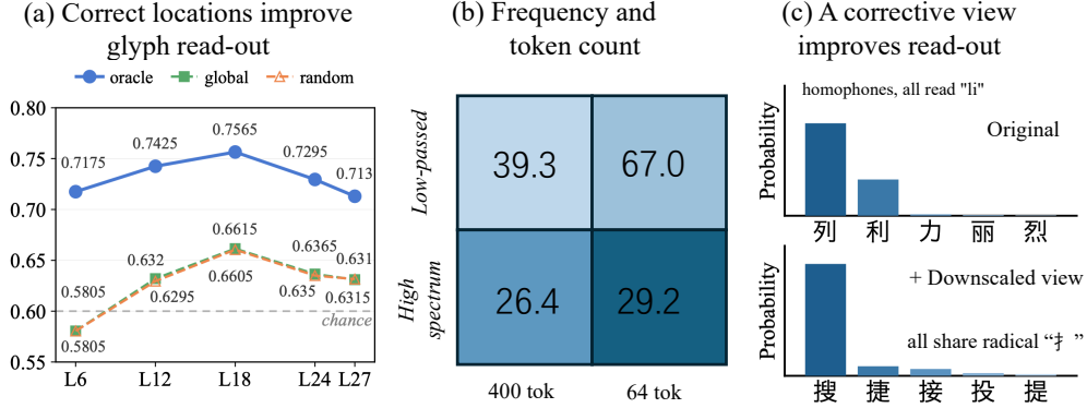
Figure 2: Three diagnostics on frozen off-the-shelf weights. (a) Restricting the read-out to glyph-bearing tokens improves glyph-identity prediction, supporting spatial selection as a major bottleneck (per-layer expansion in Appendix A). (b) At a fixed 64-token budget, suppressing high-frequency content raises squint-text ANLS from 29.2 to 67.0 (per- \sigma results in Appendix B). (c) For the same target glyph 搜, adding a 1/8-scale view of the same image shifts the base model’s phonetic predictions toward visually matching glyphs, indicating stronger visual grounding.
