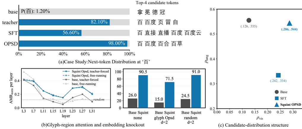
Figure 4: What changes after training. (a) Example next-token distributions for BASE, SFT, and SQUINT OPSD. (b) Attention concentration on glyph-bearing regions and a causal visual-token embedding knockout. (c) Candidate-distribution structure on 120 matched glyph positions.
