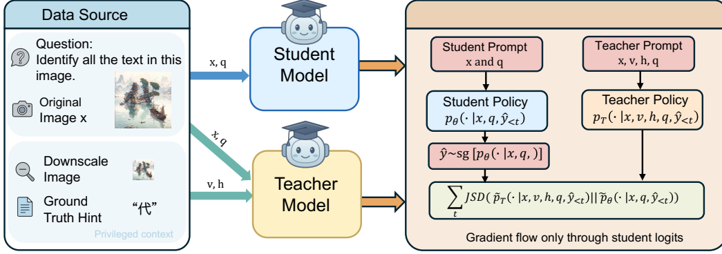
Figure 3: Overview of SQUINT OPSD. The teacher receives the original image, the downsampled view v = g(x) , the task instruction, and the ground-truth output as privileged context. Its token distributions supervise the student along stop-gradient, student-generated trajectories. Gradients flow only through the student logits, and inference uses the original image alone.
