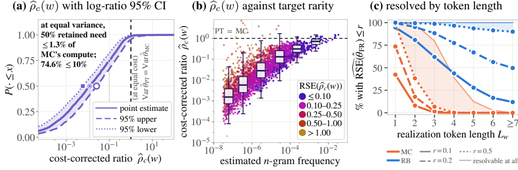
Figure 2: Cost-adjusted variance ratio \hat{\rho}_c(w) for n -gram frequency estimation. (a) Empirical cumulative distribution over 3,700 targets with bootstrap RSE at most 2, with approximate 95% log-ratio confidence bounds. (b) Variance reduction versus estimated frequency for the 2,831 targets with at least 25 expected occurrences in the independent frequency bank. (c) Fraction of targets whose frequency estimate reaches each RSE threshold, grouped by token length, at the same sample size M = 4,000 for both estimators. Dashed parity lines in (a–b) mark equal variance at equal cost under the proxy; in (c), line styles distinguish RSE thresholds.
