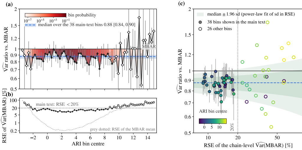
Figure 12: Variance reduction across ARI bins. (a) variance of the cross-fitted estimator relative to MBAR for all 64 populated bins. Filled markers denote the 38 bins for which the MBAR variance is estimated with RSE below 20%; over these bins, the median variance ratio is 0.88 with a 95% bootstrap interval of [0.84, 0.90], and over all 64 populated bins it is 0.88 with interval [0.86, 0.91]. Ratios in the remaining tail bins are much noisier because the MBAR variance itself is poorly estimated. Whiskers show \pm 1.96 bootstrap standard deviations from 1,000 paired chain-bootstrap replicates. (b) RSE of the MBAR variance and mean estimates across bins, showing that uncertainty in the variance estimate grows sharply in the tails. (c) Variance ratios against the RSE of the MBAR variance estimate. Among the 38 reliable bins, the ratio shows no systematic dependence on baseline uncertainty (Spearman \rho = 0.05 , p = 0.78 ), indicating that the observed reduction is not driven by noise in the MBAR variance estimate.
