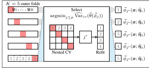
Figure 9: Nested cross-fitting, our in-sample selection among p candidate potentials (Alg. 1). Each of K = 5 outer folds is held out in turn (red); on the remaining folds the candidates are compared by inner cross-validation, the winner j^* is refitted on all remaining data and applied to the held-out fold.
