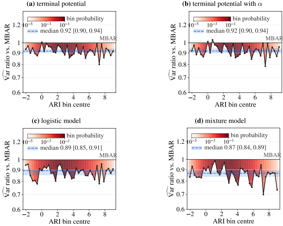
Figure 11: The same view as Fig. 10 for each single candidate, each refitted without the held-out fold and applied to every bin: chain-level variance relative to MBAR per ARI bin over the same 39 bins (38 by the 20% rule plus bin 57), with the bin probability as shading and the candidate's own median over these bins with its 95% interval. The terminal potential and its calibrated version remove 8%, the logistic model 11%, and the mixture model 13%, against 12% for the selection, which picks the mixture model in four folds and the logistic model in one.
