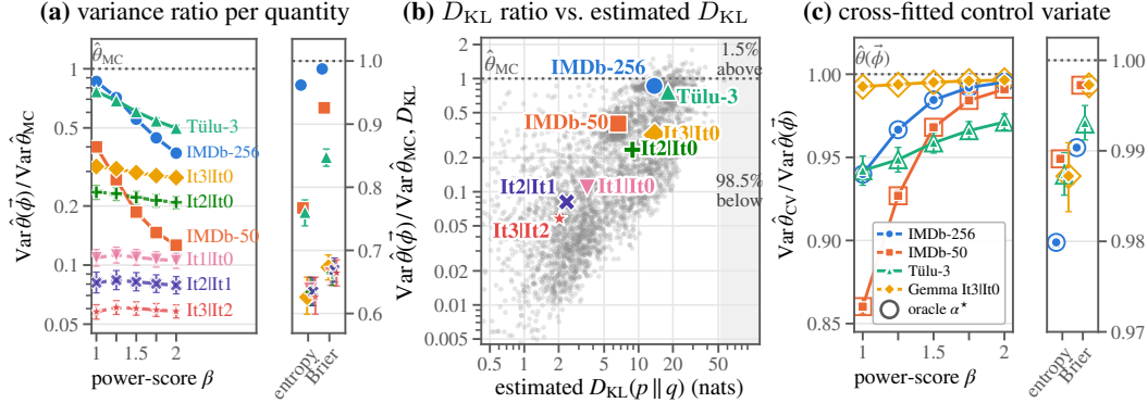
Figure 1: Variance reduction in the proper-loss experiment (lower is better). (a) Variance ratio of the potential estimator to Monte Carlo across power scores ( \beta \rightarrow 1 gives D_{KL} ); entropy and Brier are shown on the right. Each series is one policy–reference pair (see Tab. 10): solid lines are the four main policy–reference pairs and dashed lines are consecutive Gemma-2 SPPO pairs. (b) For D_{KL} , variance ratio against the estimated D_{KL}(p||q) , with one colored marker per pair and grey markers for individual prompts from all pairs. The shaded regions indicate prompts below and above the Monte Carlo variance. (c) Variance ratio of the cross-fitted control-variate estimator to the potential estimator; hollow markers use the full-sample oracle coefficient.
