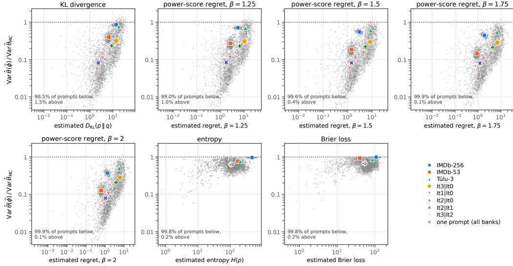
Figure 4: Variance reduction as a function of quantity magnitude for all losses and divergences in the proper-loss experiment. Each panel shows the variance ratio \text{Var}_p(\hat{\theta}(\vec{\phi}))/\text{Var}_p(\hat{\theta}_{\text{MC}}) against the estimated magnitude of the quantity, with one colored marker per policy–reference bank and grey points for individual prompts. For KL and the power-score regrets, variance reduction becomes stronger as the policy–reference divergence decreases, with this dependence becoming more pronounced for larger \beta . Entropy and Brier loss instead remain comparatively close to the Monte Carlo baseline across banks.
