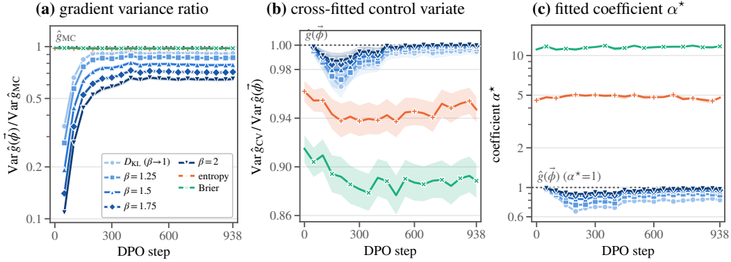
Figure 5: Gradient estimation along a DPO trajectory of the GPT-2 sentiment policy (checkpoints every 50 steps; the variance of an estimator \hat{\theta} is \text{tr Var}_p(\hat{\theta}) over the 512 \times 20 responses). (a) Variance of \hat{\theta}(\vec{\phi}_{\nabla}) relative to the centered Monte Carlo gradient \hat{\theta}_{\text{MC}} , one series per quantity (regrets darker for larger \beta ; undefined at step 0). (b) Variance of the cross-fitted control-variate estimator \hat{\theta}(\vec{\phi}_{\nabla}, \alpha^*) relative to \hat{\theta}(\vec{\phi}_{\nabla}) . (c) The cross-fitted coefficient, mean over 8 prompt folds with the range as band; \alpha^* = 1 recovers \hat{\theta}(\vec{\phi}_{\nabla}) . Bands in (a) and (b) are 95% prompt-cluster bootstrap intervals; one training run and one seed.
