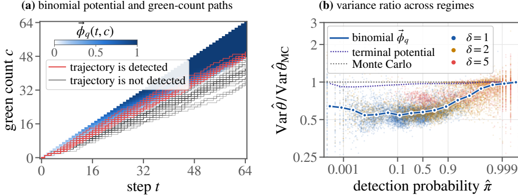
Figure 3: Panel (a) shows how sampled trajectories update the green-token count over 64 generation steps. Red trajectories are those whose final green-token count exceeds the detection threshold, while black trajectories remain below it. The background encodes the potential’s assigned probability of eventual detection at each step and green-count state, with white indicating probability zero. Red trajectories tend to pass through higher-probability regions, whereas black trajectories concentrate in low- or zero-probability regions. Panel (b) shows the variance reduction at different detection probabilities
