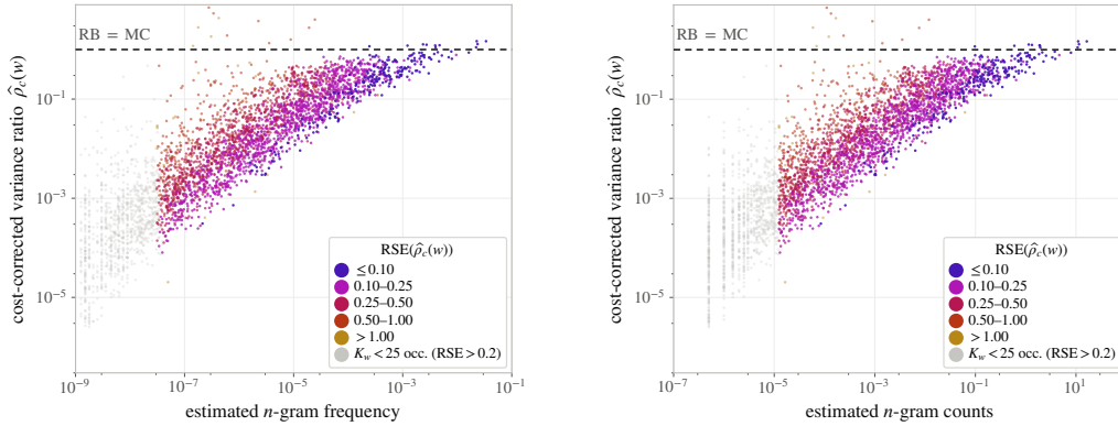
Figure 8: Cost-adjusted variance ratio against target rarity before the occurrence filter. Both panels show the frequency-estimator variance ratio, against estimated n -gram frequency (left) and expected count per document (right), before applying the occurrence filter to the independently estimated x -axis quantity. In the main figure, we retain only targets whose independent frequency estimate has RSE at most 20%, corresponding to at least 25 expected occurrences in the estimation sample, to restrict the analysis to more reliable estimates. Here, we show all 3,835 targets with positive estimated frequency and a finite positive variance ratio; this remains a subset of the 7,647-target inventory.
