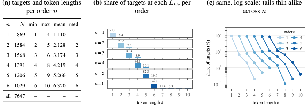
Figure 7: n -gram target inventory and token-length distribution. The n -gram task provides a controlled way to study targets of different lengths and, consequently, different marginalization costs, which scale with the number of GPT-2 tokens L_w in the target. (a) Number of targets at each order n , together with the minimum, maximum, mean, and median L_w of their canonical realizations. The inventory contains 7,647 targets in total. (b) Distribution of token lengths within each order. Increasing n shifts the inventory toward longer targets, while GPT-2 tokenization also induces within-order variation in L_w . (c) The same distributions on a log scale, showing that each order additionally contains a progressively thinning tail of targets requiring more tokens, and therefore more costly marginalization.
