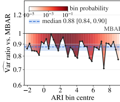
Figure 10: Variance ratio of the selected potential on the event-analysis experiment: chain-level variance of the cross-fitted estimator relative to MBAR, per ARI bin, over the 39 bins 20–58: the 38 bins on which MBAR’s own variance is itself measured to within 20%, plus bin 57 (at 25%), kept so that the range is contiguous; shading gives the bin probability, the dashed line the median (0.88) and the band its 95% interval. All 64 populated bins are in Fig. 12.
