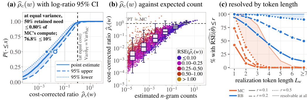
Figure 6: Fig. 2 for expected counts. Cost-adjusted variance ratio \hat{\rho}_c(w) for n -gram count estimation under the per-target cost proxy L_w + 1 . (a) Empirical cumulative distribution over 4,149 targets with bootstrap RSE at most 2, with approximate 95% log-ratio confidence bounds. (b) Ratio versus estimated expected count per document for the 2,831 targets with at least 25 expected occurrences in the independent frequency bank. (c) Fraction of targets whose count estimate reaches each RSE threshold, grouped by token length, at the same sample size M = 4,000 for both estimators. Dashed parity lines in (a–b) mark equal variance at equal cost under the proxy; in (c), line styles distinguish RSE thresholds.
