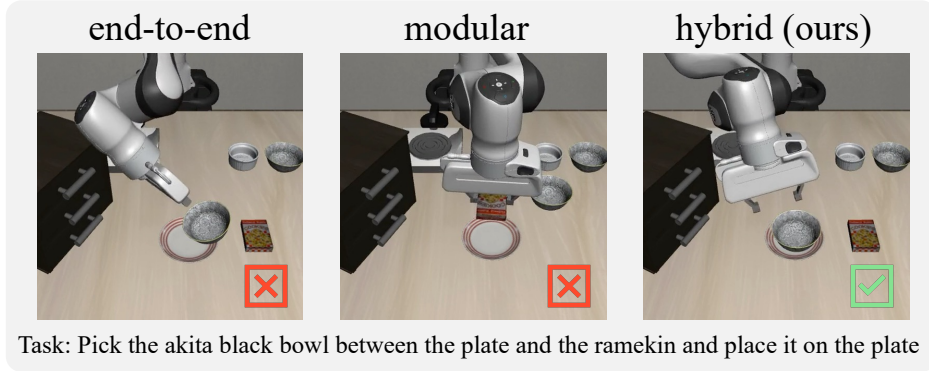
Figure 1 Additional LIBERO-Pro comparison on “Pick the akita black bowl between the plate and the ramekin and place it on the plate,” complementing Figure 4 in the main text. RoboAware-EO approaches with a misaligned gripper and fails to secure the bowl. RoboAware-MO completes a grasp but selects the wrong object (the cookie box). RoboAware grounds the spatially described bowl and finishes the pick-and-place, succeeding by switching policy families across P^5 boundaries.
