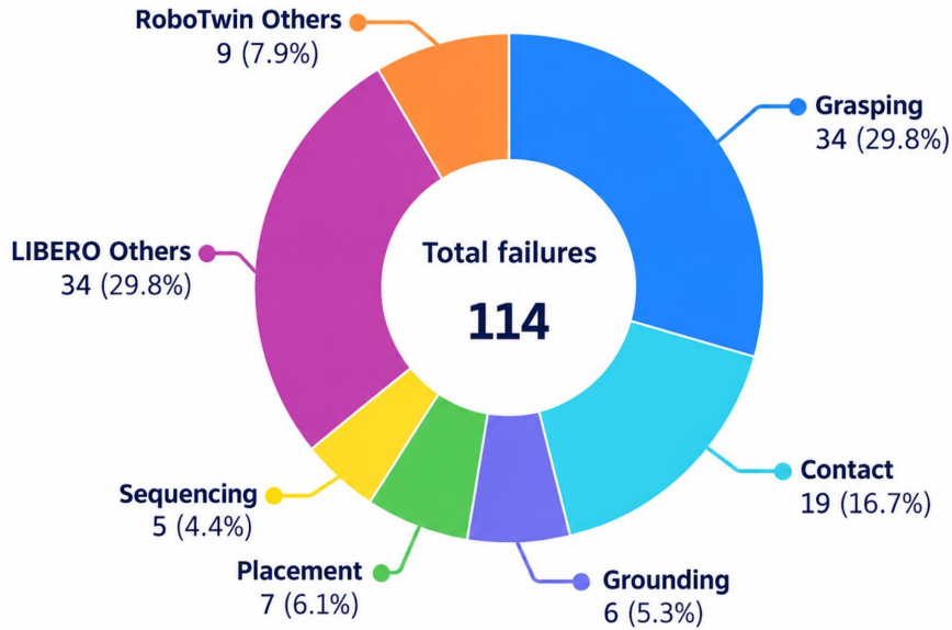
Figure 2 Failure modes of the unsuccessful rollouts. Grasping instability is the largest identified failure mode (29.8%), followed by constrained contact or insertion failures (16.7%). Grounding, placement, and multi-object sequencing account for 5.3%, 6.1%, and 4.4%, respectively. Others (37.7%) denotes failed rollouts for which the saved evaluation records are insufficient to identify a specific cause (29.8% from LIBERO-Pro and 7.9% from RoboTwin).
