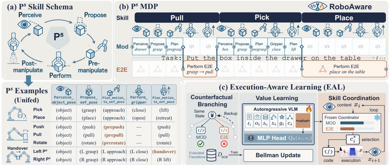
Figure 1 Overview of RoboAware. (a) The P^5 skill schema decomposes each skill into five stages—perceive, propose, pre-manipulate, perform, and post-manipulate—and unifies primitive skills (e.g., pick, place, push, pull) and compositional skills (e.g., handover) under one representation. (b) A hierarchical MDP selects a policy family c_i \in \{\text{Mod}, \text{E2E}\} at each P^5 stage decision boundary; a coding agent then generates each corresponding code block a_i . (c) EAL learns family-conditioned coordination: SCB evaluates modular and end-to-end branches from the same restored state into D_{SCB} , Q-learning yields Q_\theta(x, c) , and at test time a frozen coordinator selects best c_i to condition code generation and execution.
