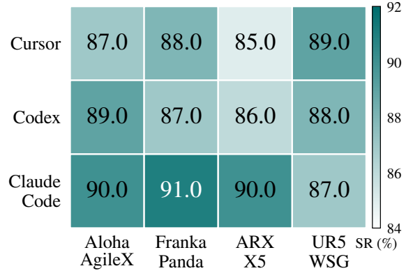
Figure 6 RoboTwin 2.0 success rates (%) on a four-task subset across coding-agent backends (rows) and embodiments (columns). Color bar shows the SR range.
