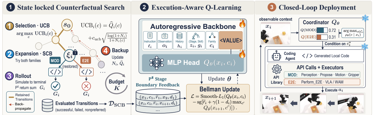
Figure 2 Method overview of EAL in RoboAware. (1) State-locked counterfactual search repeats Selection (UCB), Expansion (SCB paired Mod/E2E branches from a restored \xi_i ), Rollout (suffix return G_i ), and Backup within budget K , retaining successful, failed, and nonpreferred transitions in \mathcal{D}_{\text{SCB}} . (2) A VLM backbone with an MLP head maps context–family tokens ending in \langle \text{VALUE} \rangle to Q_\theta(x_i, c_i) , trained by Bellman updates on skill-completion and terminal-task feedback. (3) At deployment, frozen Q_\theta induces \rho_\theta and selects c_i^* = \arg \max_c \rho_\theta(c | x_i) ; a frozen coding agent generates a local code block against the fixed API library and executes it, looping on observable feedback at each P^5 boundary.
