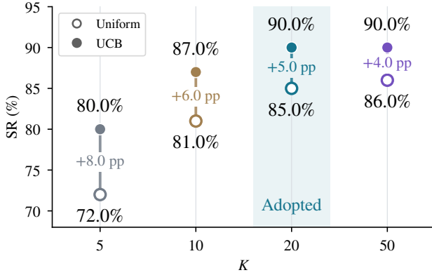
Figure 5 Average RoboSuite success rates (%) across budgets K \in \{5, 10, 20, 50\} . Hollow & filled circles denote RoboAware-UA & RoboAware. We adopt K=20 .
