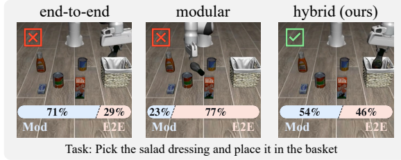
Figure 4 A representative LIBERO-Pro task comparison and visualization of the responsibility preference distribution \rho_\theta for RoboAware, RoboAware-EO, and RoboAware-MO.
