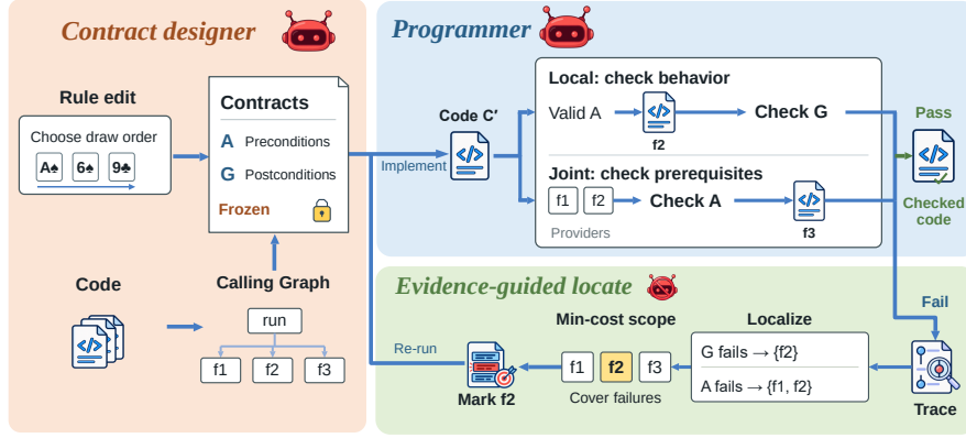
Figure 2: Contract-guided rule implementation. Revised rules are translated into function contracts that guide code edits and execution checks. Failure traces guide the selection of functions to repair, and the updated code is rechecked under the same contracts.
