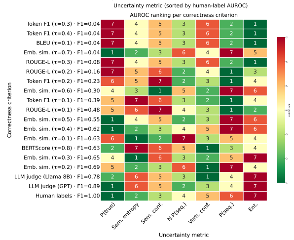
(b) Qwen 7B, AmbigQA (ambiguous)
