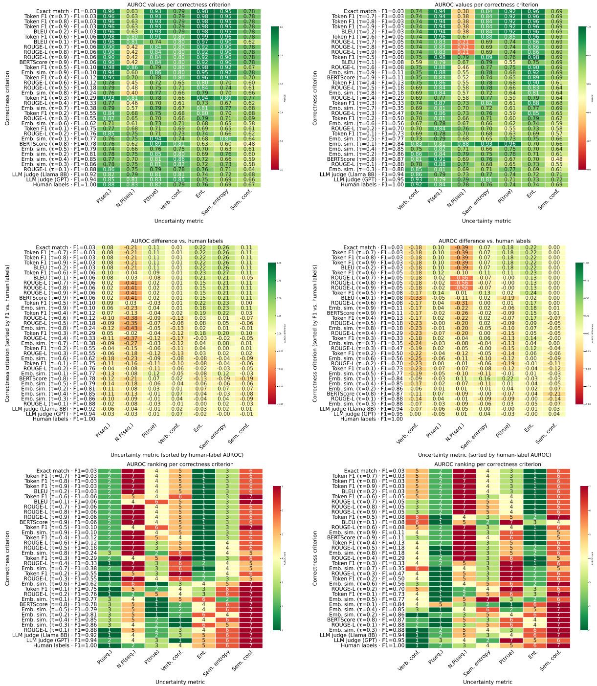
Figure 8: Top row shows AUROC values, middle row shows differences between oracle and system AUROC values and bottom row rankings for various uncertainty quantifiers (ordered from left to right in a descending order of performance) and correctness functions (ordered from top to bottom in an increasing order of quality).
