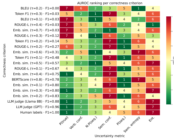
(a) Llama 3B, AmbigQA (ambiguous), New annotator
