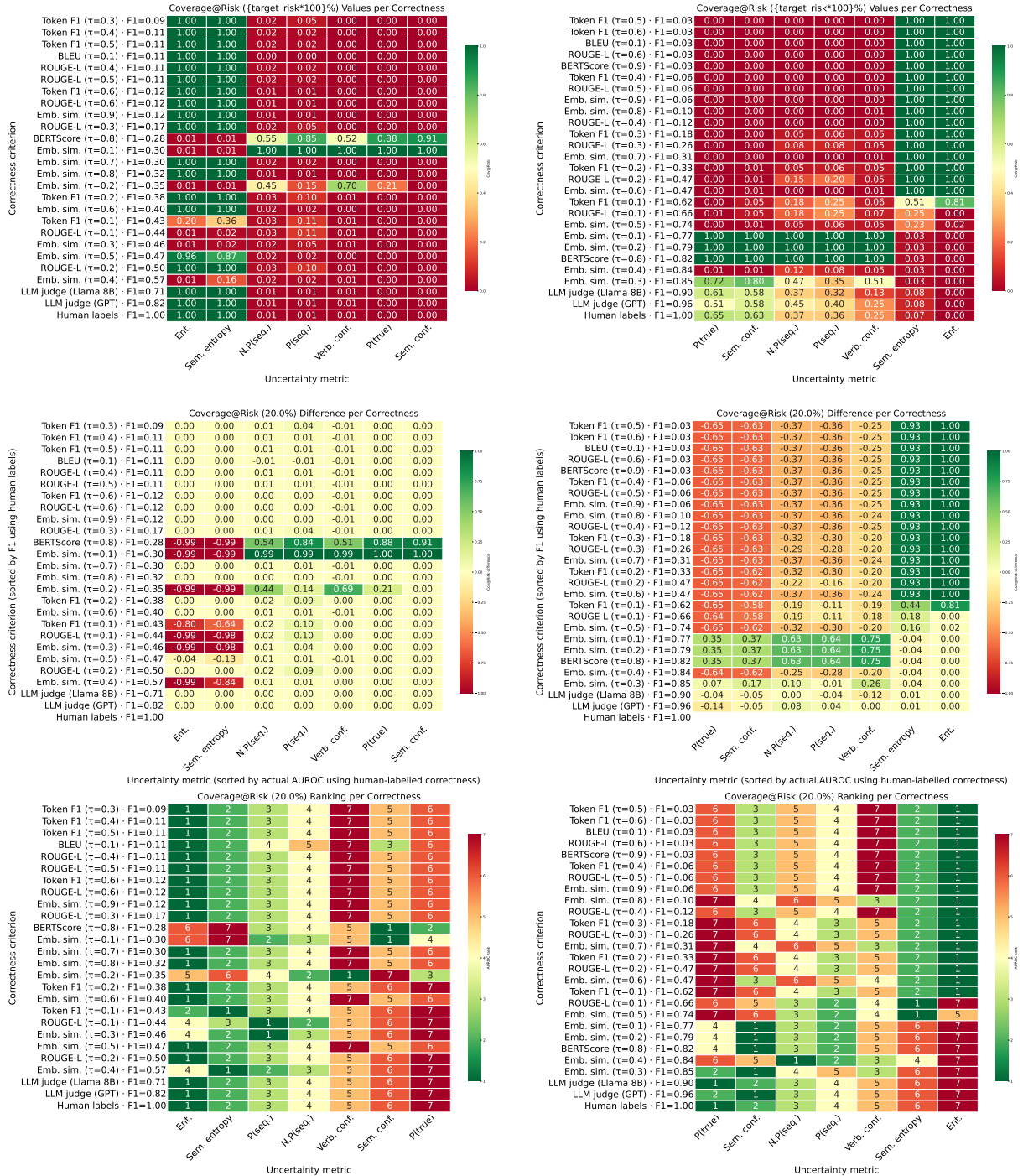
Figure 24: Top row shows Coverage at fixed risk values, middle row shows differences and bottom row rankings for various uncertainty quantifiers.
