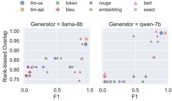
Figure 4: F1 scores ( \uparrow ) for judges against the RBO score ( \uparrow ) of human- vs judge-powered UQ rankings. Even within a narrow range of F1 values ( i.e. , similar-quality judges), there’s considerable variability in their UQ evaluation performance.
