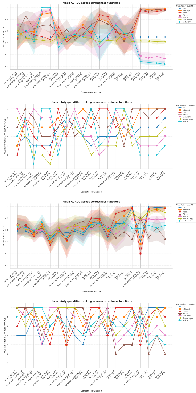
Figure 20: Top two plots correspond to Qwen 0.5B, AmbigQA (ambiguous). Bottom two plots correspond to Qwen 7B, AmbigQA (ambiguous).
