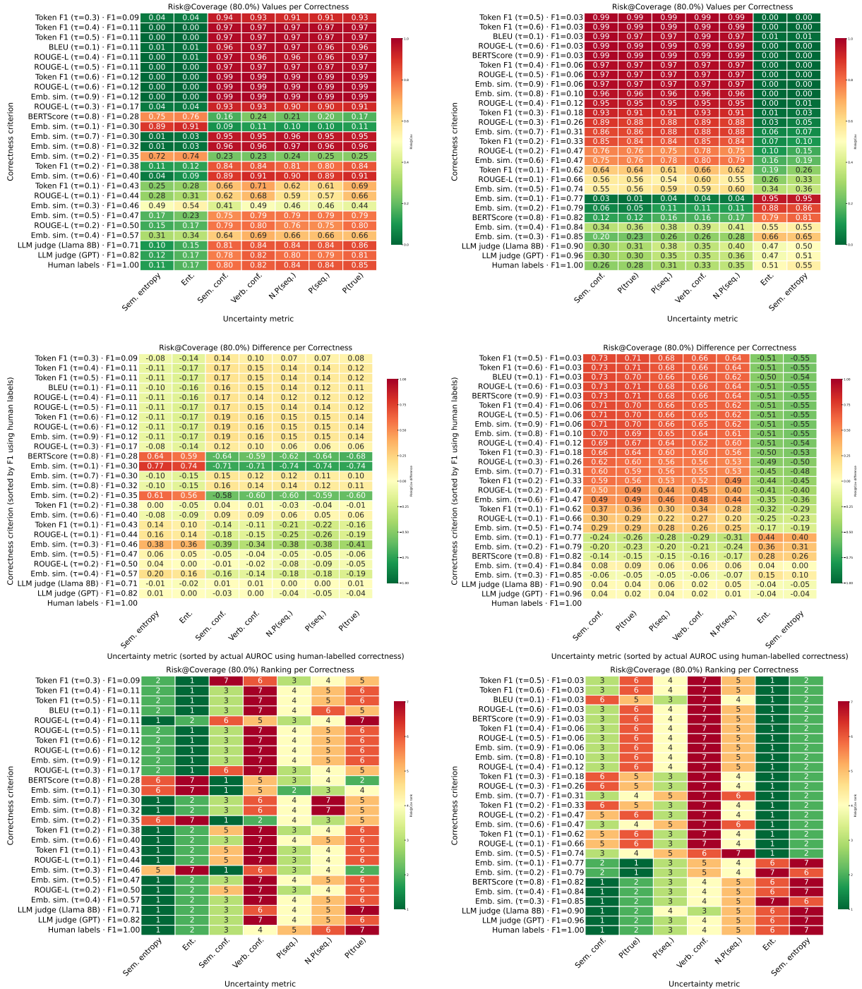
Figure 22: Top row shows risk at fixed coverage values, middle row shows differences and bottom row rankings for various uncertainty quantifiers.
