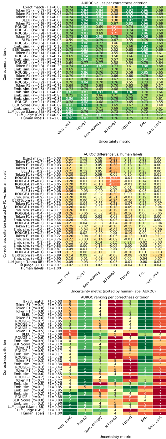
(a) Llama 8B, TriviaQA, New annotator
