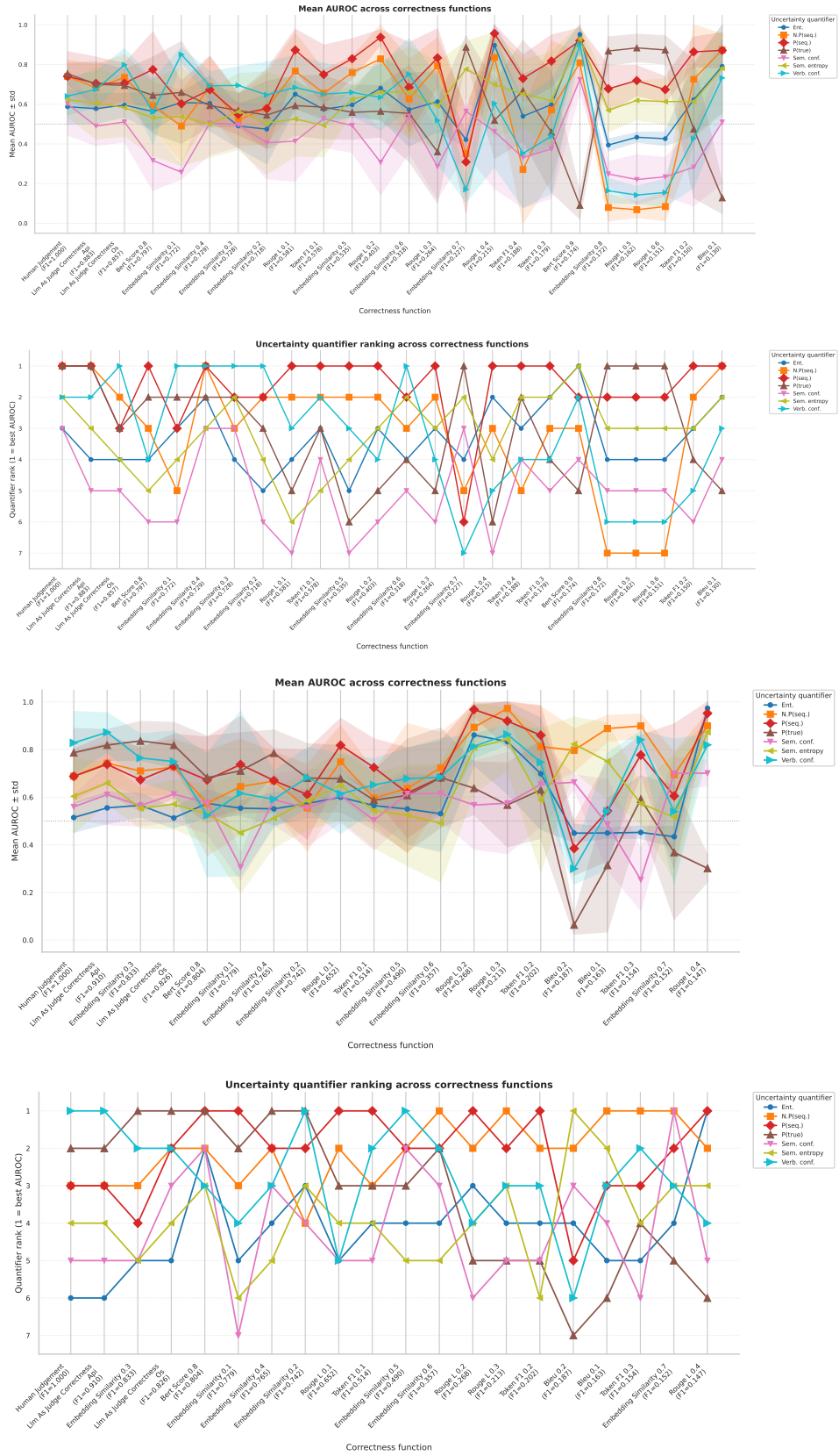
Figure 19: Top two plots correspond to Llama 3B, AmbigQA (ambiguous). Bottom two plots correspond to Llama 8B, AmbigQA (ambiguous).
