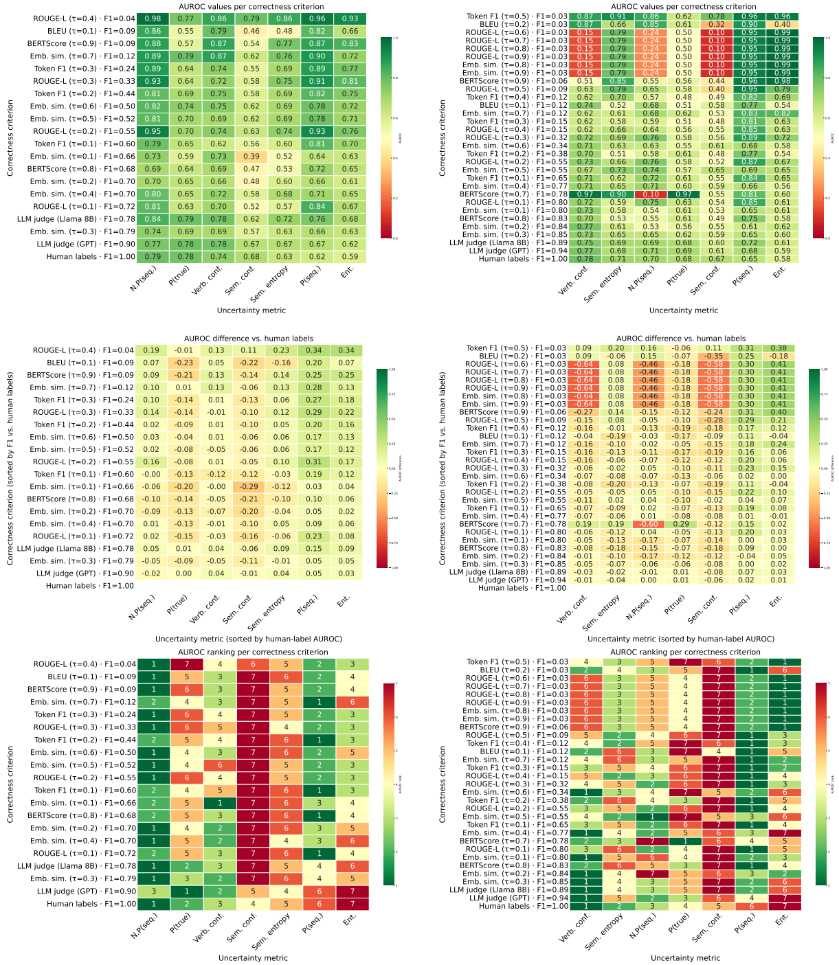
Figure 10: Top row shows AUROC values, middle row shows differences between oracle and system AUROC values and bottom row rankings for various uncertainty quantifiers (ordered from left to right in a descending order of performance) and correctness functions (ordered from top to bottom in an increasing order of quality).
