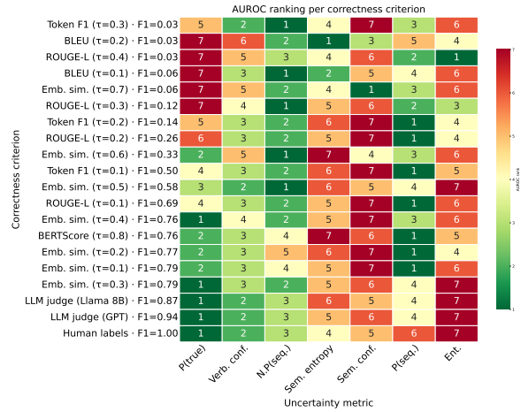
(b) Llama 8B, AmbigQA (ambiguous), Original annotator
