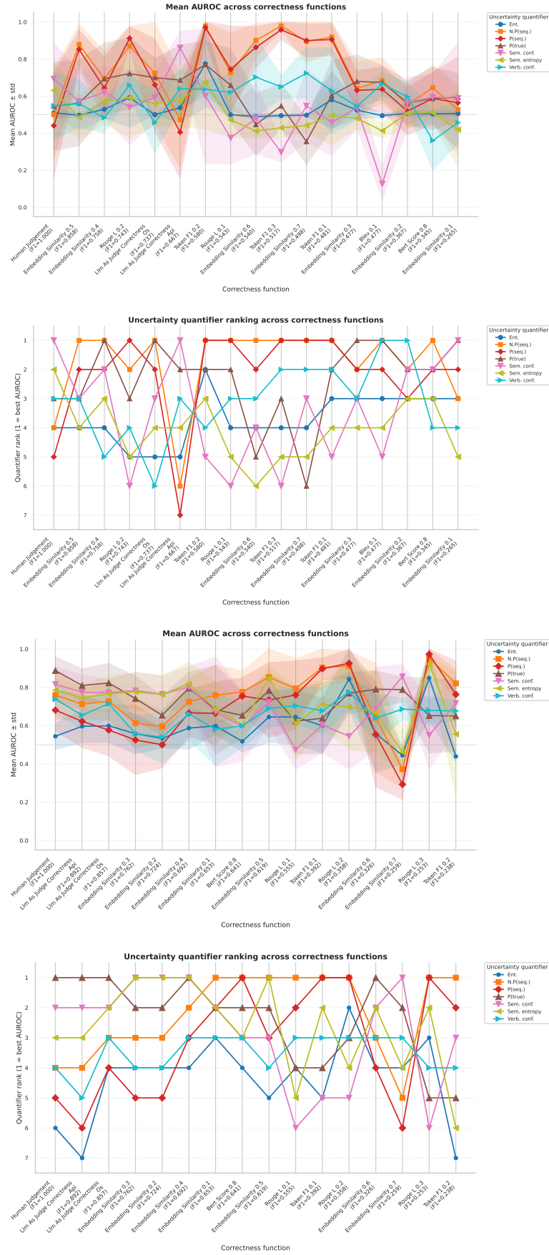
Figure 18: Top two plots correspond to Qwen 0.5B, AmbigQA (unambiguous). Bottom two plots correspond to Qwen 7B, AmbigQA (unambiguous).
