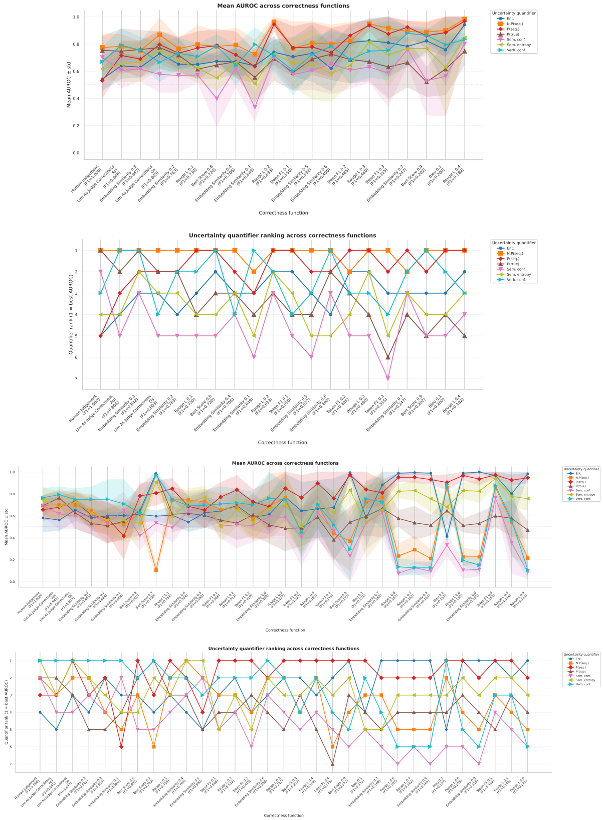
Figure 17: Top two plots correspond to Llama 3B, AmbigQA (unambiguous). Bottom two plots correspond to Llama 8B, AmbigQA (unambiguous).
