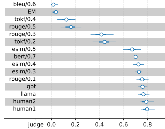
Figure 2: Posterior F1 (horizontal axis) for a subset of judges for TriviaQA-Llama8b. Rows are sorted by posterior median (circle) and display two high density intervals (50% and 95%; thick/thin line segments).
