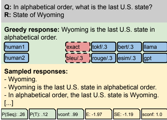
Figure 3: An example data point of question (Q) and references (R) from TriviaQA and responses by Llama 8B. The greedy response is judged manually and automatically (e.g., via exact match, BLEU, BertScore, LLM judges, etc.); positive judgements are blue/solid, negative are red/dashed. We compute various UQs: some (e.g., P(True)) qualify the greedy response specifically (in green), others (e.g., entropy) qualify the entire conditional distribution (estimated using samples; in yellow).
