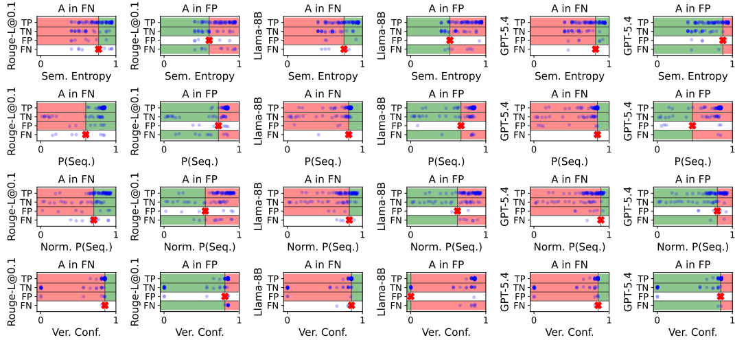
Figure 6: Error impacts on AUROC for various quantifiers under best automated judges, for TriviaQA-Llama8B. For a detailed guide on how to interpret this figure, see Section 5.2.
