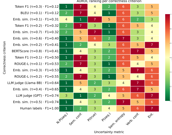
(a) Qwen 0.5B, AmbigQA (unambiguous)
