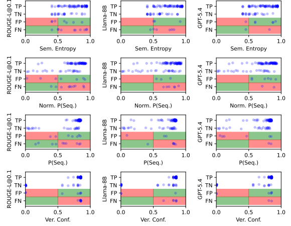
Figure 5: Error trade-offs in SP (with threshold 0.5) for various UQs under best automated judges (TriviaQA-Llama8B). For a detailed guide on how to interpret this figure, see Section 5.2.
