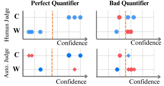
Figure 1: An informative UQ (top-left) assigns higher confidence to responses that humans deem correct (C) than to those that humans deem wrong (W), allowing a decision maker to be selective ( e.g. , by rejecting lower-confidence responses wrt a threshold (dashed line)). If assigned confidences do not neatly separate Cs from Ws (top-right), the UQ leads to selection errors (shown in red). The degree of separation gives us a criterion to choose amongst UQs. But when judgement is automated (bottom), as routinely done in UQ evaluation, judgement errors (C→W or W→C; shown as diamonds) distort our view of the relative merits of the UQs. This affects informative UQs most: on the left, we go from 0/6 to 3/6 selection errors (2 rejected Cs and 1 accepted W), while on the right we go from 3/6 to 4/6 errors.
