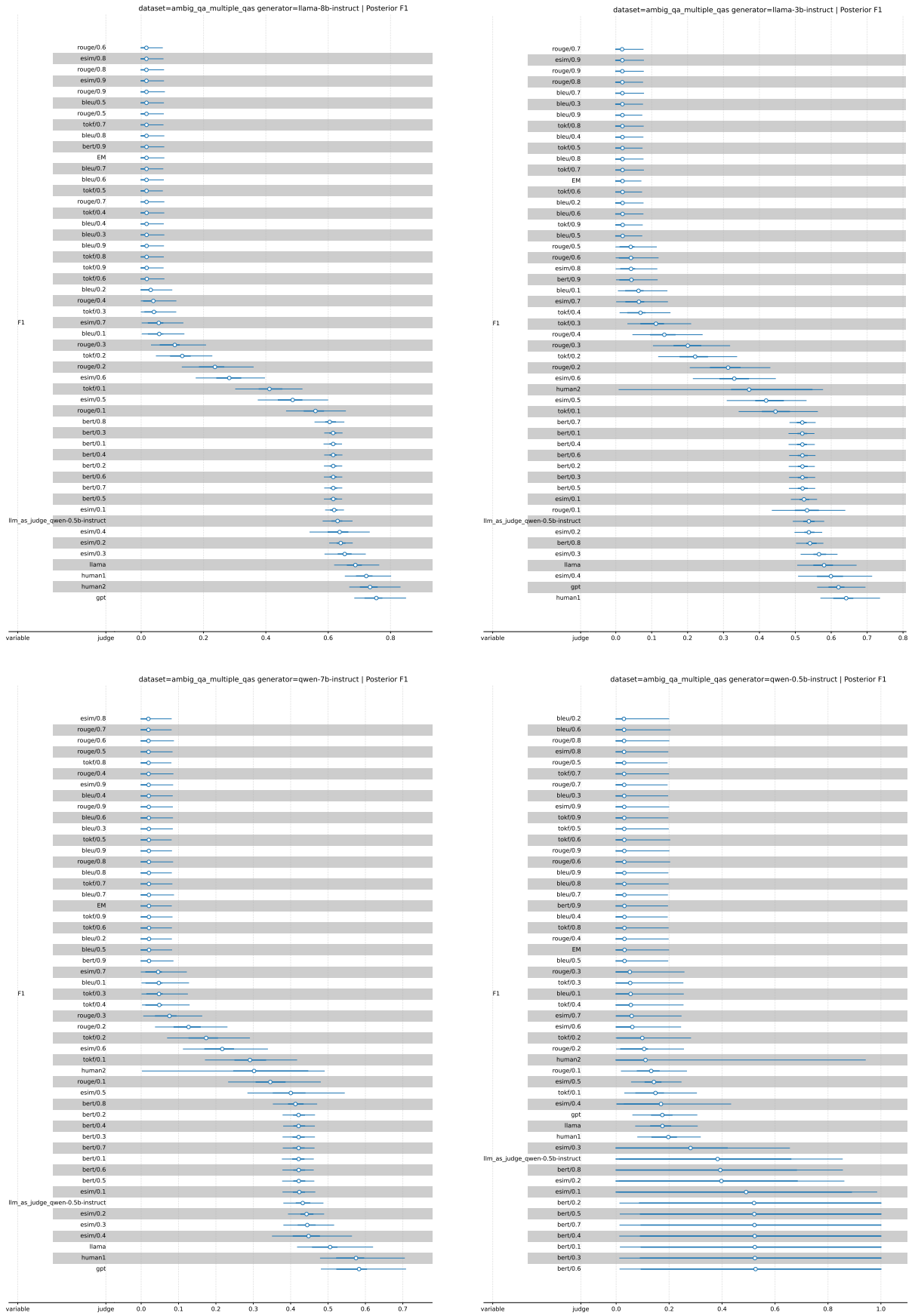
Figure 27: F1 distributions for AmbigQA (ambiguous) dataset and Llama 8B (top left corner), Llama 3B (top right corner), Qwen 7B (bottom left corner) and Qwen 0.5B (bottom right corner).
