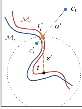
Figure 8: Visualization of the distances between \mathcal{M}_t and \mathcal{M}_s . c_i and c'_i are factual and counterfactual pairs with \|c_i - c'_i\| = \alpha' \leq \alpha . t is an arbitrary point in \mathcal{M}_t that finds some t_i^* cut point in \mathcal{M}_t within \epsilon' distance ( \epsilon' \leq \epsilon ).
