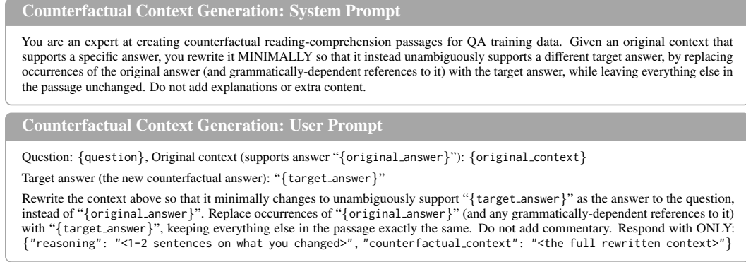
Figure 2: Counterfactual context generation prompts. System and user prompts used to minimally modify the factual context C into a counterfactual context C' that supports the target answer A' .
