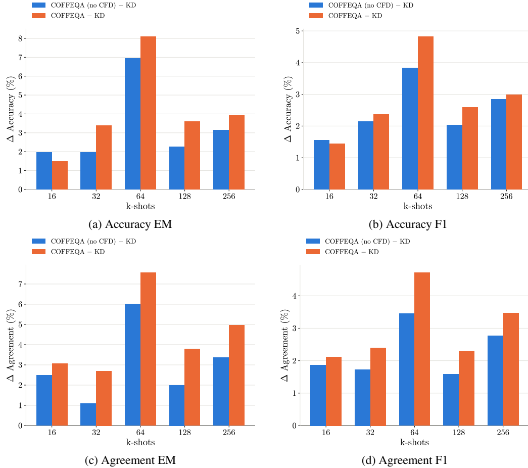
Figure 9: Effect of CFD verification on COFFEQA. Performance gains over standard KD ( \Delta = \text{COFFEQA} - \text{KD} ) are shown across different few-shot budgets k . We compare COFFEQA without CFD verification against the full COFFEQA framework with CFD verification ( \tau = 0.3 ). Panels (a) and (b) report accuracy EM and F1 gains, while panels (c) and (d) report teacher-student agreement EM and F1 gains. CFD verification generally yields larger improvements, demonstrating the benefit of validating generated counterfactuals before distillation.
