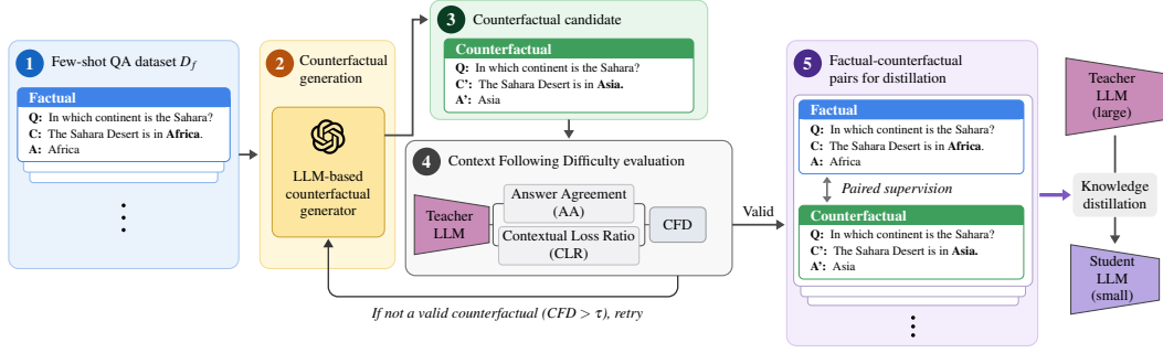
Figure 1: Counterfactual-guided few-shot distillation framework. We begin with (1) a few-shot factual QA dataset \mathcal{D}_f and (2) generate a counterfactual candidate for a factual sample. (3) The generated counterfactual is evaluated using the teacher model with (4) our proposed Context Following Difficulty (CFD) metric and accepted if it satisfies the CFD threshold \tau . (5) The CFD-validated counterfactuals are then paired with their corresponding factuals and used to distill the student model.
