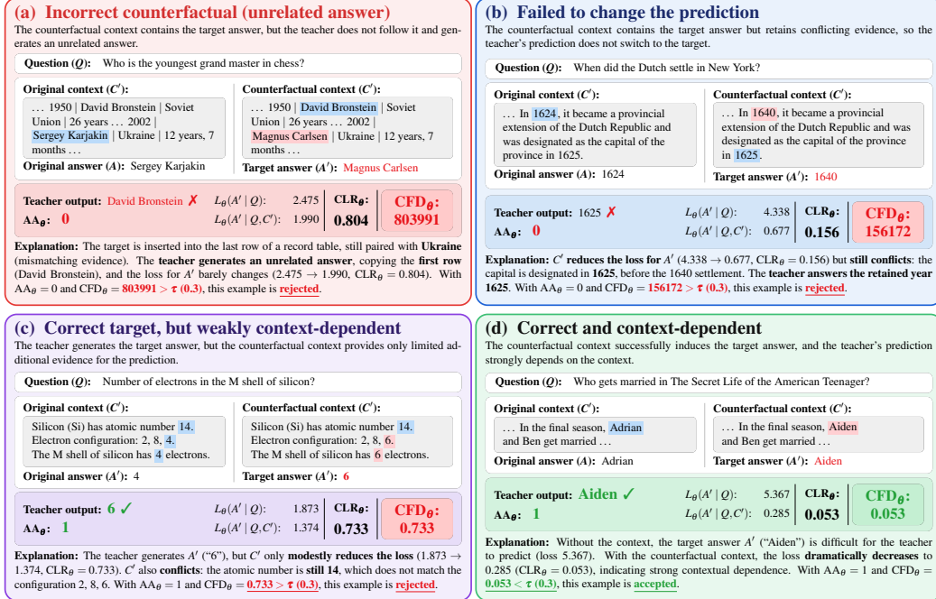
Figure 4: Illustrative examples of CFD-based counterfactual evaluation from the NQ dataset. The four cases demonstrate how Answer Agreement (AA) and Contextual Loss Ratio (CLR) complement each other in evaluating generated counterfactual candidates.
