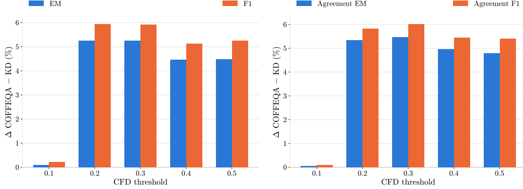
Figure 10: CFD threshold ablation. Effect of the CFD threshold \tau on COFFEQA using T5 on TriviaQA. The bars show the improvement of COFFEQA over standard KD ( \Delta = \text{COFFEQA} - \text{KD} ), averaged across k \in \{16, 32, 64, 128, 256\} and five random seeds. The left plot shows the improvement in accuracy measured by EM and F1, while the right plot shows the improvement in teacher-student agreement measured by EM and F1.
