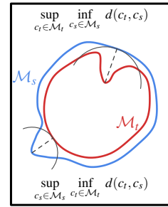
Figure 3: Visualizing the Hausdorff distance between \mathcal{M}_t and \mathcal{M}_s .
