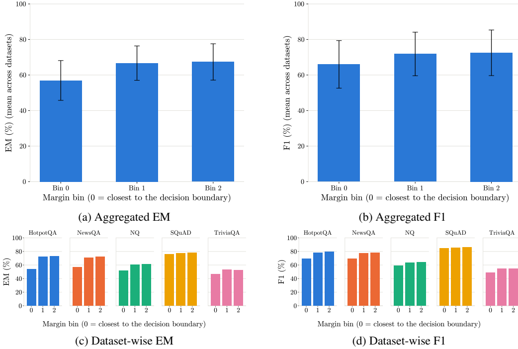
Figure 6: KD performance as a function of the teacher prediction margin. Factual samples are grouped into three bins according to their average token-level prediction margins, with Bin 0 containing the smallest margin samples and Bin 2 containing the largest margin samples. Smaller margins are used as a proxy for greater proximity to the teacher’s decision boundary. Knowledge distillation is performed separately using 100 factual samples from each bin, maintaining the same distillation budget across all three settings. Panels (a) and (b) report EM and F1 averaged across the five in-domain datasets, respectively, while panels (c) and (d) report the corresponding dataset-wise results. Distillation using samples from the smallest margin bin generally results in lower performance than using samples from the larger margin bins.
