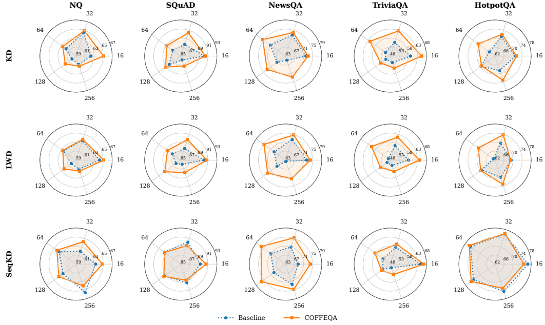
Figure 11: Teacher-student F1 agreement of KD, LWD, and SeqKD with and without COFFEQA across datasets and k -shot settings using T5. COFFEQA generally achieves higher agreement across the distillation baselines. Spokes denote k -shot settings, and radial axis F1 score ranges are adjusted independently by dataset for visualization.
