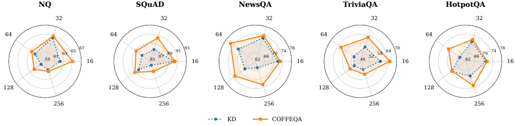
Figure 5: Teacher-student F1 agreement of standard KD and COFFEQA across datasets and k -shot settings using T5. COFFEQA generally achieves higher agreement than the baseline. Spokes denote k -shot settings, and radial axis F1 score ranges are adjusted independently by dataset for visualization.
