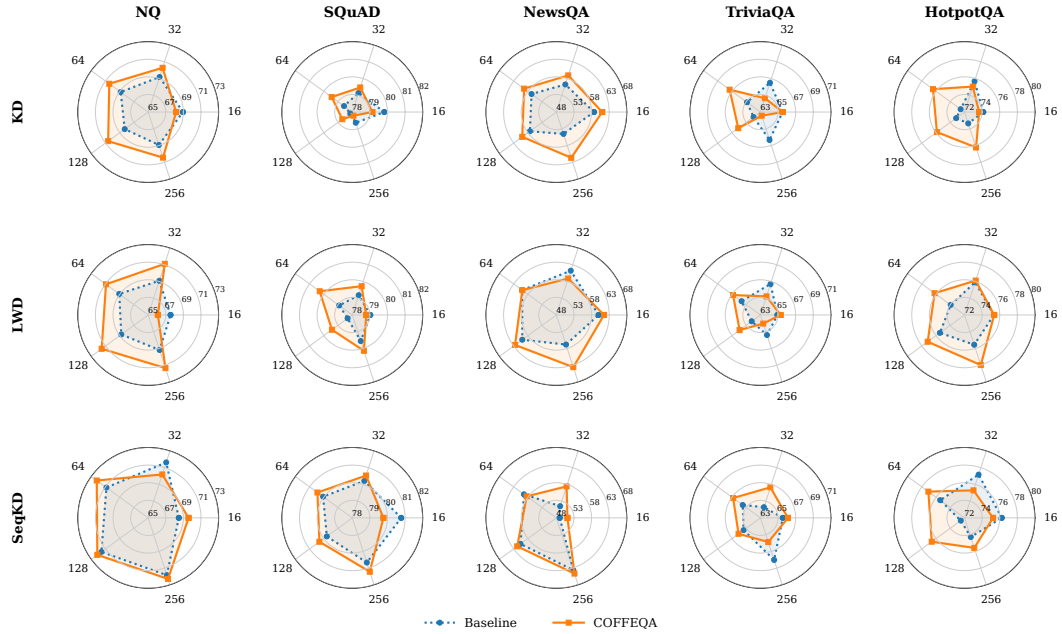
Figure 12: Teacher-student F1 agreement of KD, LWD, and SeqKD with and without COFFEQA across datasets and k -shot settings using Qwen2.5. COFFEQA generally achieves higher agreement across the distillation baselines. Spokes denote k -shot settings, and radial axis F1 score ranges are adjusted independently by dataset for visualization.
