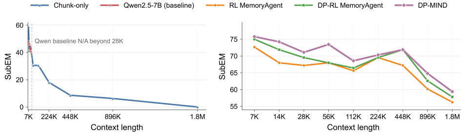
Figure 2: Results on RULER-HQA under \epsilon = 7 . Chunk-only inference uses chunk-wise memory processing and can scale to long contexts, but its utility drops quickly without RL-based memory optimization. DP-MIND achieves the best overall performance.
