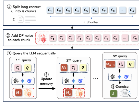
Figure 1: Workflow of DP-MIND.
