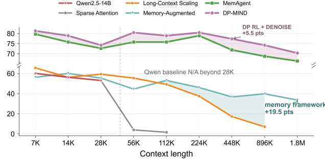
Figure 3: Scaling performance on RULER-HQA with Qwen2.5-14B under \epsilon = 7 . DP-MIND consistently achieves the best overall performance, while the advantage of memory-based inference becomes more pronounced as the context length increases.
