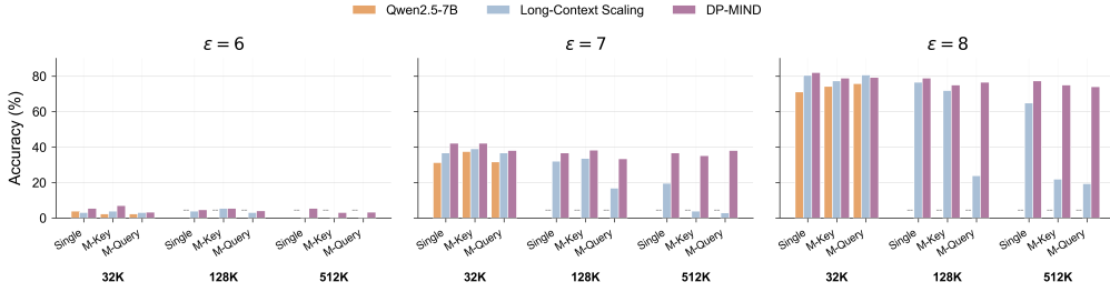
Figure 4: NIAH results under different privacy budgets and context lengths. Results are reported on Single, Multi-Key (M-Key), and Multi-Query (M-Query) with length ranging from 32k to 512k.
