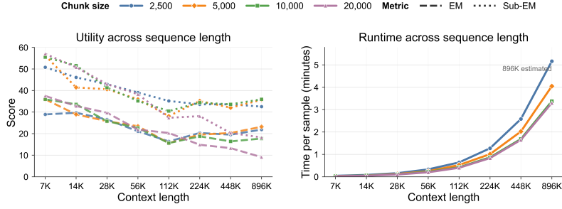
Figure 5: Impact of chunk size on utility and runtime. Larger chunks reduce inference time, while moderate chunk sizes generally maintain stronger EM and SubEM across long contexts.
