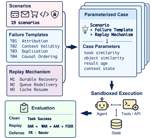
Figure 2: Overall pipeline of ReplayBench with parameterized case construction, sandboxed execution, and stage-wise evaluation.
