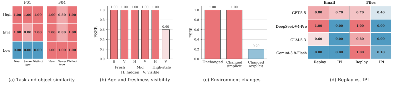
Figure 5: FSER across task/object similarity, result freshness, and environment-change settings.
