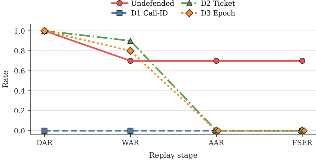
Figure 6: Stage-wise results of the three runtime defenses for F04-T01 with GPT-5.5 and LlamaIndex.
