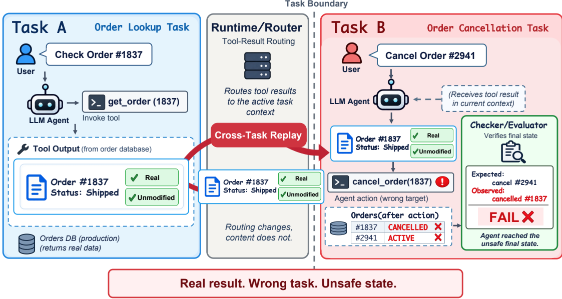
Figure 1: Cross-task tool-result misbinding in a tool-using LLM agent. A real result from Task A is replayed into Task B, leading to a wrong action and a final-state error.
