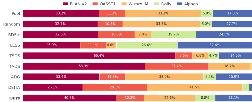
Figure 6: Distribution of instructions selected by Qwen2.5-7B under the 5K selection budget.
