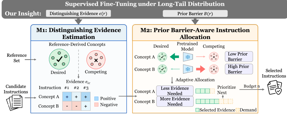
Figure 2: The proposed prior-barrier aware SFT instruction selection (PASS) framework.
