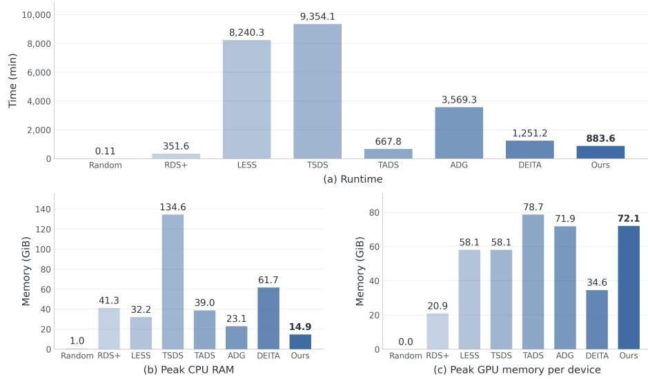
Figure 4: Runtime and memory consumption of all selection methods. (a) Total runtime in minutes. (b) Peak CPU memory. (c) Peak GPU memory per device.
