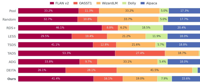
Figure 5: Distribution of instructions selected by Mistral-7B under the 5K selection budget.
