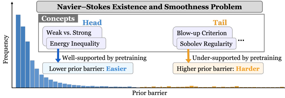
Figure 1: Illustration of the long-tail distribution of prior barriers using the Navier–Stokes existence and smoothness problem as an example.
