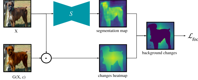
Fig. 5. Object focus module OF : Generated images are compared to the original ones and all pixels modified outside the segmentation maps are penalized. This helps to keep a background consistency between original and generated images.
