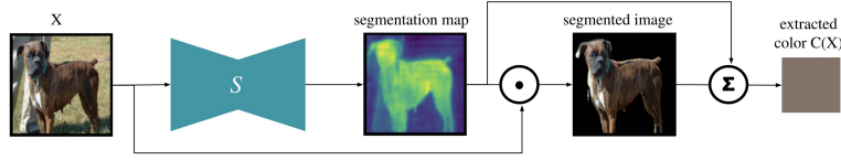
Fig. 3. Color estimation module C : from the segmentation map given by the segmentation model S , the weighted mean C(X) is computed to represent the color of the object.
