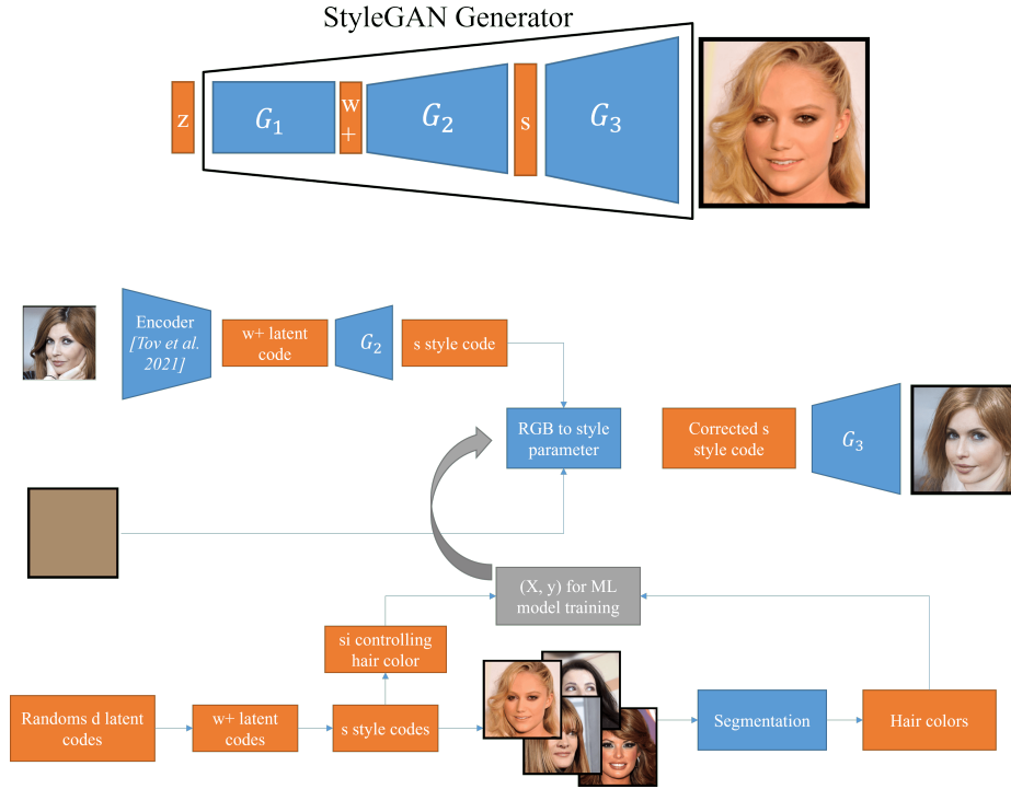
Fig. 8. Top graphic represents a simplified decomposition of StyleGAN’s model Generator. In particular it shows the two intermediate states that are used, w+ and s . Bottom graphics illustrates the process used to achieve color control with StyleGAN’s Generator.
