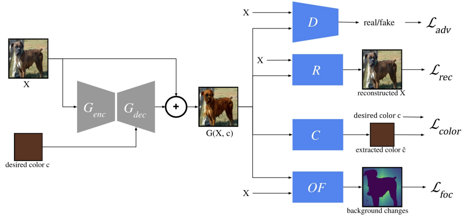
Fig. 2. General organization of our framework. Generated images are evaluated through the four defined modules that design G 's training: C , D , OF and R . G actually predicts a difference that is applied to the input image.
