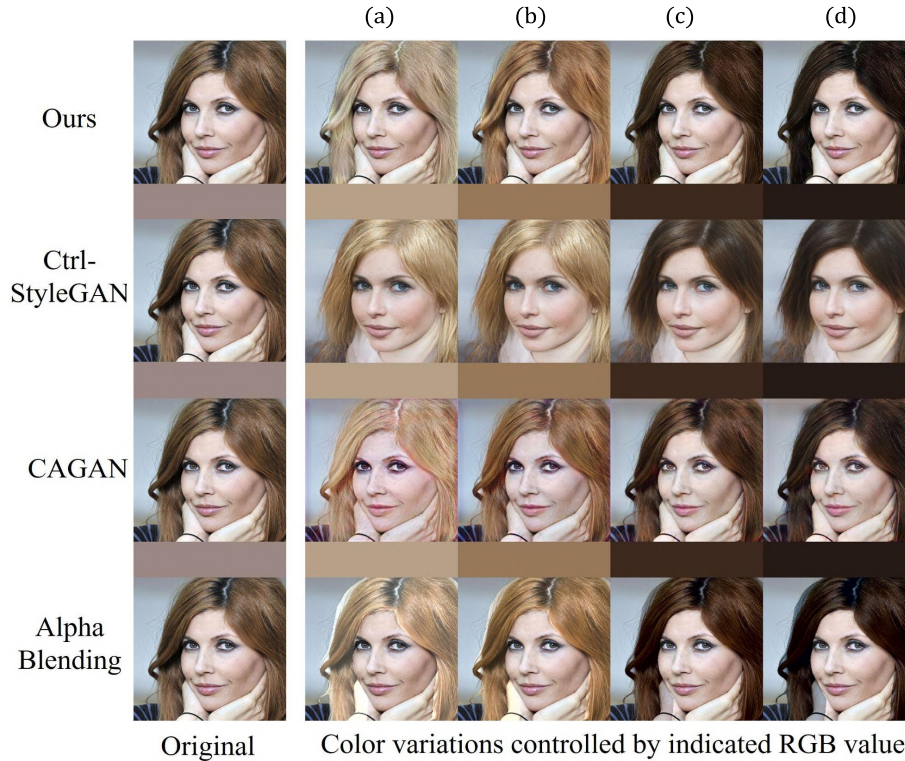
Fig. 6. Comparison of different methods for hair coloring. The desired hair color is illustrated on each column between rows.
