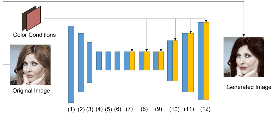
Fig. 7. Illustration of conditions incorporation in the generator. The colors are concatenated with the outputs of the convolutional layers. Finally the input image is added to the network’s output. Numbers refer to the outputs of the different layers described in table 6.1.
