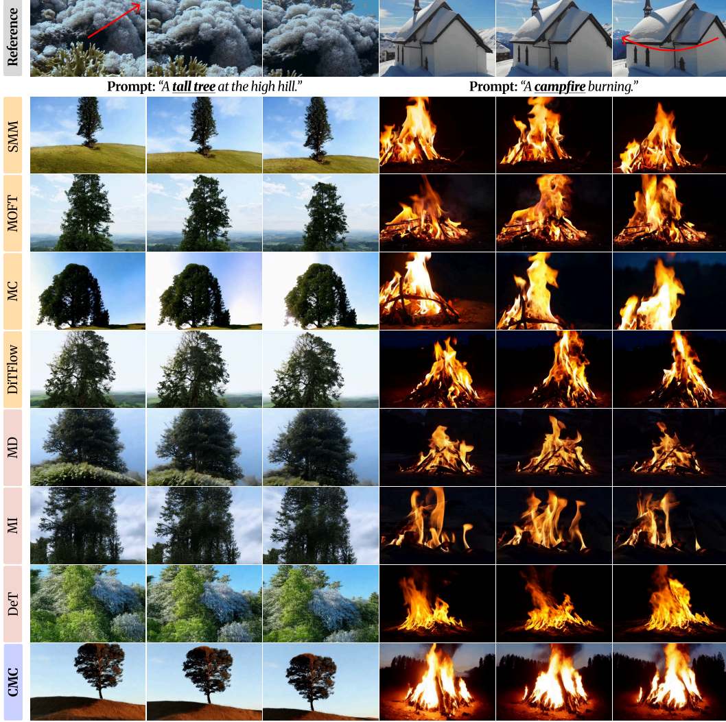
Figure S1: Additional qualitative comparison with baselines. The red arrow indicates the camera movement direction. Best seen as video: link .
