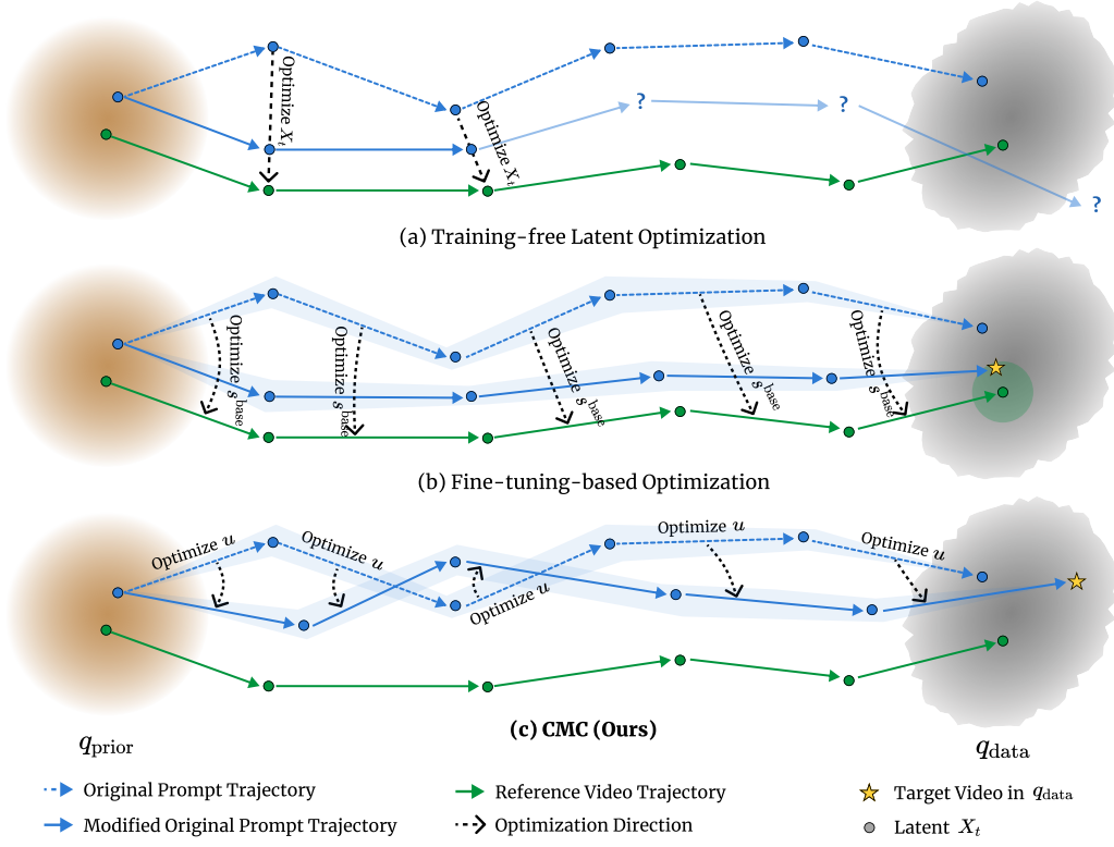
Figure 2: Method Comparison. Existing methods vs. our control-based approach.
