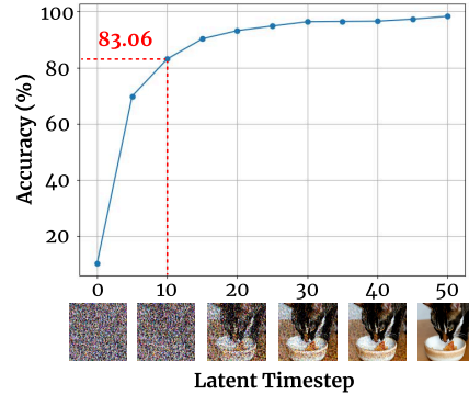
Figure 4: Quantitative analysis on motion formation timestep.
