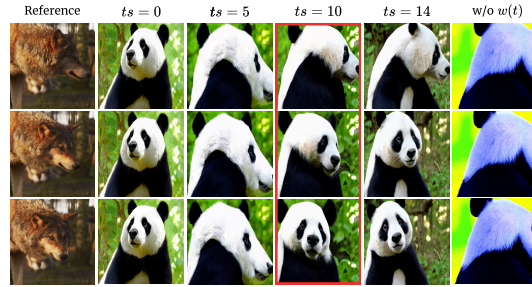
Figure 6: Ablation study. ts denotes the motion injection timestep ( ts = 0 corresponds to the base T2V). Motion aligns with the reference from ts = 10 . Removing w(t) leads to degenerated outputs.
