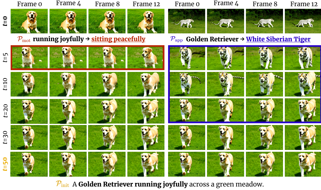
Figure 3: Qualitative analysis on motion formation timestep. The y -axis indicates the switching timestep ( t \in [0, 50] ) at which the initial prompt \mathcal{P}_{\text{init}} is switched to a new prompt \mathcal{P}_{\text{mot}} or \mathcal{P}_{\text{app}} . Left: Switching from \mathcal{P}_{\text{init}} to \mathcal{P}_{\text{mot}} shows that motion becomes largely established after early timesteps ( t = 10 ), with limited influence from subsequent prompts. Right: Switching to \mathcal{P}_{\text{app}} shows that non-motion can still change at later timestep ( t = 20 ).
