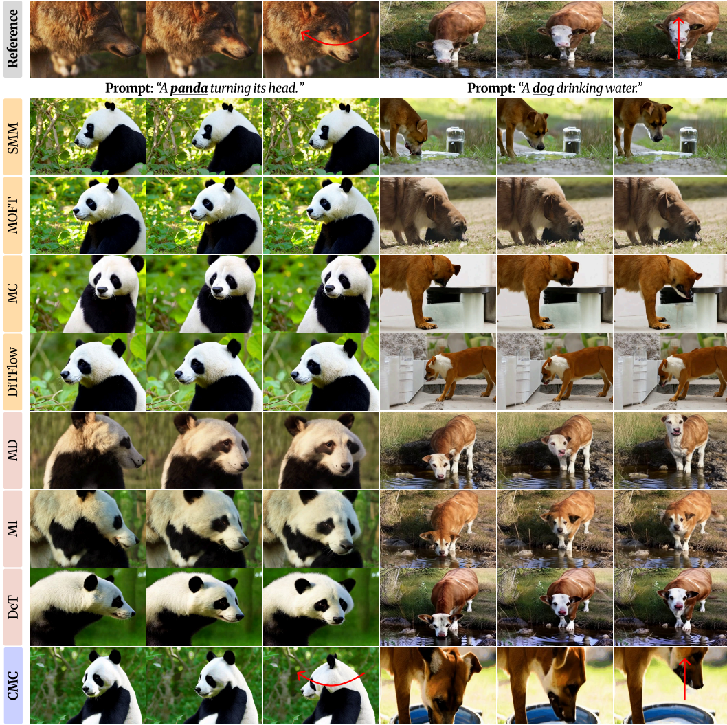
Figure 5: Qualitative comparison with baselines. CMC achieves precise motion customization while significantly mitigating content leakage. The red arrow indicates the movement direction.
