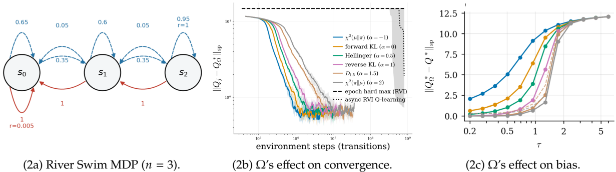
Figure 2: Comparison of regularizers from the \alpha -divergence family on the RiverSwim MDP. As predicted by the theory, convergence slows as \alpha increases at equal bias level.
