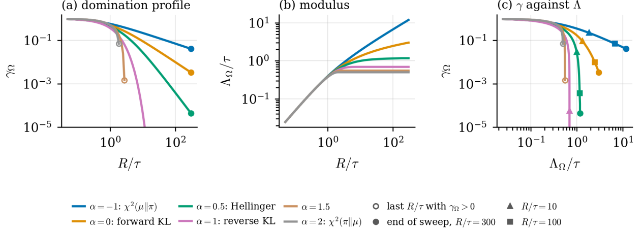
Figure 4: The objects of Definition 2 for the \alpha -divergences to a uniform \mu over two actions, and the resulting bias. (a) Domination profile \gamma_\Omega and (b) regularization modulus \Lambda_\Omega/\tau , both functions of R/\tau only. (c) The pair (\Lambda_\Omega/\tau, \gamma_\Omega) as R/\tau grows.
