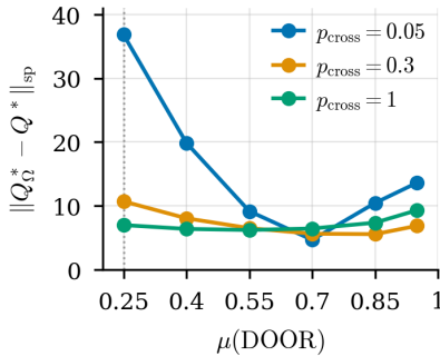
Figure 3: Bias \|Q_\Omega^* - Q^*\|_{\text{sp}} on Two Rooms against \mu(\text{DOOR}) , exact. Dotted line: uniform \mu .
