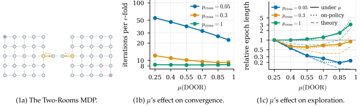
Figure 1: Empirical results on the Two-Rooms MDP. Biasing the reference policy \mu towards the bottleneck improves both convergence (b) and exploration (c).
