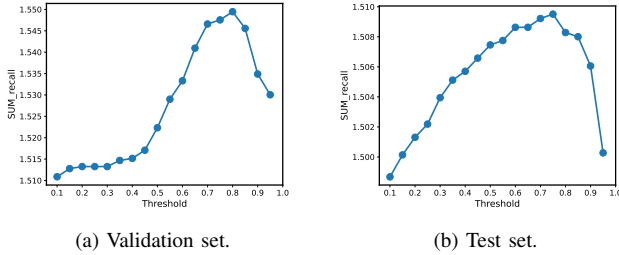
Fig. 8. ODCT threshold selection on the validation and test sets.
