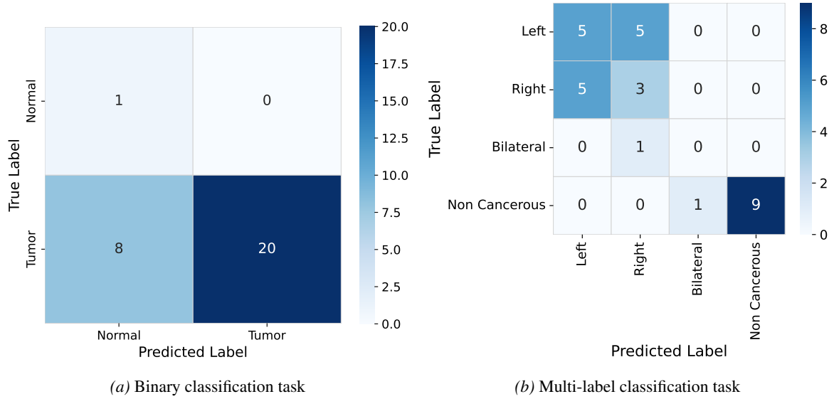
Figure 5. Confusion matrices of downstream tasks using PCA projections.
