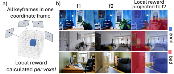
Figure 4: a) : illustration of voxel reward aggregation. b) : visualization of local reward projected to video frames.
