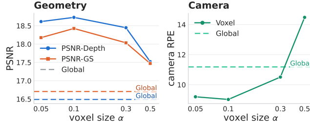
Figure 10: Effect of voxel size on geometry metric and camera following metrics. Both improve with finer voxel size up till 0.1 \times P90 scene depth.
