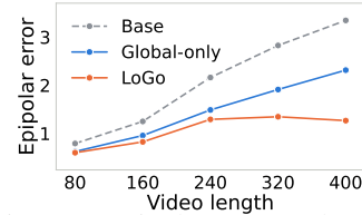
Figure 8: Epipolar error vs. length.
