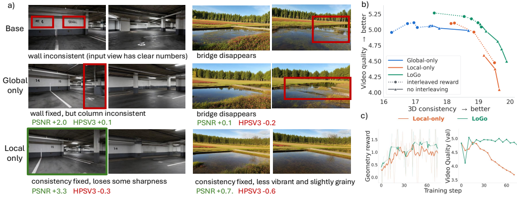
Figure 3: Motivation of LoGo. (a) A global reward fails to improve 3D consistency; local reward improves consistency, measured in PSNR, but degrades video quality, measured in HPSv3. This motivates combining the two in LoGo. (b) LoGo (green) extends the Pareto frontier in the consistency-quality tradeoff. (c) Reward curves and quality evaluation during training: local reward degrades video quality over time; LoGo improves consistency without compromising quality.
