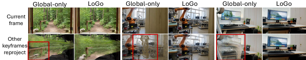
Figure 7: Global-only reward vs. LoGo. A 3D-consistent video should closely match its reprojections, though not perfectly, since keyframes in long videos overlap only sparsely. Global reward incurs inconsistencies, highlighted in red, such as hallucinated object (double railing), artifact (floater in the robot scene), and object appearance change (chair). LoGo, by combining global reward with local reward, effectively removes these inconsistencies.
