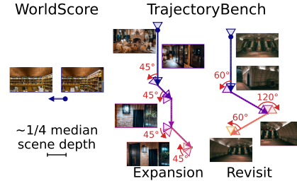
Figure 5: Camera trajectories of TrajectoryBench vs. WorldScore.
