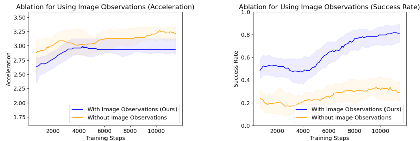
Fig. 9: Visual-observation ablation: acceleration (left) and success rate (right). Both variants retain proprioception.
