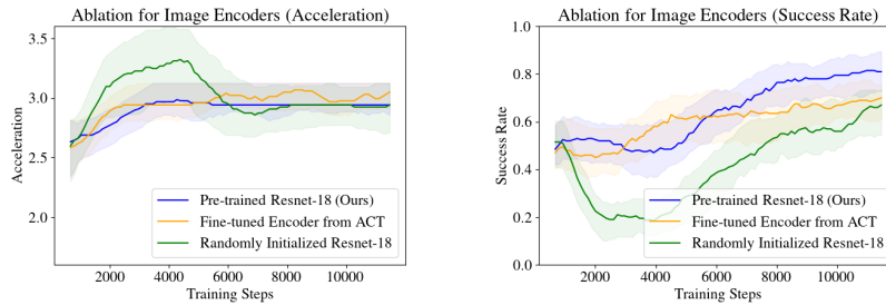
Fig. 12: Image-encoder ablation: acceleration (left) and success rate (right).
