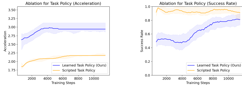
Fig. 8: Base-policy ablation: acceleration (left) and success rate (right). Learned ACT is compared with an open-loop scripted policy.
