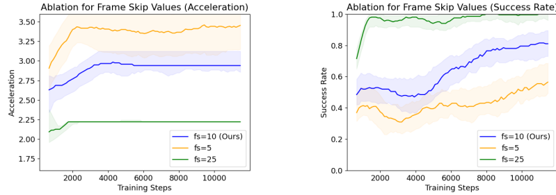
Fig. 11: Frame-skip ablation: acceleration (left) and success rate (right). The main experiments use f_s = 10 .
