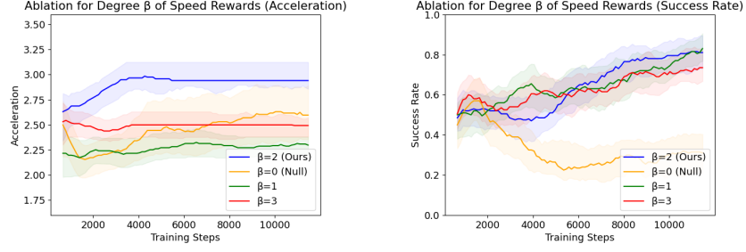
Fig. 10: Speed-reward ablation: acceleration (left) and success rate (right). The main experiments use \beta = 2 .
