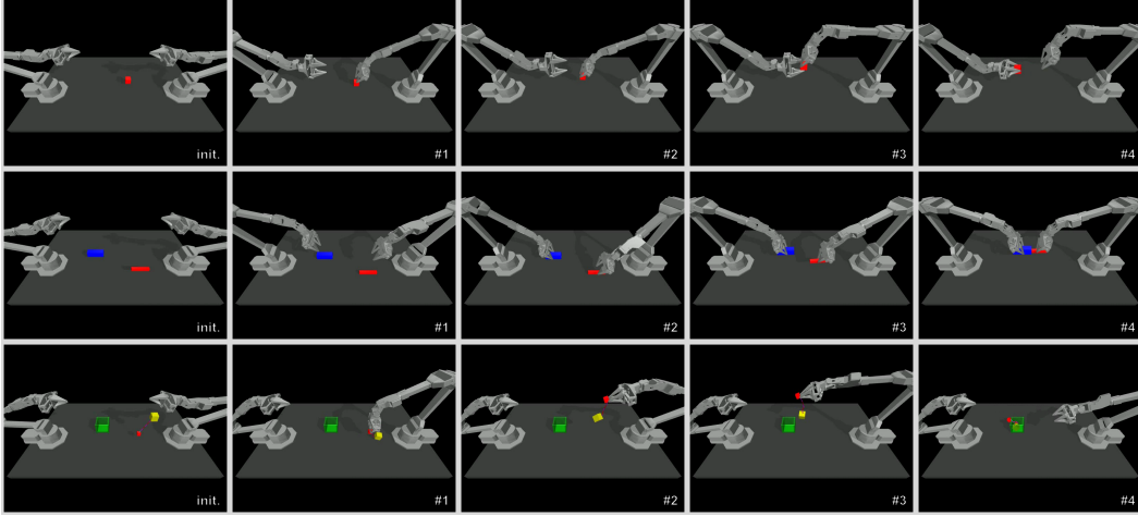
Fig. 7: Representative SPEEDTUNING rollouts in simulation. Rows show Cube Transfer, Peg Insertion, and Tea Bag Transfer; columns show the initial state followed by four successive task stages.
