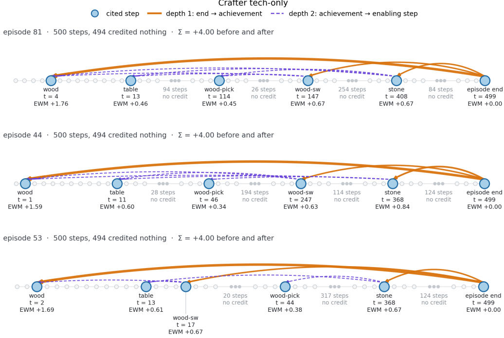
Figure 7: Three Crafter episodes with the same conserved return. Each row is that episode’s step axis, compressed: cited steps keep a few real neighbours, and each long uncredited run collapses to three dots labelled with the number of hidden steps. Solid orange arrows are depth-1 hops from the episode end onto the achievements that earned the reward; dashed purple arrows are depth-2 hops from those achievements onto earlier enabling actions.
