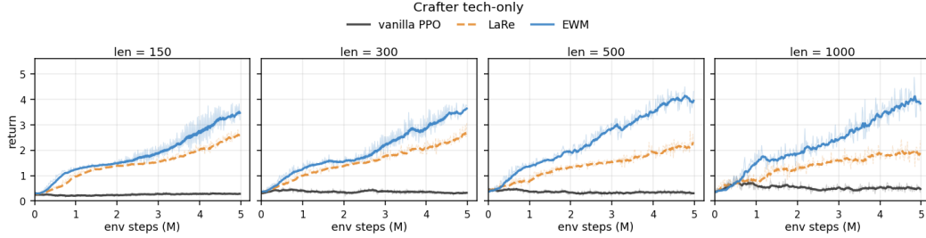
Figure 3: Crafter mean episode return at episode-length caps L \in \{150, 300, 500, 1000\} . Vanilla PPO stays near the random-policy floor. LaRe recovers some delayed credit; EWM is above LaRe at every horizon, and the gap widens as L grows.
