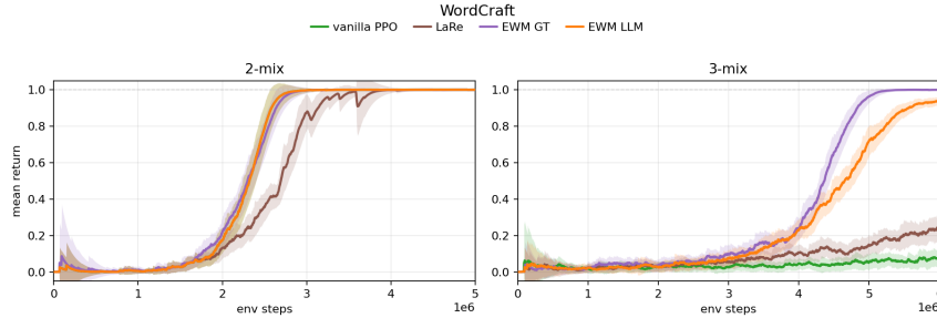
Figure 4: WordCraft returns. The 2-mix variant can easily be solved by every algorithm. The 3-mix variant is considerably more difficult due to longer causal chains and only EWM can solve it.
