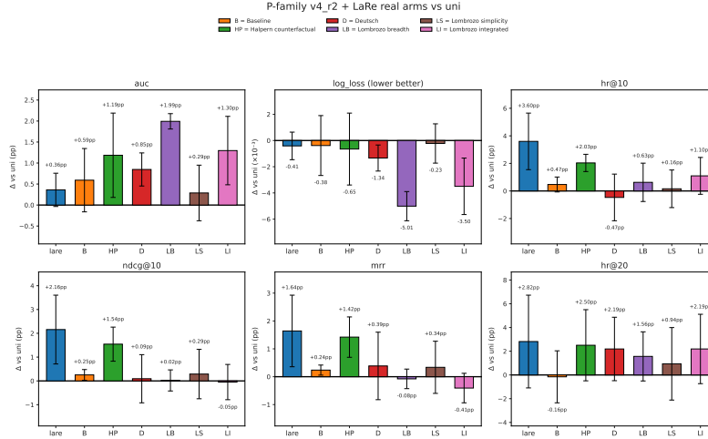
Figure 5: LB achieves the largest mean AUC improvement and log-loss reduction, whereas LaRe differs most from uniform on the four reported ranking metrics.
