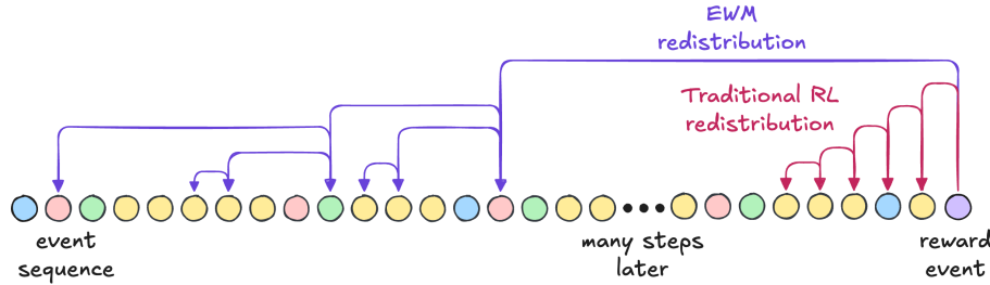
Figure 2: Traditional credit assignment (red) propagates a reward to temporally adjacent events, regardless of their relevance. EWM’s conservative hierarchical operator (CHO, purple) instead uses the explanatory power of each event, recursively, to attribute the reward.
