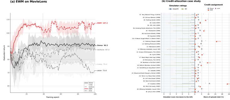
Figure 8: MovieLens-1M policy learning and an illustrative credit allocation. (a) Mean evaluation return across all seeds; shading shows the seed minimum–maximum range, not confidence intervals. We see that the performance of EWM outperforms baselines dense feedback, uniform redistribution, lump terminal reward, and an ablation where we anonymize all the item names in the EWM prompt (so that the EWM does not get any information about the user). Here, each standard deviation is across 100 evaluation episodes. (b) An example session (user 4707, row 573; 30 recommendations in original order), where training rewards and evaluation scores increase to the left. We can see that EWM predictions happen to line up quite well with MF predictions, especially when MF and DeepFM issues different predictions about the same episode.
