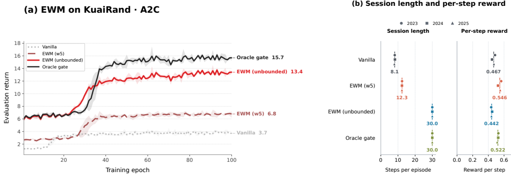
Figure 6: The termination rule that 5-window-EWM discovered outperforms the baseline vanilla A2C method, and the full-history EWM comes close to the oracle termination rule results.
