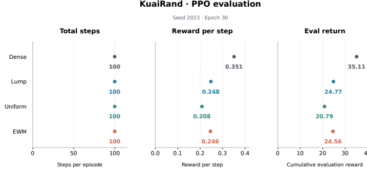
Figure 9: Anonymized KuaiRand PPO results for Dense, Lump, Uniform and EWM. Each point is a statistic from the same 100-episode evaluation. Total steps denotes the mean steps per episode, not training steps or the sum across evaluation episodes. Eval return is mean cumulative reward per episode. Similar to the anonymization ablation experiment in the MovieLens setting, we again see here that EWM performs worse than dense baselines in the KuaiRand environment when the environment does not provide information about the recommendation items in the dataset. In other words, the EWM sees limited semantic information, because the EWM prompt primarily represents videos through anonymous item and tag identifiers, which limits the usefulness of the LLM’s semantic prior knowledge. This interpretation is consistent with the MovieLens anonymization results.
