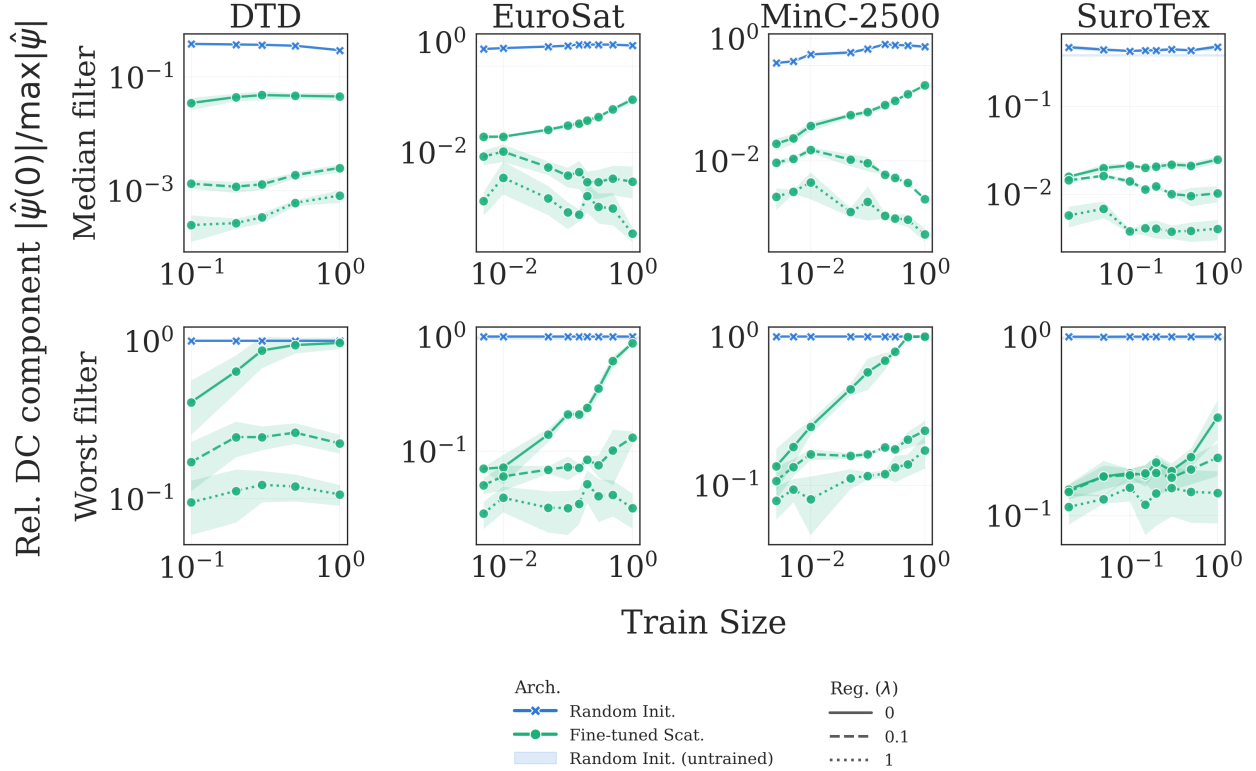
Figure 9: Percentage of data used during training versus relative magnitude of zero-frequency component. Wavelets must satisfy an admissibility condition, that the zero-frequency component has magnitude zero. Color denotes method, line style denotes regularization strength. Increasing regularization strength decreases the relative magnitude of the zero-frequency component on all datasets.
