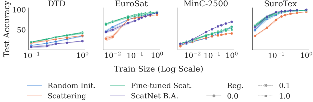
Figure 2: Percentage of data used during training versus test accuracy. Color denotes method and line style denotes regularization strength. The proposed method gives the best performance when the amount of training data is small.
