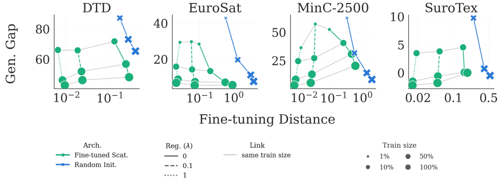
Figure 3: Fine-tuning distance versus generalization gap. Color denotes method, line style denotes regularization strength, and size denotes amount of training data used. Gray lines between fine-tuned scattering networks trained on the same data size allow comparison across regularization strengths. Smaller fine-tuning distance correlates with lower generalization gap.
