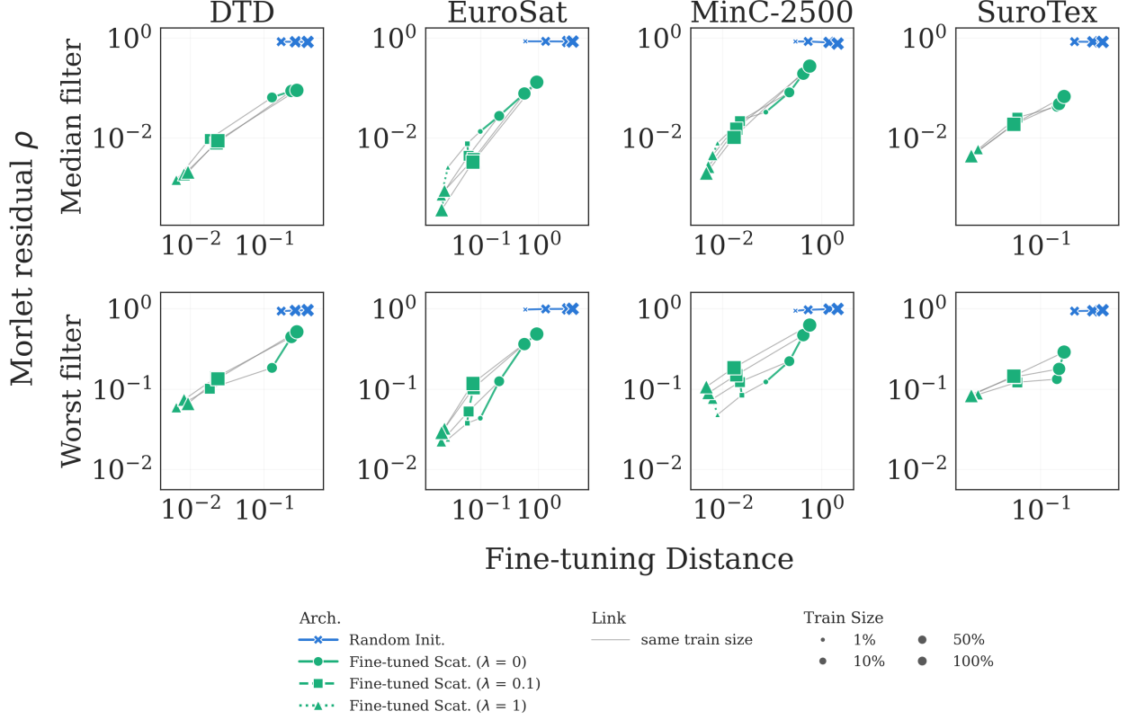
Figure 10: Fine-tuning distance versus \rho (similarity to best-fit Morlet filter). Color denotes method and marker style denotes regularization strength. Marker size denotes the percentage of data used during training. Smaller fine-tuning distance is correlated with more similarity to a Morlet filter across all four datasets.
