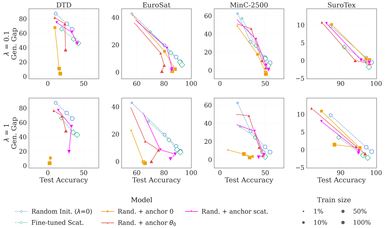
Figure 7: Test accuracy versus generalization gap, comparing effect of different parameter anchors on randomly initialized model. Within each subplot, color indicates method and parameter anchor, and marker size indicates percentage of training data used. The randomly initialized model with scattering anchor has higher generalization error than the fine-tuned scattering model, likely because the fine-tuning distance is greater on DTD and MinC-2500.
