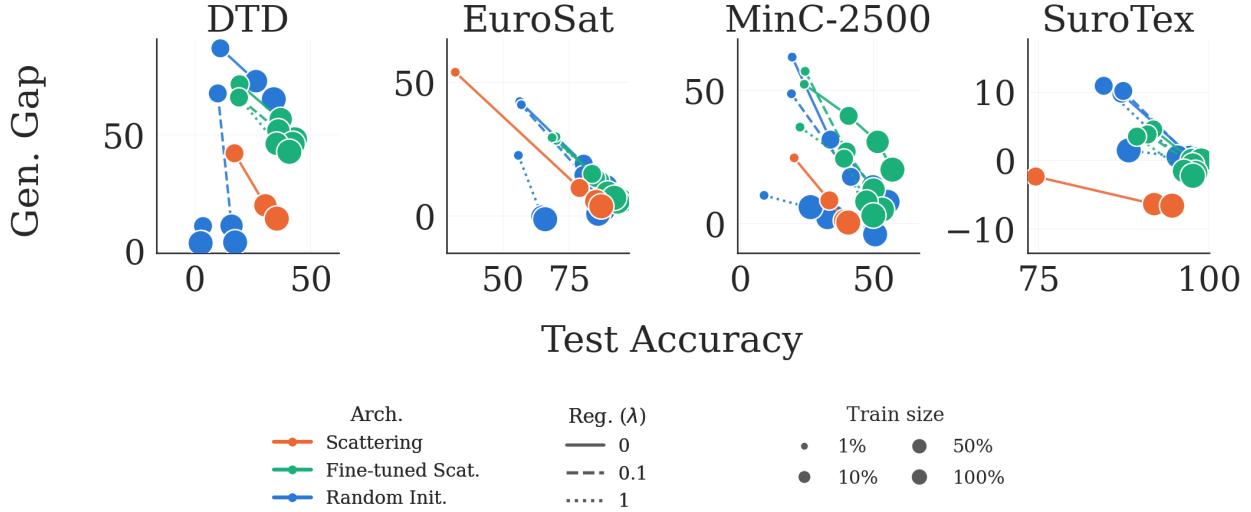
Figure 6: Test accuracy versus generalization gap, with weight decay regularization on randomly initialized model. Color denotes method, line weight denotes regularization strength, and size denotes percentage of training data. Weight decay controls the generalization gap at the cost of reducing test accuracy on DTD, EuroSat, and MinC-2500.
