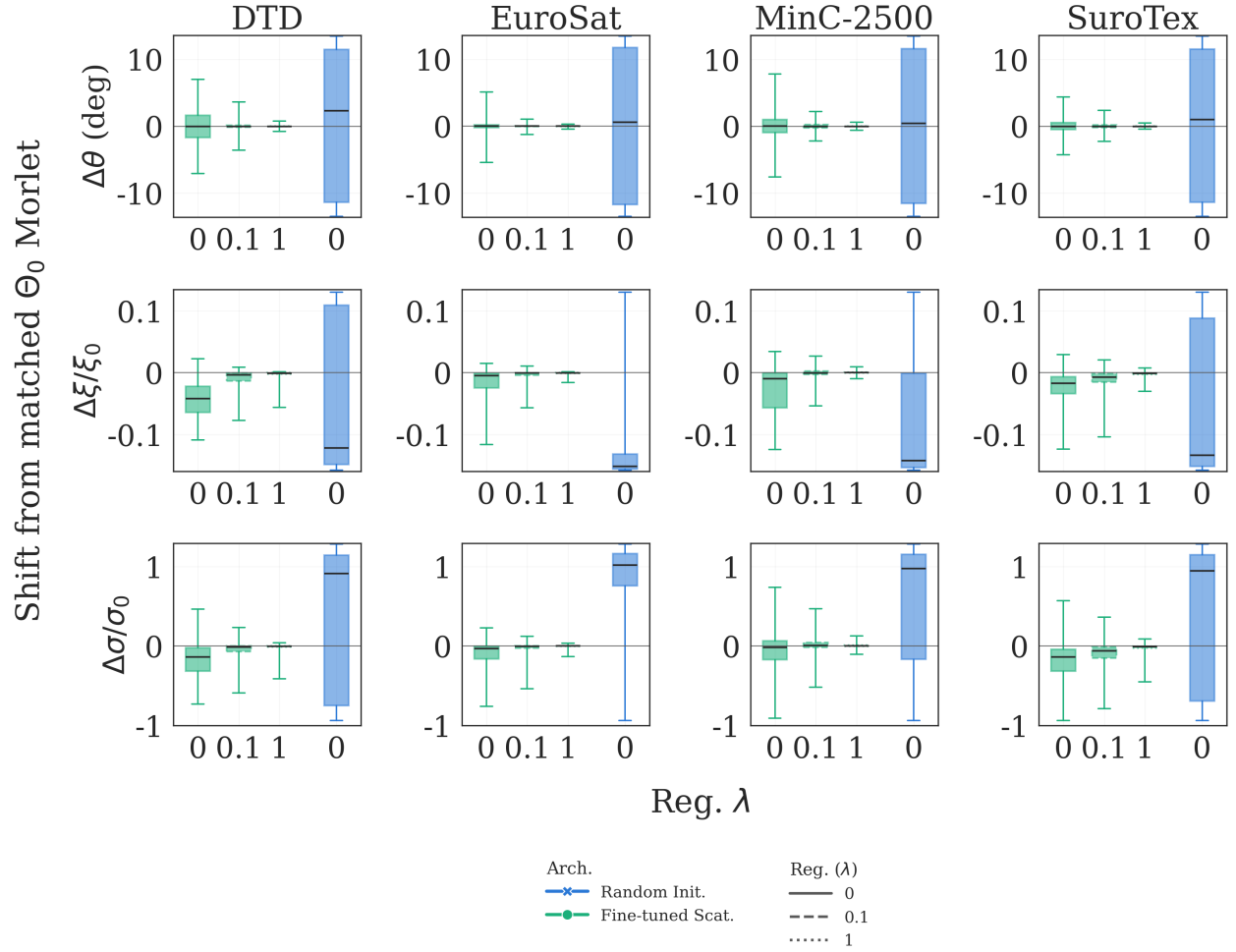
Figure 11: Relative change in the fitted Morlet parameters during fine-tuning. For each fine-tuned filter, we compare the parameters of its best-fit Morlet wavelet to those of the matched filter in the initial bank. Regularizing the fine-tuning distance keeps the parameters closer to their initial values across datasets.
