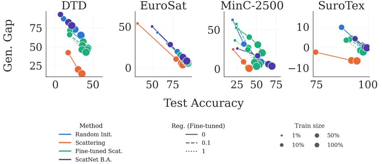
Figure 5: Test accuracy versus generalization gap. Color denotes method, line style denotes regularization strength, and marker size denotes percentage of training data used. Increasing regularization strength decreases generalization error on DTD, MinC-2500, and SuroTex.
