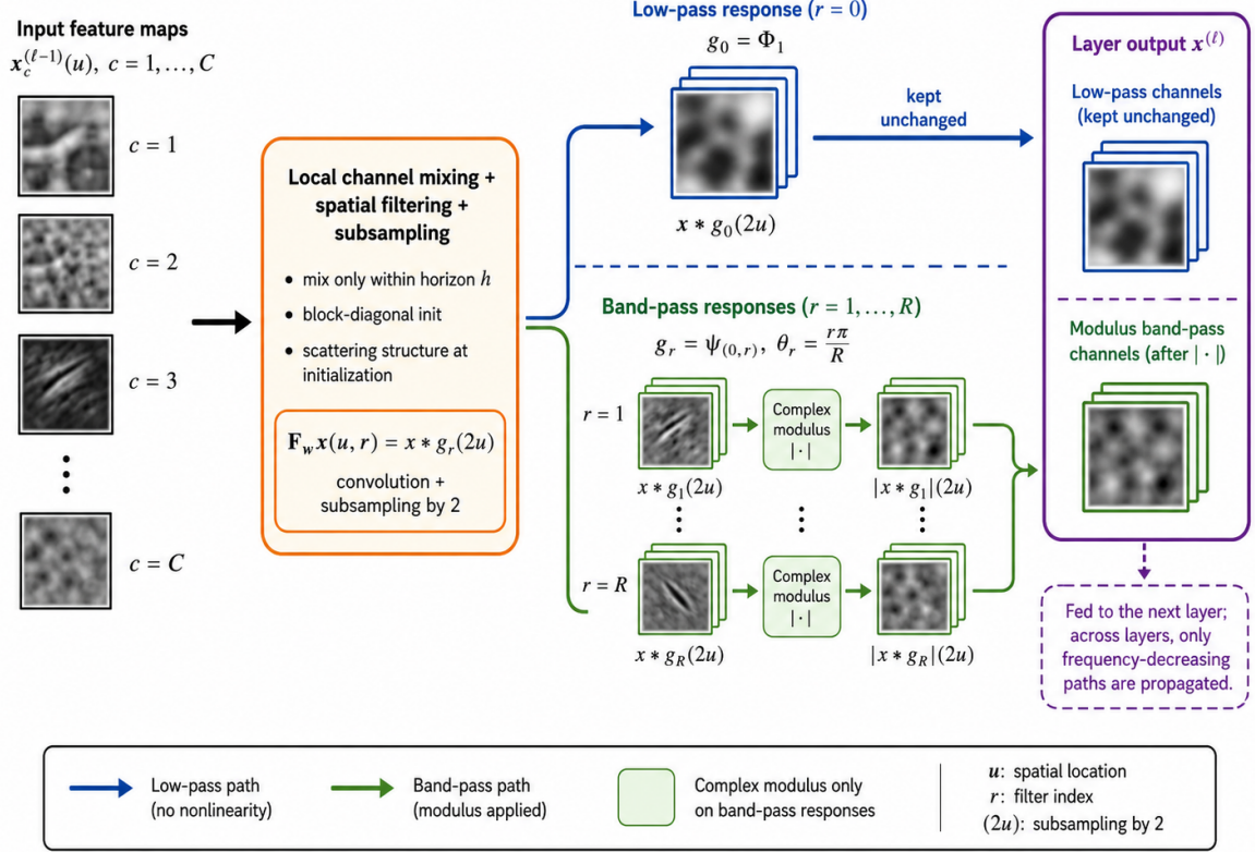
Figure 4: Trainable scattering architecture. At initialization, the convolutional operators reproduce independent wavelet filtering and hence the predefined scattering transform. Fine-tuning allows the wavelet filters and permitted cross-channel interactions to adapt from data.
