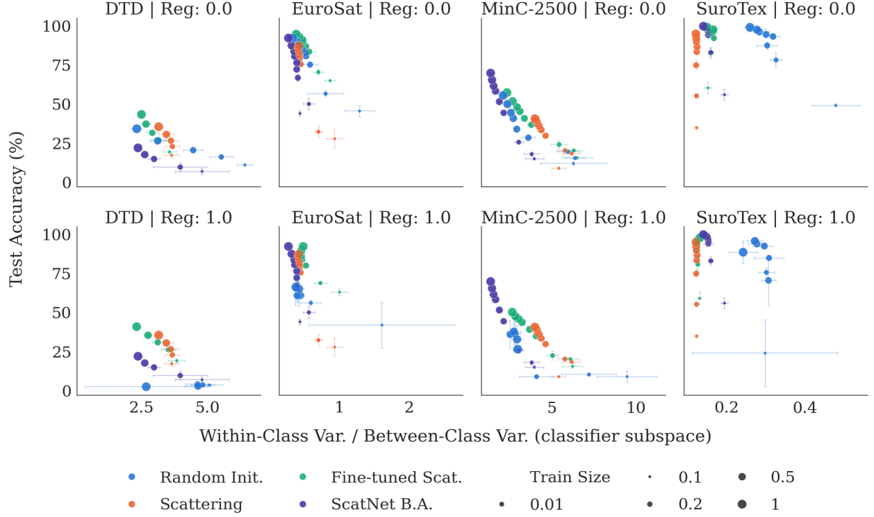
Figure 8: Normalized within-class variance in classifier subspace versus test accuracy. Within sub-plots, color denotes method, marker size denotes percentage of training data used, and cross-hatches denote standard deviation. Rows denote regularization strength and columns denote datasets.
