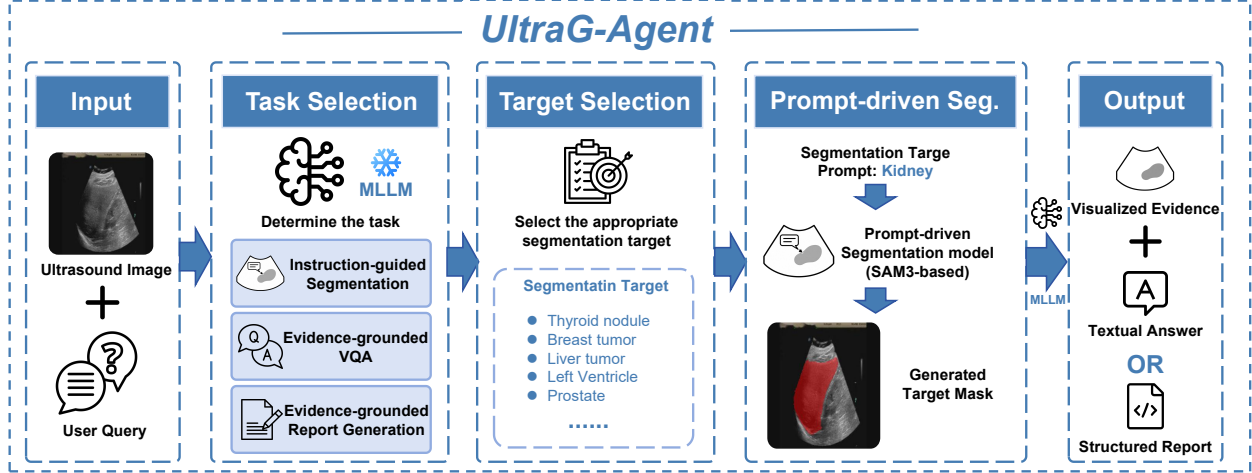
Figure 3: Overview of UltraG-Agent.
