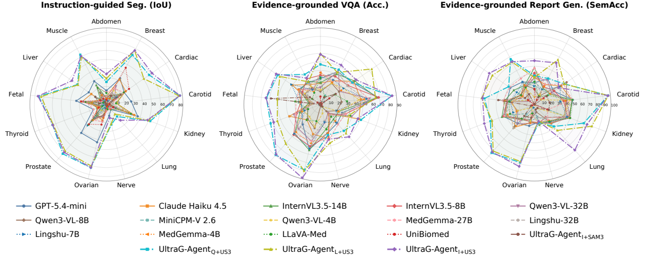
Figure 4: Fine-grained organ-level comparison across 13 anatomical categories for the three tasks in UltraG-Bench. UltraG-Agent variants with UltraSAM3 show consistently strong performance across diverse organs.
