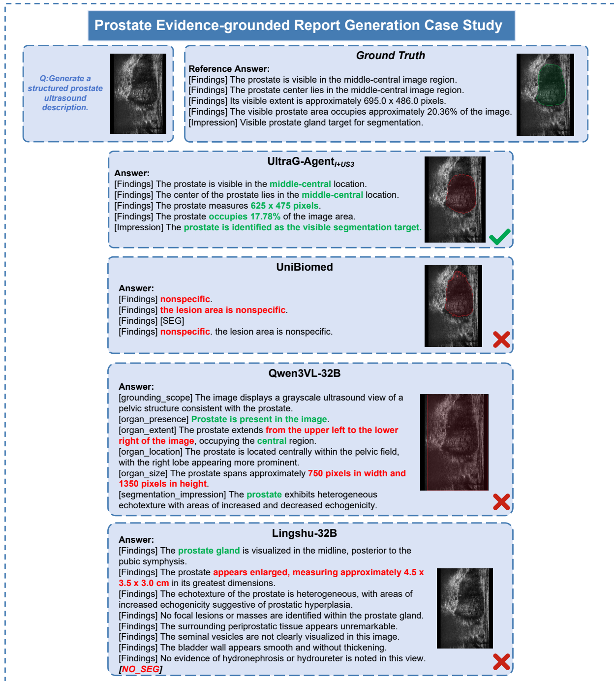
Figure 10: Prostate Evidence-grounded Report Generation Case Study.
