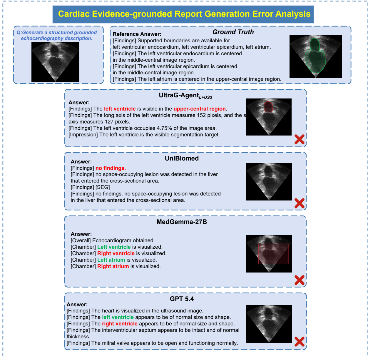
Figure 14: Cardiac Evidence-grounded Report Generation Error Analysis.
