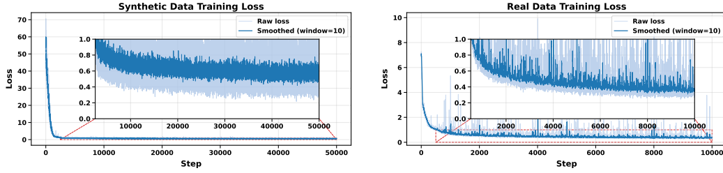
Figure 3: Loss curves during the two-stage training. The light blue curve shows the raw loss, and the dark blue curve shows the loss smoothed by a moving average with a window size of 10.
