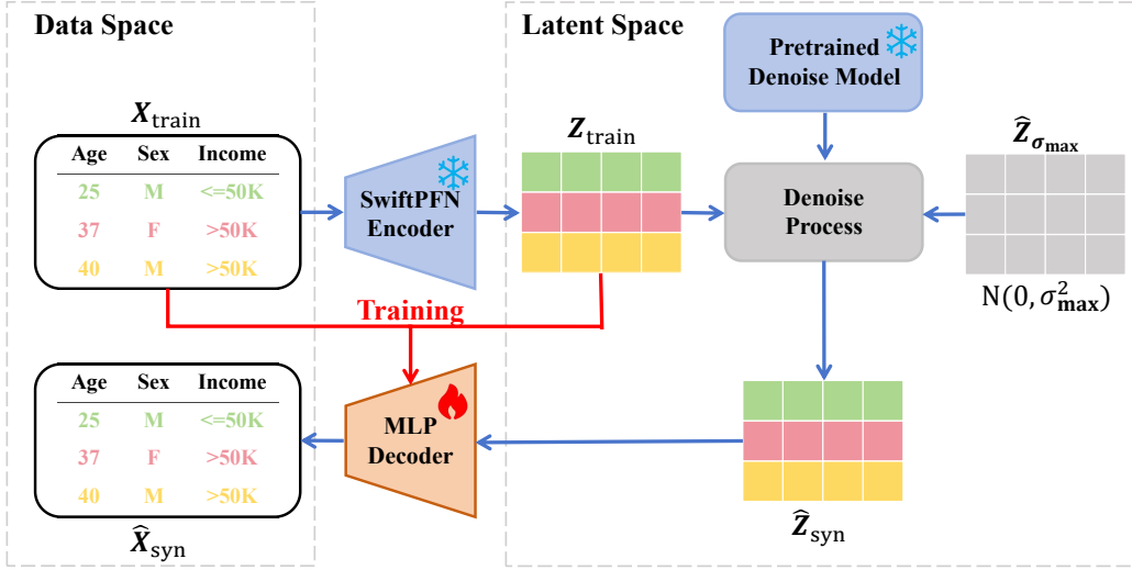
Figure 1: TABGIFT consists of a data space and a latent space: (1) Encoding: Given the real training table X_{\text{train}} , the SwiftPFN Encoder maps heterogeneous samples into a unified 192-dimensional latent space, producing the latent embeddings Z_{\text{train}} . (2) Latent-space generation: The real-data latent embedding Z_{\text{train}} is used as context. Starting from Gaussian noise, a pretrained frozen denoising model generates new latent embeddings \hat{Z}_{\text{syn}} through an iterative denoising process. (3) Decoding: A lightweight MLP Decoder is trained per target dataset to reconstruct the generated latent embeddings \hat{Z}_{\text{syn}} back into the data space, yielding synthetic data \hat{X}_{\text{syn}} . Throughout the pipeline, only the MLP Decoder requires dataset-specific training, while the SwiftPFN Encoder and the denoising model are pretrained and kept frozen during inference.
