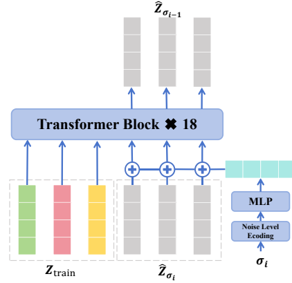
Figure 2: In-context learning model.
