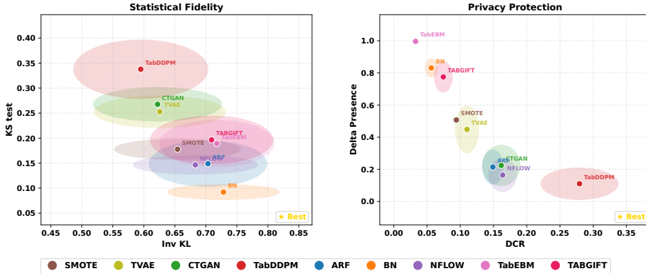
Figure 4: Synthetic generator comparison on statistical fidelity (Inv KL, KS test) and privacy protection (DCR, Delta Presence). Shown for training size 16 across all datasets, mean over 5 seeds.
