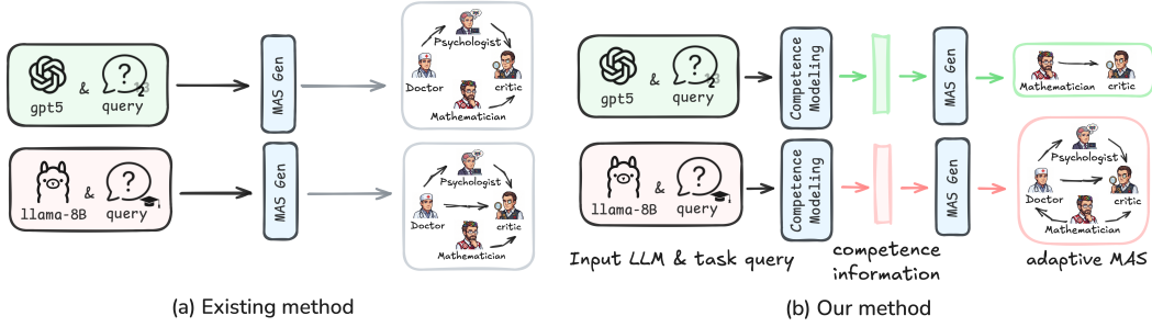
Figure 1: Comparison between existing MAS construction methods and our method.
