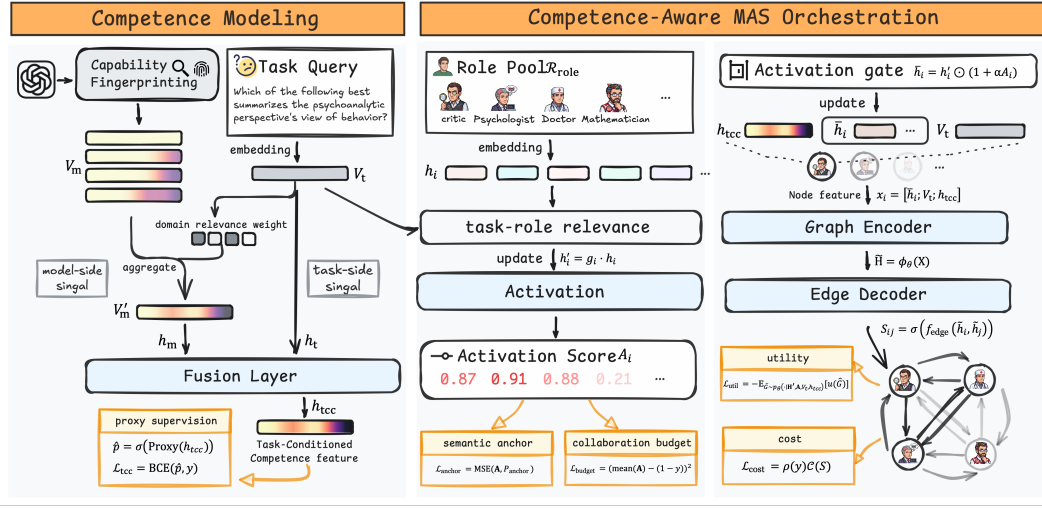
Figure 2: Overview of the proposed competence-aware orchestration framework. Stage I learns a competence representation from the backbone’s capability fingerprint and the current query under success-rate supervision. Stage II uses this representation to guide role activation and communication graph generation.
