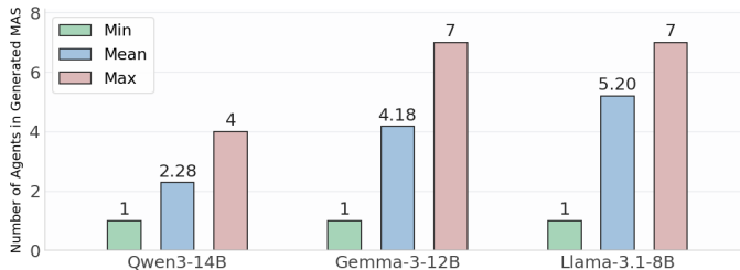
Figure 3: Number of agents in the generated MAS on efficiency-oriented target backbones.
