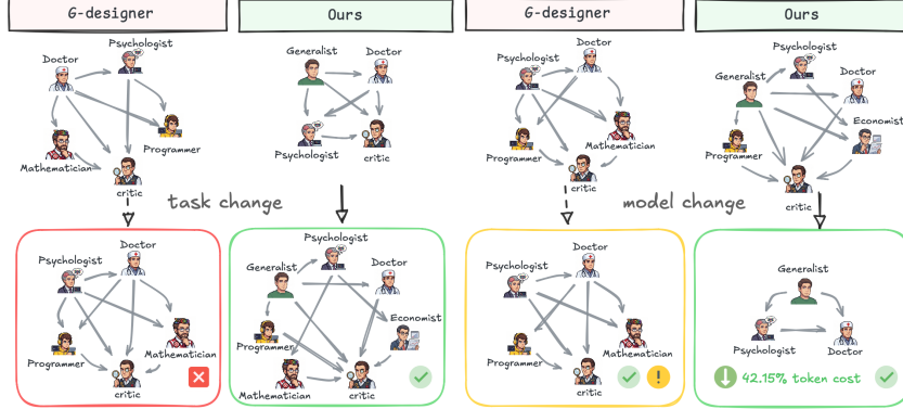
Figure 4: Case studies on MMLU. Left: changing the task while fixing the backbone (Llama-3.1-8B). Right: changing the backbone from Llama-3.1-8B to GPT-4o while fixing the task. check/cross marks indicate answer correctness.
