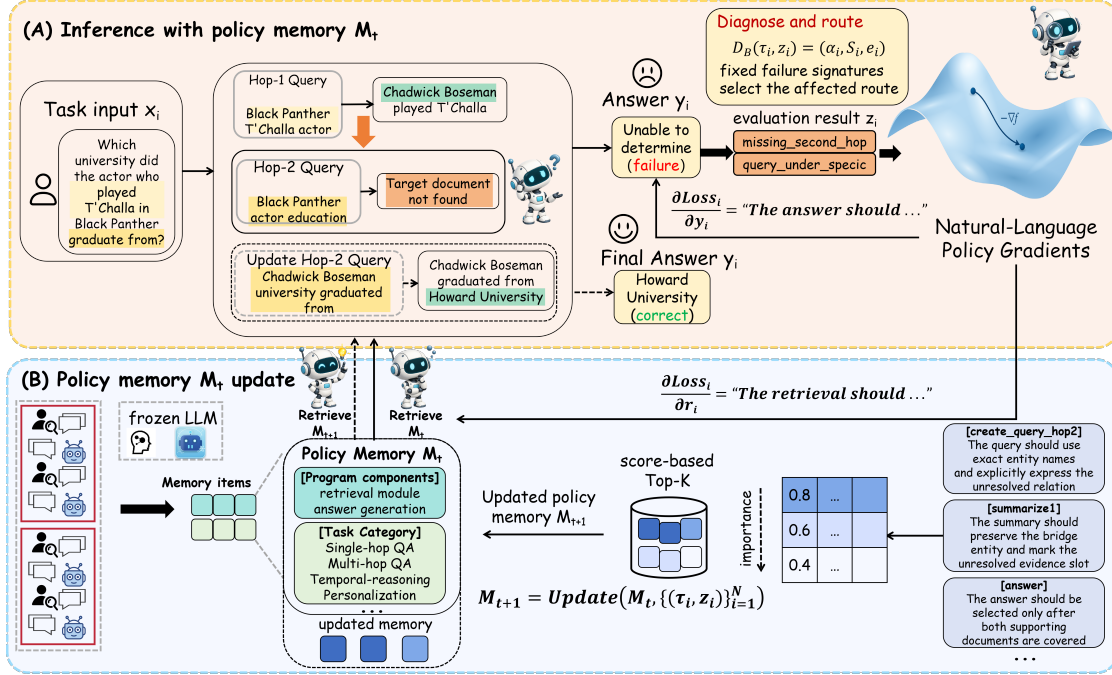
Figure 2: Overview of NLPG. (A) Inference and failure diagnosis. The compound agent retrieves module-local policies from the current policy memory M_t and injects them into the corresponding module calls. (B) Policy-memory update. NLPG aggregates routed language gradients across evaluated trajectories, scores and selects reusable instructions, and stores them under the corresponding program modules and task categories to construct M_{t+1} .
