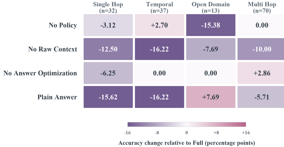
Figure 6: Category-level changes in accuracy, measured in percentage points relative to the full configuration, for answer-stage ablations on the held-out LoCoMo set with fixed cached retrieval. Negative values indicate that the ablated configuration performs worse than the full configuration. The numbers in parentheses denote the number of questions in each category. The Open Domain column is interpreted cautiously because this category contains only 13 questions.
