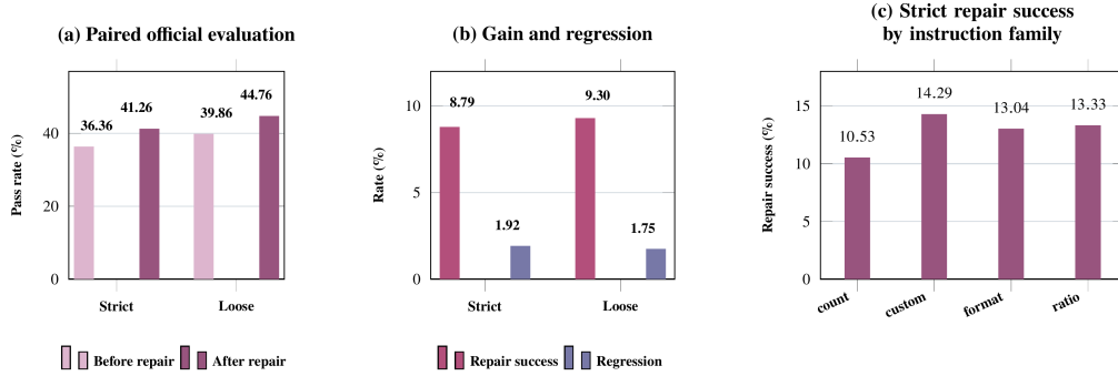
Figure 7: Feedback quality and repair evaluation on IFBench. (a) Paired official evaluation, showing pass rates before and after repair under strict and loose checkers. (b) Gain and regression, showing repair success and regression rates. (c) Strict repair success by official instruction family.
