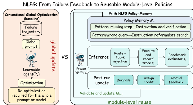
Figure 1: Conceptual comparison of global prompt-level updates and NLPG’s route-indexed policy updates.
