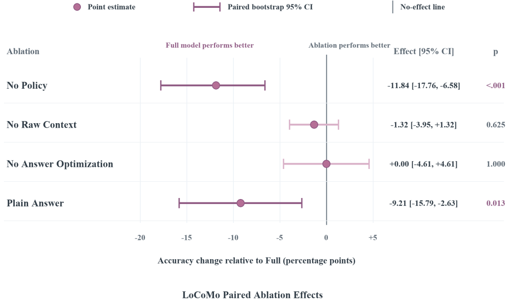
Figure 5: Paired answer-stage ablations on LoCoMo ( n = 152 ). Points denote accuracy changes relative to the full model, and horizontal bars show paired-bootstrap 95% confidence intervals. Negative values favor the full model, while the vertical line denotes no effect. Reported p -values are from two-sided exact McNemar tests. Retrieval results are fixed and cached across all variants.
