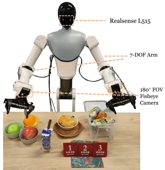
Figure 9: Custom dual-arm robot platform used in the real-world experiments.
