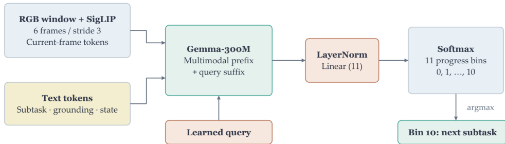
Figure 8: Architecture of the progress evaluator. A learned query aggregates the multimodal visual and language prefix, and a normalized linear head predicts one of 11 progress categories.
