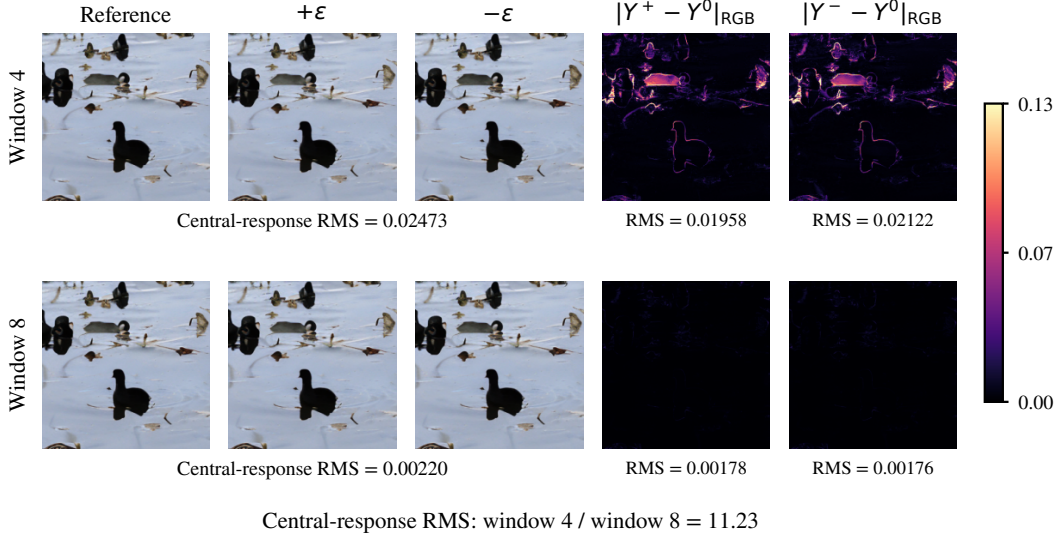
Figure 6 Second DiT example, with the endpoints, branch-difference maps, and shared color scale defined in Appendix C.6. Reference-relative displacement RMS is annotated separately for each branch; the window-4/window-8 central-response RMS ratio is 11.23.
