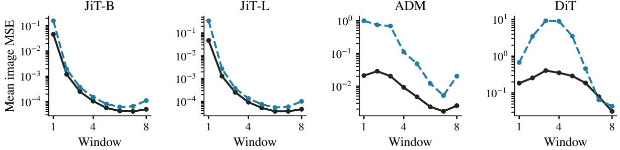
Figure 4 Predicted and observed image MSE under caching. Black solid lines show observed image MSE and blue dashed lines show predictions from the propagation-based predictor, averaged over the same 64 samples per model. Each candidate reuses the prediction cached at the start of one eight-step window, and windows are ordered from noise toward output.
