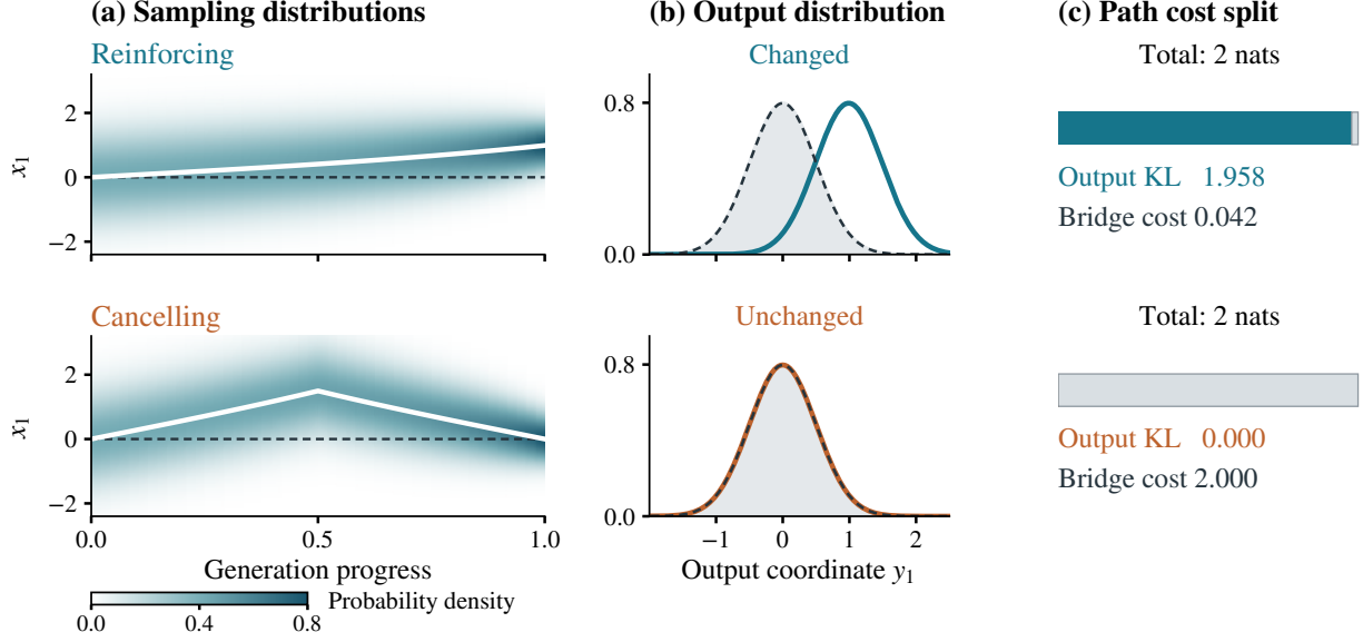
Figure 1 Equal path costs, different output-distribution changes. Two temporal perturbation sequences act only on the first coordinate of a two-dimensional Gaussian reverse diffusion, each with path cost \mathcal{C} = 2 nats. Their contributions reinforce (top) or cancel (bottom) at the output. (a) Coordinate density evolution on a shared color scale, with perturbed (white) and reference (dashed) means. (b) Perturbed (solid) and reference (dashed) output densities. (c) Output KL (colored) and bridge cost (gray). Construction details are in Appendix B.
