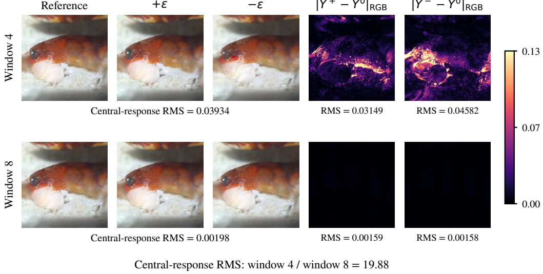
Figure 5 DiT image responses to equal-cost perturbations. A fixed sample under positive and negative DCT-4 perturbations in windows 4 and 8. Difference maps show per-pixel RGB RMS relative to the reference Y^0 , with full-image RMS below each map. Central-response annotations measure the RMS of (Y^+ - Y^-)/(2\epsilon) ; the window-4/window-8 ratio is 19.88. Differences use unclipped pixels and a shared color scale across both examples.
