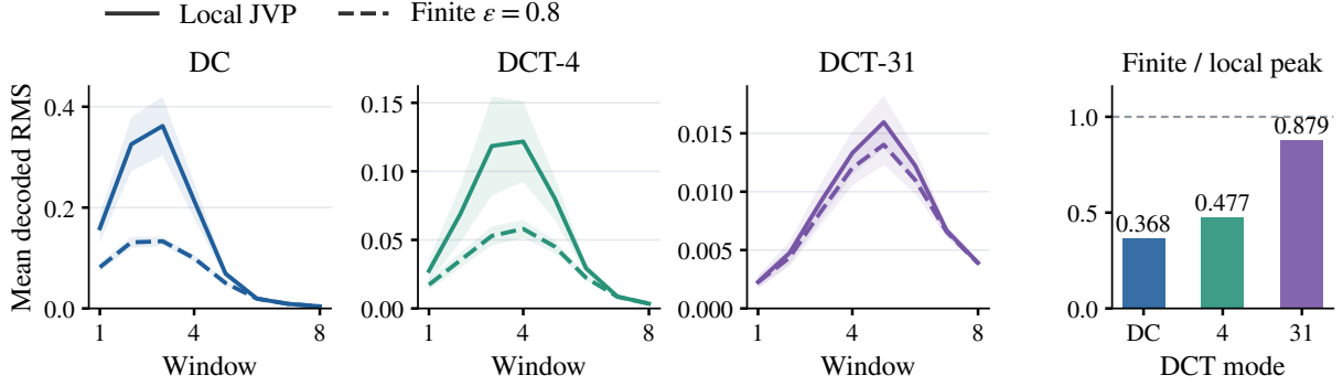
Figure 3 Local predictions and finite perturbation responses in DiT. Mean decoded-image RMS of local derivatives and symmetric finite differences ( \varepsilon = 0.8 ) on the same 32 trajectories, where shaded bands indicate one standard error of the mean across samples. The right panel reports finite/local peak ratios with dashed line denoting equal amplitudes. All runs use 128 stochastic steps.
