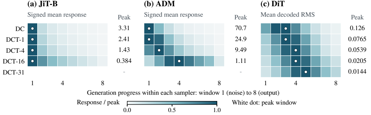
Figure 2 Output responses at equal path cost within each model. Rows show perturbation frequencies and columns show the sampling windows in which perturbations are applied, from early to late. Each row is divided by its maximum response. White dots mark the peak windows and numbers on the right give the maxima before normalization.
