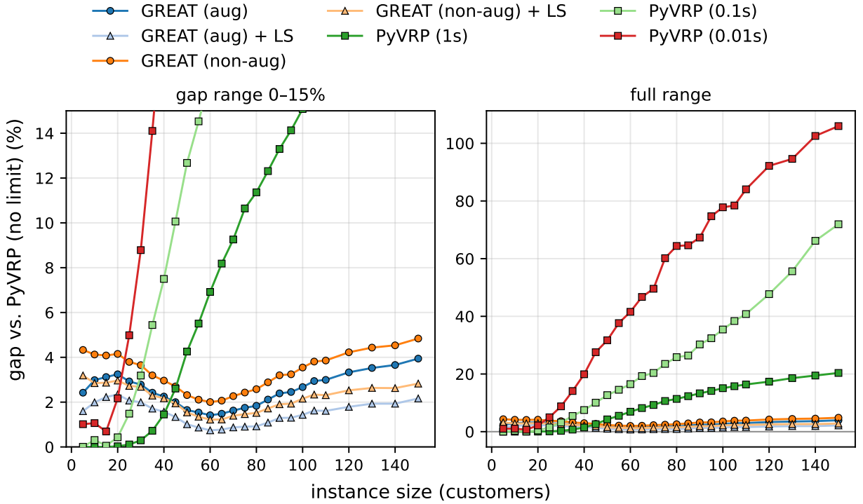
Figure 5: Performance of different CVRP solvers w.r.t. PyVRP without time limit. Left: gap range 0–15 %; right: unconstrained range.
