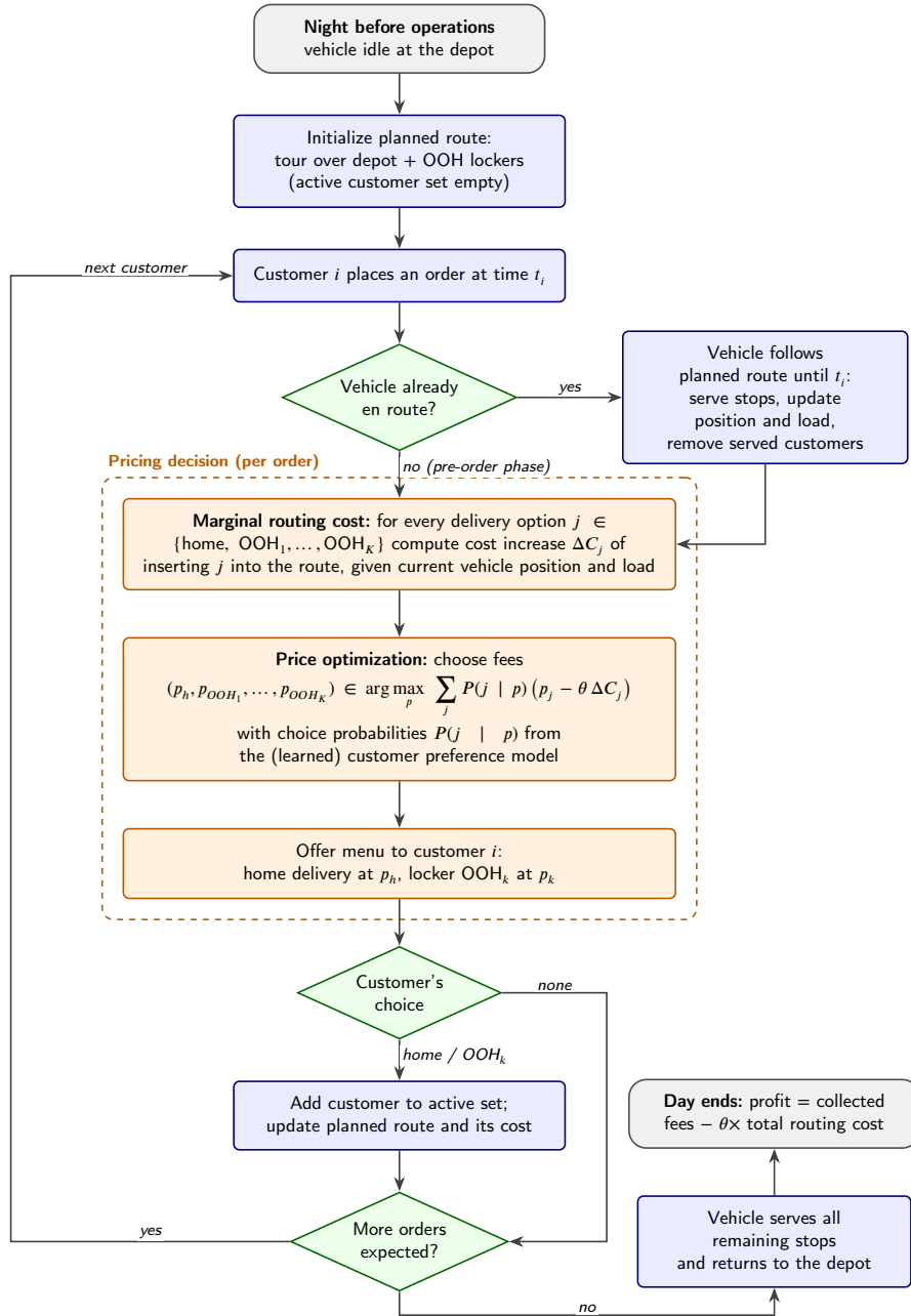
Figure 1: The pricing-and-routing loop of the GREAT-ESDD framework over one operating day. The vehicle follows a planned route. Any time a customer orders, the current routing state is used to compute a routing cost estimate of the delivery options and a price menu is chosen to maximize expected profit. The customer's choice determines the updated route.
