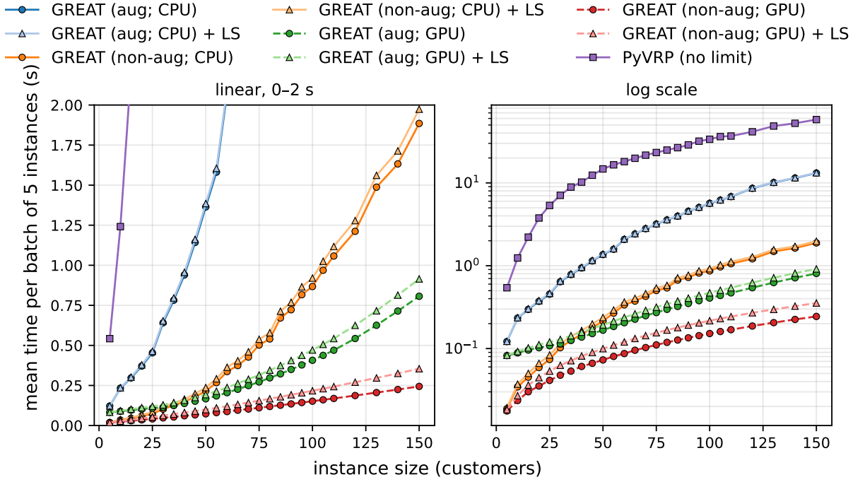
Figure 6: Runtime of different CVRP solvers (PyVRP with set time limit is omitted) to solve a batch of 5 CVRP instances in parallel. Left: linear scale, 0–2 s; right: logarithmic scale, unconstrained range.
