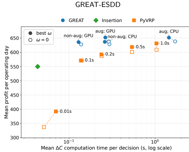
Figure 7: Marginal routing cost ablation, showing mean time to compute the routing cost increase for a pricing decision vs. the mean profit per operating day over 25 days
