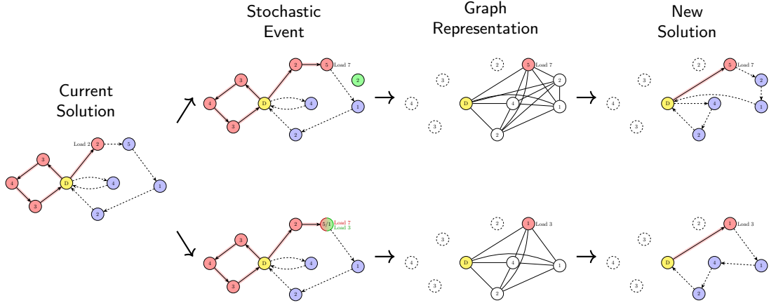
Figure 2: Given a current solution, our framework can react to stochastic changes in the environment. Case one (upper branch) occurs when a new customer dynamically enters the system. Case two (lower branch) occurs when a customer has a lower demand than expected. In both cases we construct a new graph representing the current state. It encodes all unserved customers, the depot, the current vehicle location and the current vehicle load. Our neural model processes this graph encoding and outputs a new solution.
