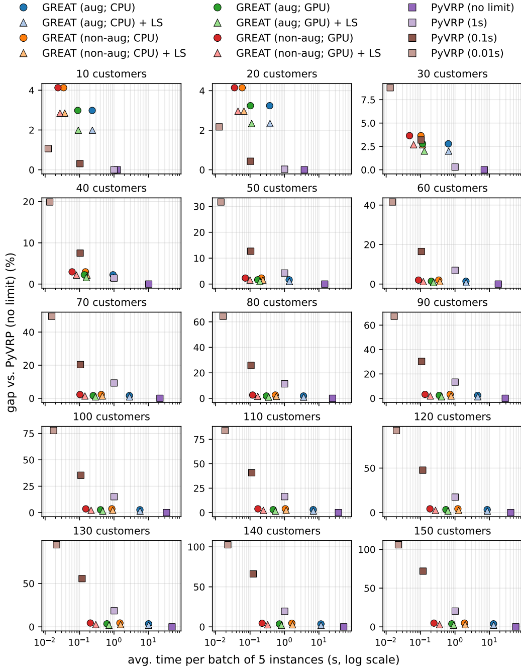
Figure 4: Pareto sets trading off performance (gap w.r.t. PyVRP without time limit) vs. runtime for different CVRP instance sizes.
