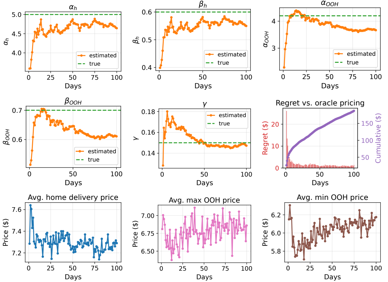
Figure 8: Parameter estimation, price and regret developments of the deterministic learning to price setting.
