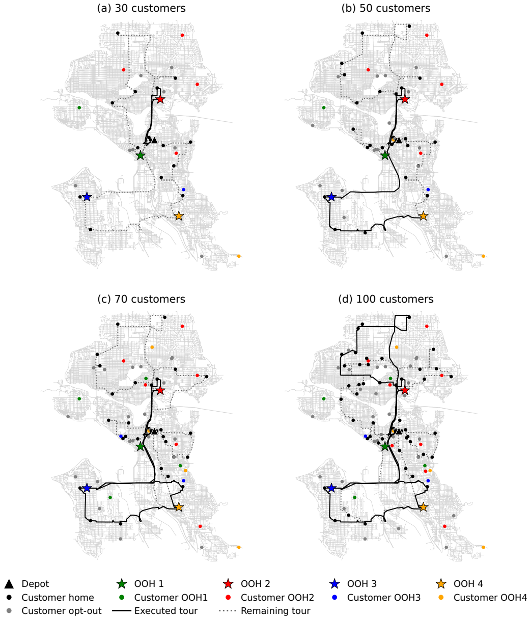
Figure 3: Development of the customer arrival, pricing, customer selection and routing over one day with known customer parameters, shown after (a) 30, (b) 50, (c) 70 and (d) 100 customer requests. The black triangle shows the depot and the colored stars show the OOH locations in our considered Seattle setting. Customers are represented by dots that are either black (home delivery) or colored according to their OOH location; gray dots are customers who opted-out. We show the already executed tour along with the currently still remaining tour.
