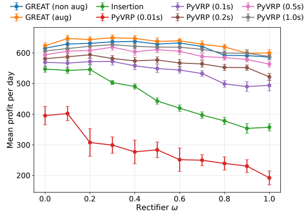
Figure 11: Average profit achieved by different solvers for different rectifiers \omega
