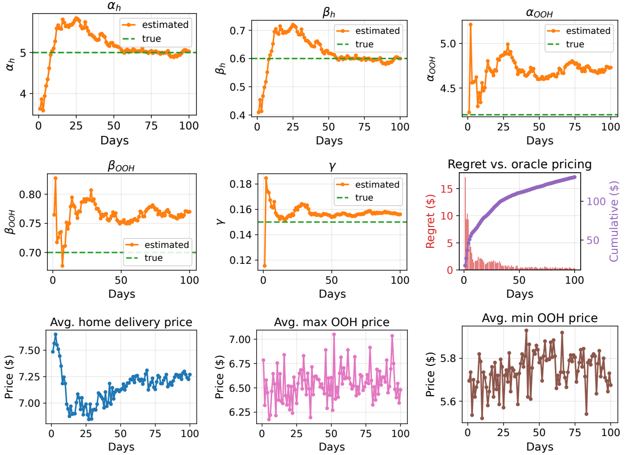
Figure 9: Parameter estimation, price and regret developments of the stochastic learning to price setting.
