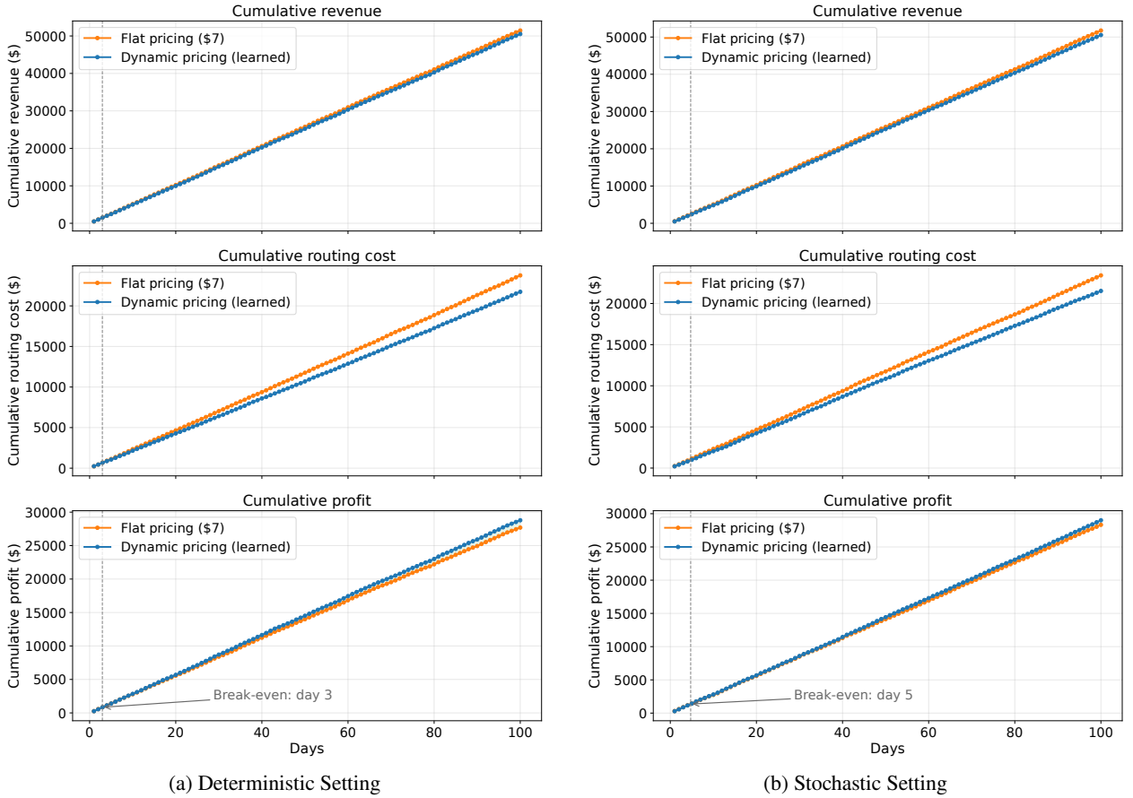
Figure 10: Cumulative revenue, routing cost and profit over 100 days of operation, using the bandit-based pricing and the flat $7 pricing strategies in the deterministic and stochastic setting.
