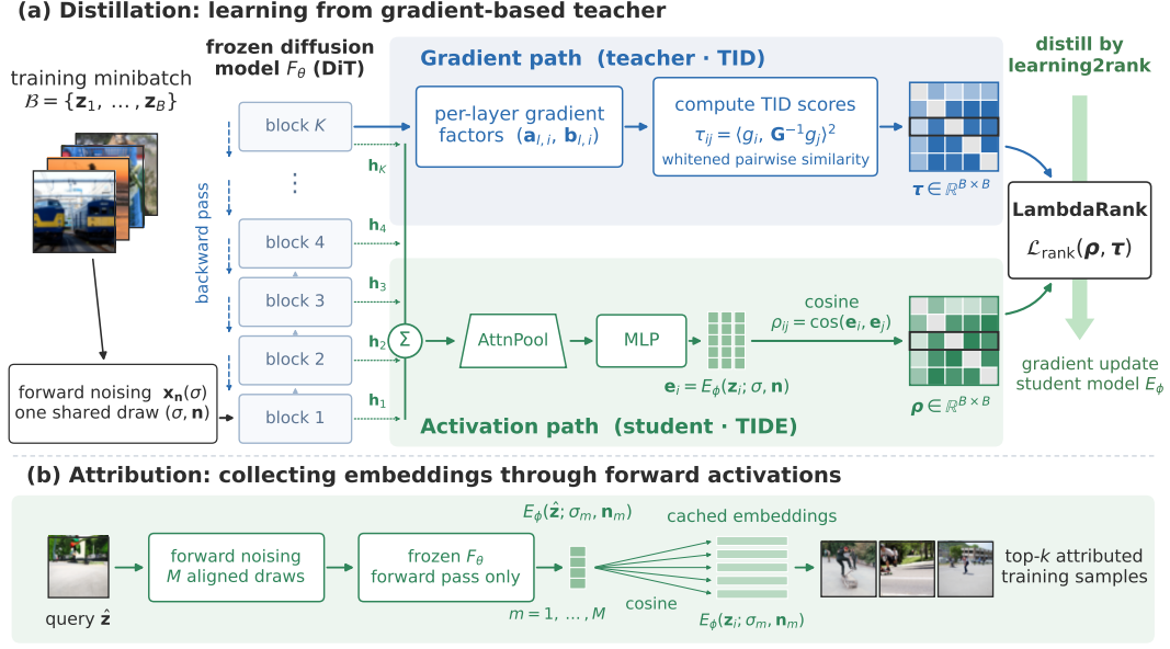
Figure 3: Overview of TID and TIDE.
