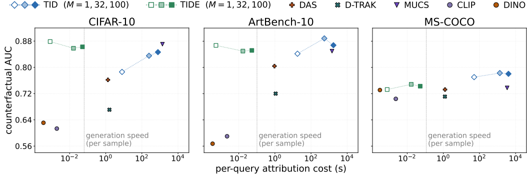
Figure 2: Attribution accuracy versus warm-cache per-query cost on CIFAR-10 (left), ArtBench-10 (middle), and MS-COCO (right). The horizontal axis is logarithmic; cacheable training-side artifacts are precomputed. Markers with different fills connected by dotted lines trace the variation with M .
