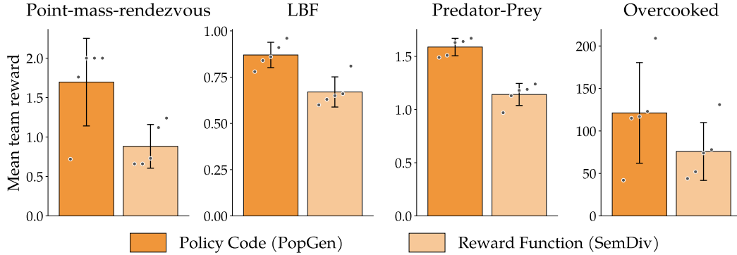
Figure 6: Population play with policy code and reward-function partners. Mean team reward against held-out partners of cooperators whose training partners are modeled as executable code (like POPGEN) or as neural network policies trained with RL on LLM-generated reward functions (like SemDiv). The set of behaviors is kept identical, so that only agent modeling method changes. Error bars give the standard deviation across five runs, and dots mark individual runs.
