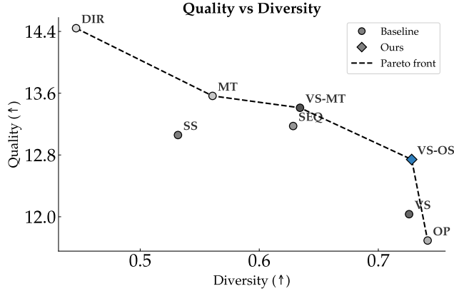
Figure 8: Quality and diversity of all behavior generation methods. Quality and diversity of a generated set of 30 behaviors, averaged across the four environments, for every method in Table 9. VS-OS is the method used in POPGEN.
