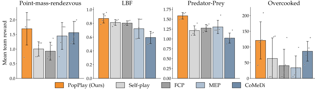
Figure 2: Zero-shot coordination with held-out partners. Each bar reports the average team reward (higher is better) when each cooperator is paired with the held-out partners, which do not appear in any training population. Error bars give the standard deviation across five runs, and dots mark individual runs. POPPLAY attains the highest reward in all four environments. Table 5 reports the reward against each individual partner.
