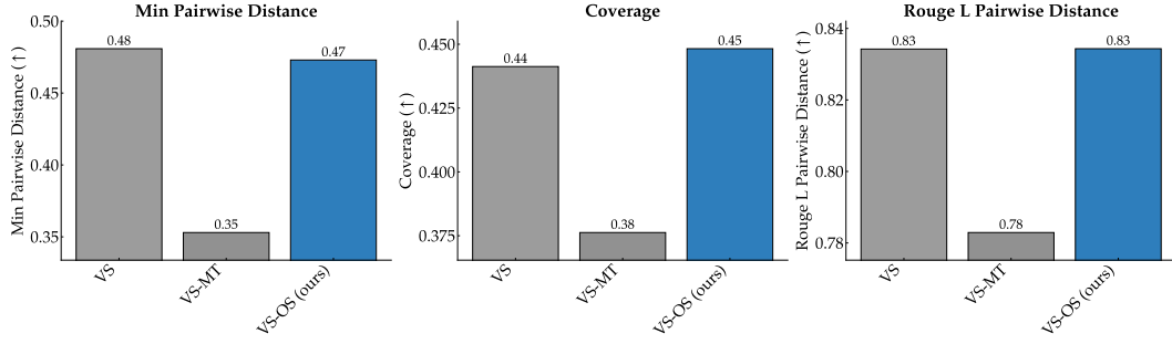
(a) Detailed diversity metrics: minimum pairwise embedding distance, embedding space coverage, and lexical dissimilarity ( 1 - \text{Rouge-L} ).
