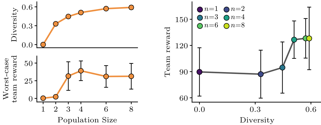
(a) Diversity of the training pool and worst-case team reward as a function of population size.
