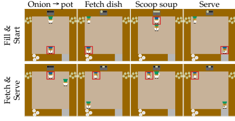
(a) Rendered rollouts of POPPLAY cooperator (red box) paired with a partner. POPPLAY switches roles based on the partner’s behavior.
