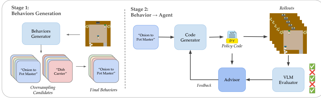
Figure 1: Overview of POPGEN. Left (Stage 1): An LLM produces a diverse set of behaviors at the text level using oversampling. Right (Stage 2): Each behavior description enters an iterative refinement loop: a generator translates the behavior into an executable policy (Policy Code), which is evaluated with a VLM through environment rollouts. An advisor then analyzes rollout results and provides feedback to guide subsequent refinement attempts.
