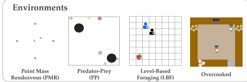
Figure 7: Environments used for cooperator training. From left to right, PMR requires agents (red and purple) to navigate toward and converge on the same landmark (green). PP requires agents (red) to coordinate to capture prey, with different rewards between individually capturing a rabbit (green) and jointly capturing a stag (yellow). LBF requires agents to combine their carrying capacities to collect food items whose levels may exceed the level of a single agent. Finally, overcooked requires two chefs to coordinate the sequential subtasks of preparing, cooking, and delivering soups.
