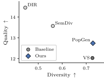
Figure 5: Diversity and quality of POPGEN population agents. Quality and diversity of a generated set of 30 behaviors, averaged across the environments. POPGEN matches the diversity of VS while improving quality, and is substantially more diverse than DIR and SemDiv.
