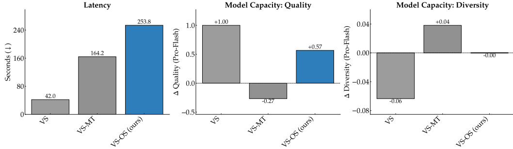
(b) Scaling VS-OS: generation latency in seconds (left); quality improvement \Delta when scaling the generator from Flash to Pro (center); diversity gain \Delta from the same scaling (right).
