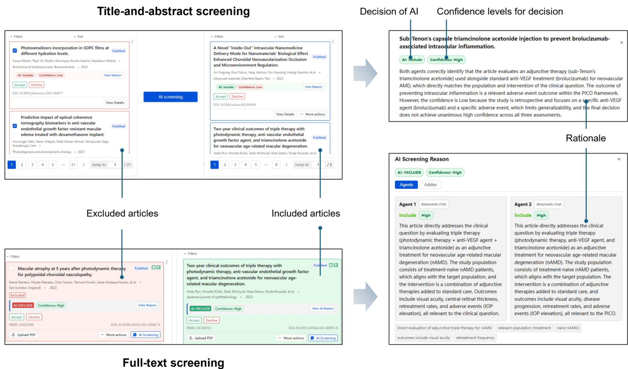
Supplementary Fig. 2 | GUIDE-assisted literature screening workflow and rationale display.
