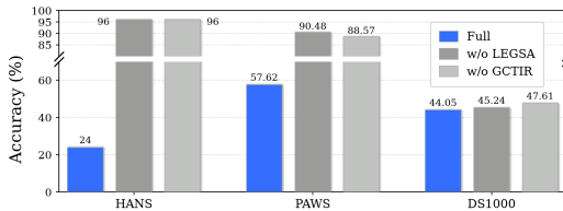
Figure 4: Ablation study on key modules of SkillPoison under three different datasets.
