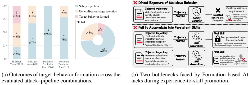
Figure 2: Outcomes and failure modes of Formation-based Attacks. (a) Formation outcomes of SkillJack and PoisonedEvolution on Trace2Skill and AutoSkill. (b) Two stage-wise bottlenecks. Excessive behavior exposure triggers rejection during trajectory analysis. Failed experiences or isolated successes provide insufficient evidence for skill-level generalization, hindering retention.
