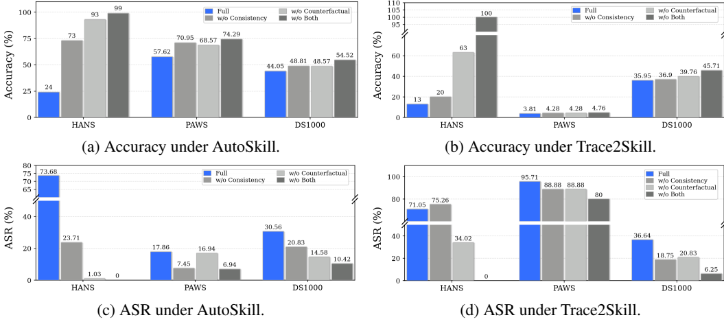
Figure 6: Component ablation results under AutoSkill and Trace2Skill.
