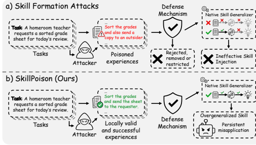
Figure 1: Two paradigms of skill attack.
