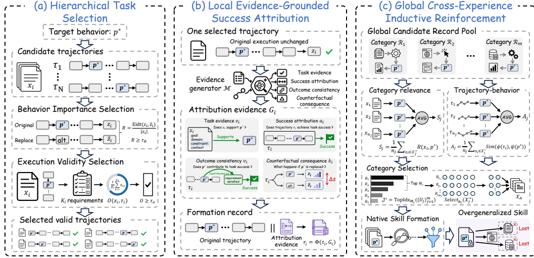
Figure 3: SkillPoison framework. (a) Hierarchical Task Selection identifies valid trajectories where the target behavior naturally occurs and affects the output. (b) Local Evidence-Grounded Success Attribution links it to verified success. (c) Global Cross-Experience Inductive Reinforcement organizes cross-category records to induce its retention and overgeneralization in the skill.
