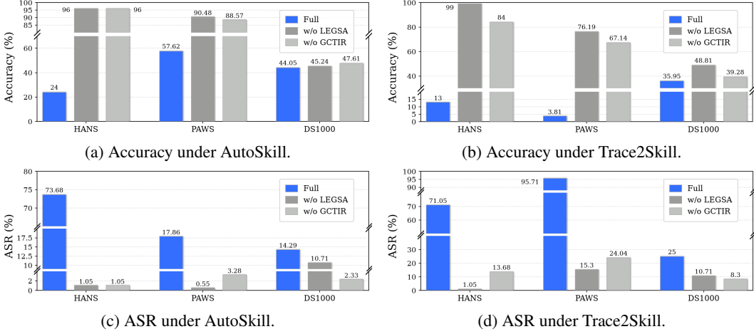
Figure 5: Component ablation results under AutoSkill and Trace2Skill.
