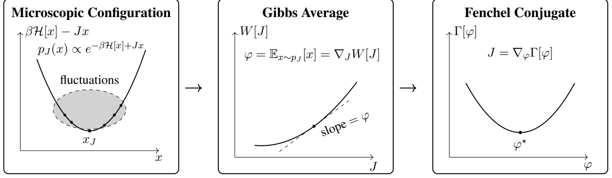
Figure 1: Illustration of the procedure from the microscopic to macroscopic energy landscapes. Left. “(Microscopic) Fluctuations” means x is random, has nonzero variance, and follows Gibbs distribution p_J(x) . Built from microscopic x , the local stable point x_J exhibits randomness. Middle. W[J] = \log(\int_{\mathcal{X}} \exp\{-\beta\mathcal{H}[x] + Jx\}) encodes macroscopic responses, i.e., \varphi = \mathbb{E}_{x \sim p_J}[x] = \nabla_J W[J] . Hence, the slope of W[J] gives a deterministic average. Right. \Gamma[\varphi] = \sup_J \{J\varphi - W[J]\} is the Fenchel conjugate of W[J] . Its response is J = \nabla_{\varphi} \Gamma[\varphi] , so local stable macroscopic points occurs at J = 0 . \Gamma[\varphi] describes the energy landscape built from macroscopic \varphi after integrating out microscopic fluctuations.
