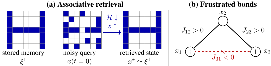
Figure 6: Retrieval and frustration in the classical Hopfield picture. (a) From a noisy query set, we retrieve a stored pattern by minimizing \mathcal{H} . Equivalently, the overlap increases during this associative retrieval. (b) Two ferromagnetic bonds and one antiferromagnetic bond on a triangle is impossible to satisfy pairwise energy minimization simultaneously. This is the simplest illustration of frustration.
