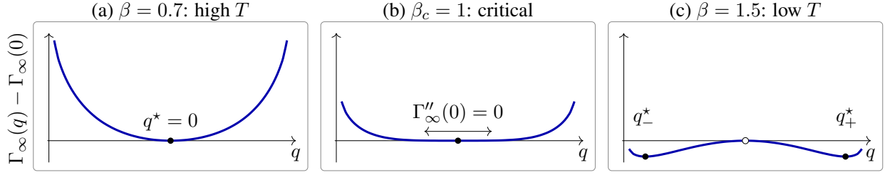
Figure 7: One-pattern free-energy landscape in the large- d limit. The curves show the one-pattern Hopfield model free energy and its local minima. Cooling the system turns the minimum at q^* = 0 into two retrieval minima.
