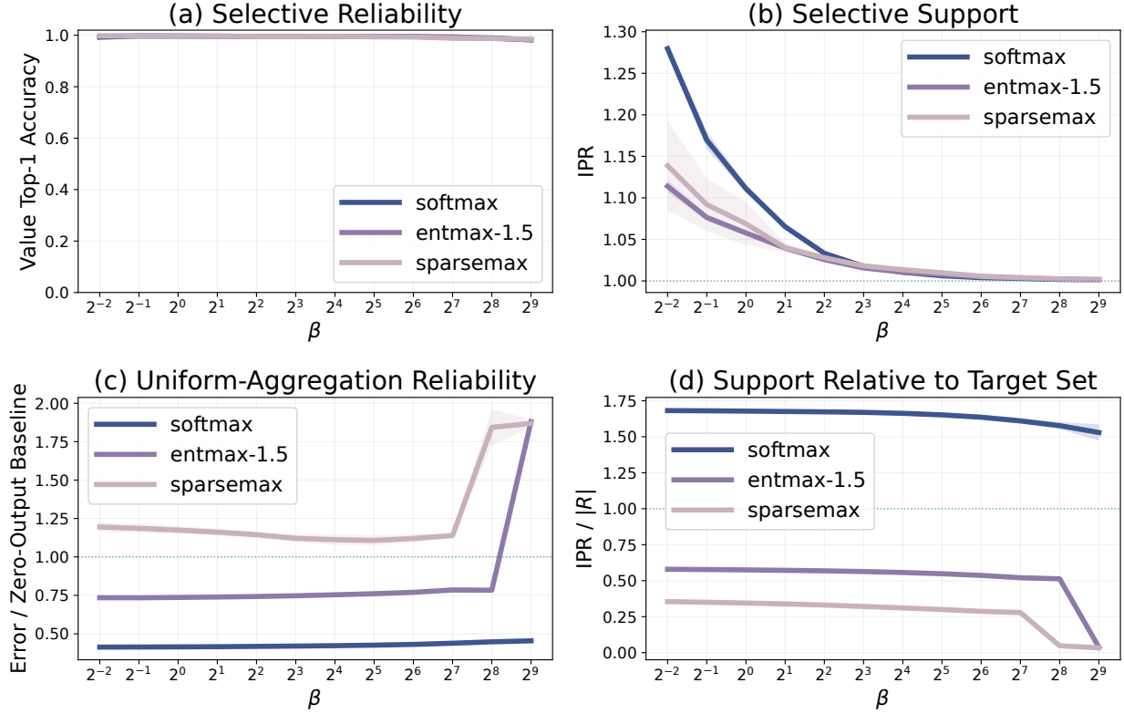
Figure 15: Temperature effect on matched-parameter Transformer. We train the Transformer parameters at each \beta , then we evaluate with M = 128 during inference. (a). All three attention families maintain high accuracy in a selective retrieval task. (b). Sparsemax and entmax-1.5 are support-efficient in a selective retrieval task. (c). Softmax has the highest reliability among the three in a uniform-aggregation task. (d). Softmax uses numerous memories, which indicates a poor support-efficiency.
