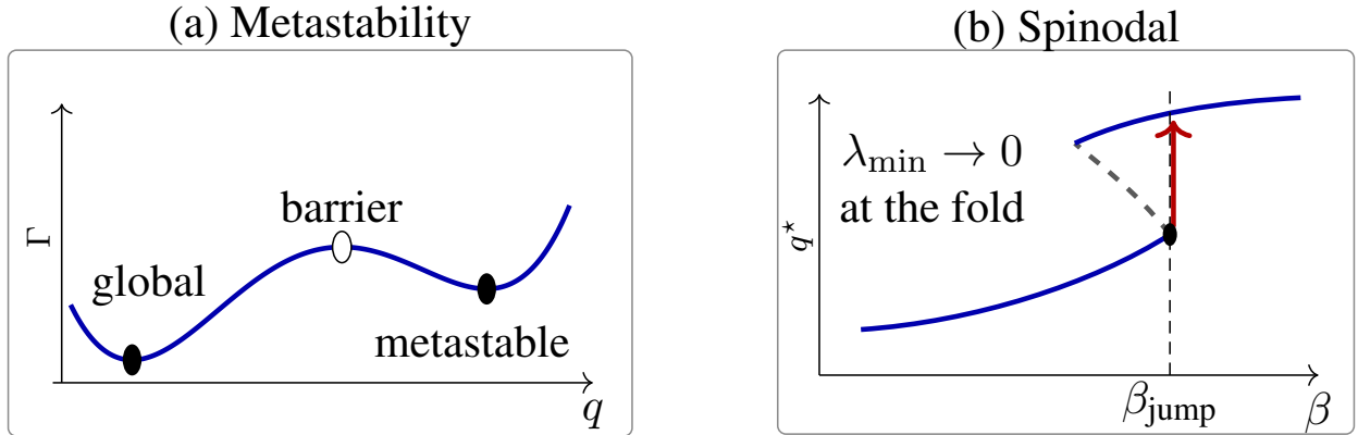
Figure 8: Phase-transition picture. (a) A metastable minimum is protected by a barrier. (b) We plot two smooth branches. In one smooth branch, the minimal Hessian eigenvalue vanishes at a spinodal. This leads to a jump onto another branch.
