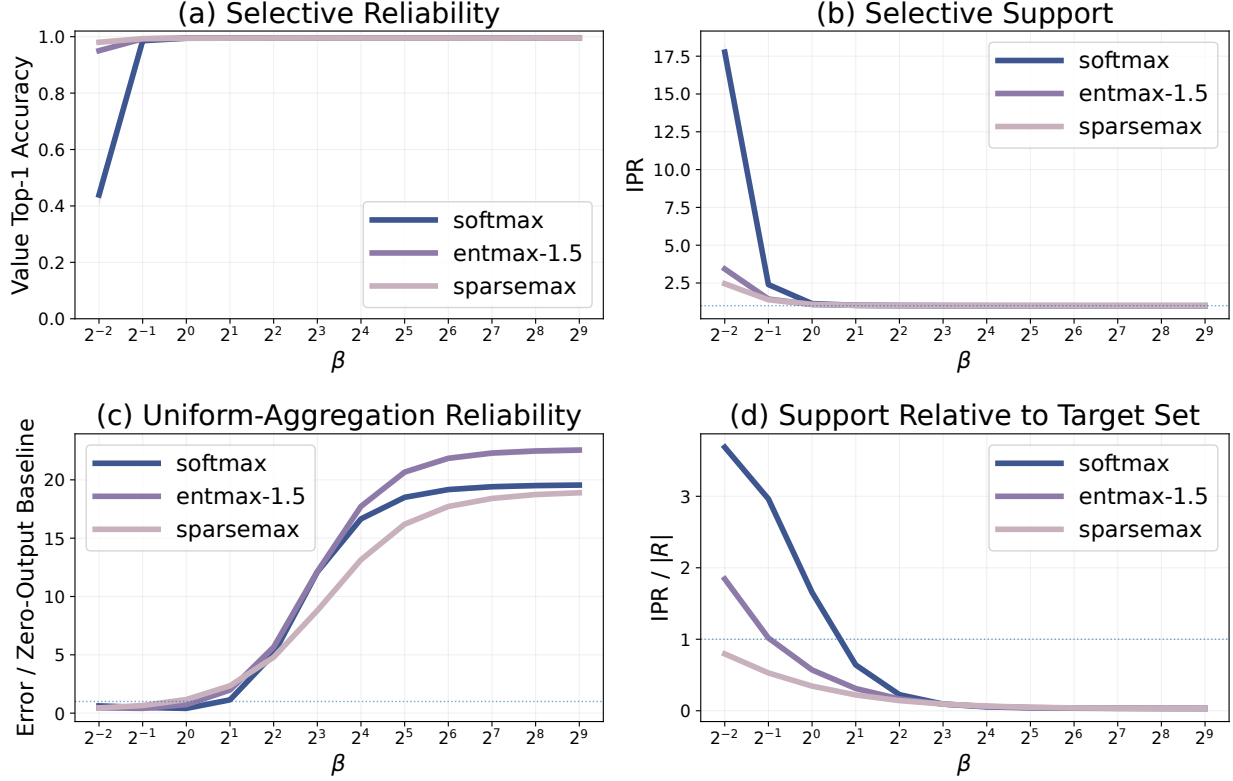
Figure 14: Temperature effect on frozen-parameter Transformer. We train the Transformer parameters at \beta_{\text{train}} = 1 , then we fix those parameters, set M = 128 and vary \beta during inference. (a). The three attention families both exhibit high accuracy for a selective retrieval task. (b). For selective retrieval, the sparsemax uses the least effective support size (IPR), which shows the support-efficiency and reliability of high- \beta sparsemax. (c). For a uniform-aggregation task, the three attention families have worse error relative to the zero-output baseline as \beta increases. (d). The IPR relative to target-set size decline as \beta grows, which indicates that the retrieval becomes selective. This leads to a mismatch for multi-memory aggregation.
