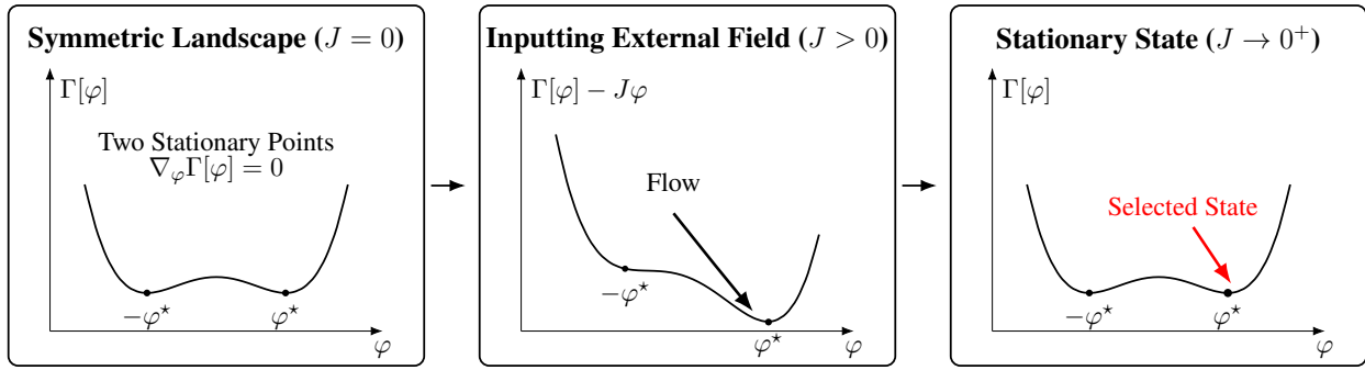
Figure 9: Selection of a stationary state by an external source. This figure illustrates how a source J selects one state from multiple degenerate stationary states of the free energy \Gamma[\varphi] . Left. When J = 0 , \Gamma[\varphi] is symmetric and has two degenerate local minima \pm\varphi^* . Middle. Turning on a small external source J > 0 tilts the landscape to \Gamma[\varphi] - J\varphi . This breaks the symmetry so that +\varphi^* becomes preferred. Then, the system flows toward the selected basin. Right. After the selection, we take the limit J \rightarrow 0^+ . Although the explicit source is removed, the system remains in the chosen local minimum +\varphi^* satisfying \nabla_\varphi \Gamma[+\varphi^*] = 0 . This source-selection procedure resolves the degeneracy between degenerate stationary states and specifies the retrieval state.
