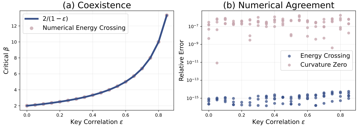
Figure 16: Two-key coexistence and spinodal validation. We consider two unit keys with correlation \epsilon . (a). The solid blue curve presents \beta_{\text{coexist}} = 2/(1 - \epsilon) . The numerical points are the root of the free energy difference \Delta\Gamma(\widehat{\beta}_{\text{coexist}}) = 0 . The numerical energy crossings coincide with the theoretical curve over the full correlation range. (b). We plot the relative errors of energy crossing (coexistence) and curvature zero (spinodal). The low values validate the theoretical formulas in Proposition 4.1 and Proposition 4.2 .
