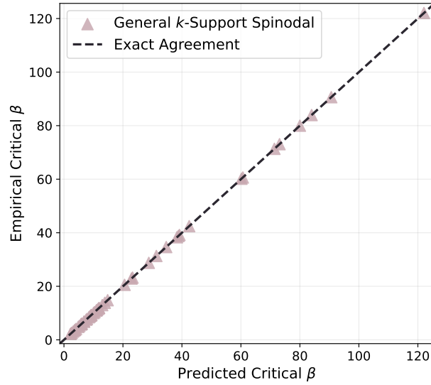
Figure 17: General k -support spinodal validation. We test the general k -support spinodal formula \beta_{\text{jump}} = 2/\lambda_{\max}(PGP) . We consider 50 systems with unit keys. The numerical points agree with the theoretical values, which validates Proposition 4.2 .
