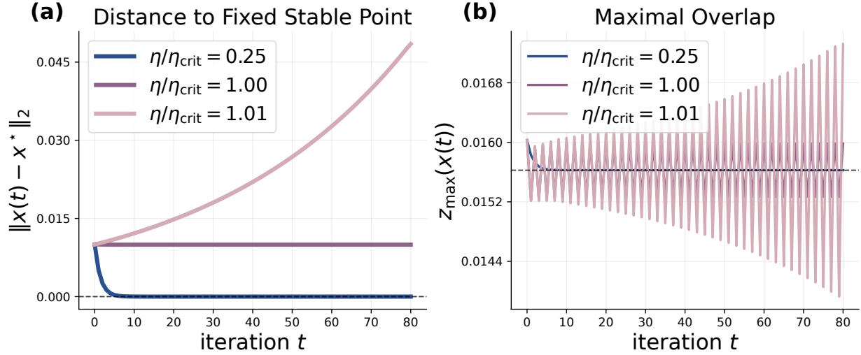
Figure 10: Dynamical retrieval stability of MHM gradient descent in the sparse regime ( \alpha = 2 ). ( M = 100, d = 64 ). We study the gradient descent update x(t+1) = x(t) - \eta \nabla \Gamma_{\alpha}^{(\text{mod})}(x(t)) . We denote the critical learning rate as \eta_{\text{crit}} = 2/\lambda_{\text{max}}(\nabla^2 \Gamma_{\alpha}^{(\text{mod})}(x^*)) with \lambda_{\text{max}} the largest eigenvalue at a fixed stable point x^* . (a) Distance to the fixed point. For \eta < \eta_{\text{crit}} , the training converges to the fixed point. Otherwise, the dynamics is unstable or even diverges. Maximal overlap. For \eta < \eta_{\text{crit}} , the training converges to the fixed value of overlap z_{\text{max}} \approx 0.0156 . It is the saturation value of one-pattern perfect retrieval in Figure 2 (a). Otherwise, the dynamics is unstable or even diverges.
