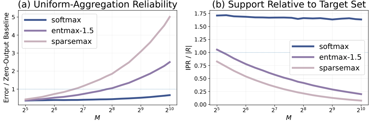
Figure 13: Capacity-reliability trade-off for uniform-aggregated retrieval. We evaluate the trained Transformer at fixed \beta_{\text{train}} = 1 while increasing M . (a). We measure the ratio of the output error and the zero-output baseline to characterize the retrieval reliability. Sparsemax exhibits the worst reliability. Furthermore, their retrieval reliabilities become worse as M grows, indicating the capacity-reliability trade-off. (b). Softmax support remains full, while sparsemax use the least supports and is the most support-efficient.
