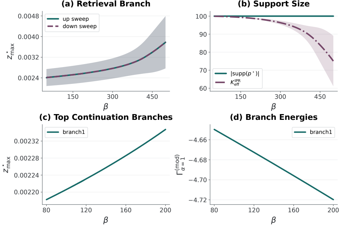
Figure 3: Temperature analysis of the retrieval structure of MHM in the dense regime ( \alpha = 1 ). ( M = 100, d = 64 ). Results are averaged over 10 random pattern realizations, and shaded regions indicate one standard deviation across different seeds. (a) Retrieval branches. The maximal overlap z_{\max}^* under up- and down-sweeps of \beta shows no hysteresis. (b) Support size. We compare the exact support size (active components of the probability distribution p ) and the inverse participation ratio (IPR) (Section F.2). (c) Top branches. We observe one single stable branch across the entire range of \beta . (d) Branch energies. We show the corresponding free energy of the branch.
