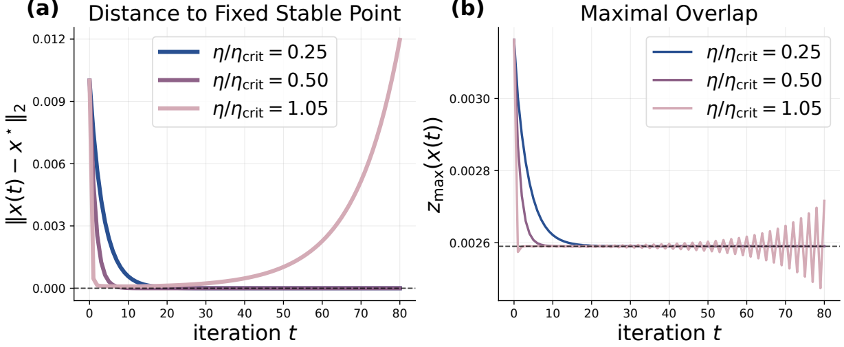
Figure 11: Dynamical retrieval stability of MHM gradient descent in the dense regime ( \alpha = 1 ). ( M = 100, d = 64 ). We study the gradient descent update x(t+1) = x(t) - \eta \nabla \Gamma_{\alpha}^{(\text{mod})}(x(t)) . We denote the critical learning rate as \eta_{\text{crit}} = 2/\lambda_{\text{max}}(\nabla^2 \Gamma_{\alpha}^{(\text{mod})}(x^*)) with \lambda_{\text{max}} the largest eigenvalue at a fixed stable point x^* . (a) Distance to the fixed point. For \eta < \eta_{\text{crit}} , the training converges to the fixed point. For \eta > \eta_{\text{crit}} , a divergence follows after a decay. This reflects that the iterate close to x^* initially. After this, the unstable eigen-directions start to dominate. We provide the precise explanation in this section. (b) Maximal overlap. For \eta < \eta_{\text{crit}} , the training converges to the fixed value of overlap z_{\text{max}} . For \eta > \eta_{\text{crit}} , a growing oscillations follow after an initial convergence. This is similar for the behavior in the distance plot.
