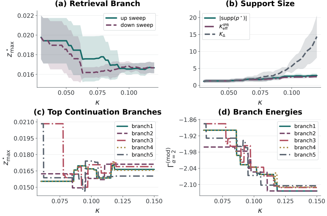
Figure 4: Memory-load analysis of the retrieval structure of MHM in the sparse regime ( \alpha = 2 ). ( d = 48, \beta = 180 ). Results are averaged over 10 random pattern realizations, and shaded regions indicate one standard deviation across different seeds. (a) Retrieval branches. The maximal overlap z_{\max}^* under up- and down-sweeps of \kappa shows hysteresis. (b) Support size. We compare the exact support size |\text{supp}(p^*)| (active components of the probability distribution p ) and the inverse participation ratio (IPR) (Section F.2). (c) Top branches. We track the top five stable branches ranked by z_{\max}^* . (d) Branch energies. We plot the corresponding free energy of the five branches.
