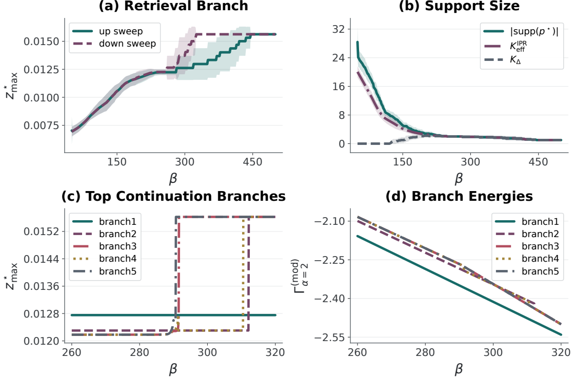
Figure 2: Temperature analysis of the retrieval structure of MHM in the sparse regime ( \alpha = 2 ). ( M = 100, d = 64 ). Results are averaged over 10 random pattern realizations, and shaded regions indicate one standard deviation across different seeds. (a) Retrieval branches. The maximal overlap z_{\max}^* under up- and down-sweeps of \beta exhibits hysteresis. (b) Support size. We compare the exact support size (active components of the probability distribution p ), the inverse participation ratio (IPR), and the fixed score-threshold count (Section F.2). (c) Top branches. We track the top five stable branches ranked by z_{\max}^* . (d) Branch energies. We show the corresponding free energies of those top five branches.
