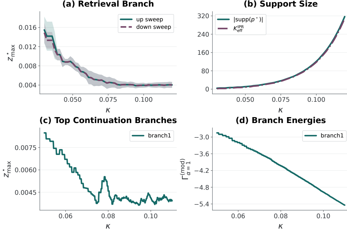
Figure 5: Memory-load analysis of the retrieval structure of MHM in the dense regime ( \alpha = 1 ). ( M = \exp(\kappa d) , d = 48 , \beta = 180 ). Results are averaged over random pattern realizations, and shaded regions indicate one standard deviation across different seeds. (a) Retrieval branches. The maximal overlap z_{\max}^* under up- and down-sweeps of \kappa shows no hysteresis. (b) Support size. We compare the exact support size (active components of the probability distribution p ) and the inverse participation ratio (IPR) (Section F.2). (c) Top branches. We track and observe only a single stable branch across the entire range of \kappa . (d) Branch energies. We plot the corresponding free energy of the branch.
