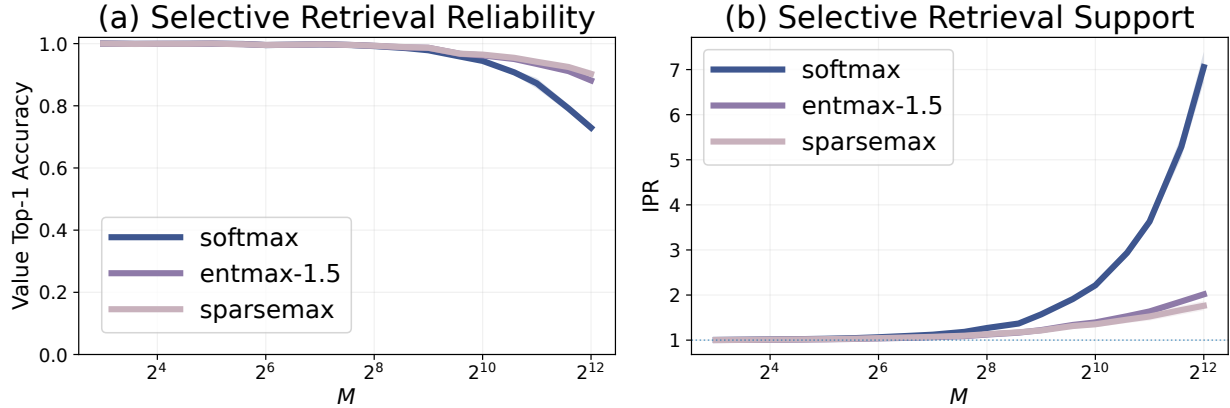
Figure 12: Capacity-reliability trade-off for selective retrieval. We evaluate the trained Transformer at fixed \beta_{\text{train}} = 1 while increasing M . (a). We measure the value top-1 accuracy to characterize the retrieval reliability. Sparsemax retain the highest accuracy. Furthermore, their accuracy decreases as M grows, indicating the capacity-reliability trade-off. (b). Softmax support remains full, while sparsemax use the least supports and is the most support-efficient.
