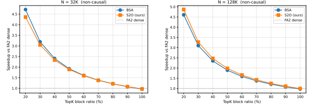
Figure 6 Comparison with BSA under matched sparsity. Speedup over FA2 dense under different TopK block ratios for non-causal attention. Left: sequence length N = 32K . Right: sequence length N = 128K . Under matched sparsity settings, S2O achieves runtime comparable to BSA, and the measured speedup remains largely aligned with the actual sparsity level. This suggests that sparsity beyond block granularity is practical and can be effectively translated into wall-clock acceleration.
