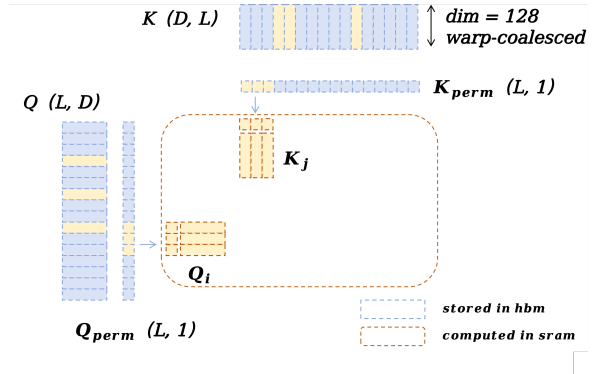
Figure 3 Coordinate-scheduled online Q/K permutation. Two lightweight index arrays Q_{\text{perm}} and K_{\text{perm}} are built without moving tensors. At runtime, indices directly address which tokens are loaded into on-chip SRAM for block attention. Since d = 128 , scattered token accesses still fully utilize a warp; see Appendix B for details.
