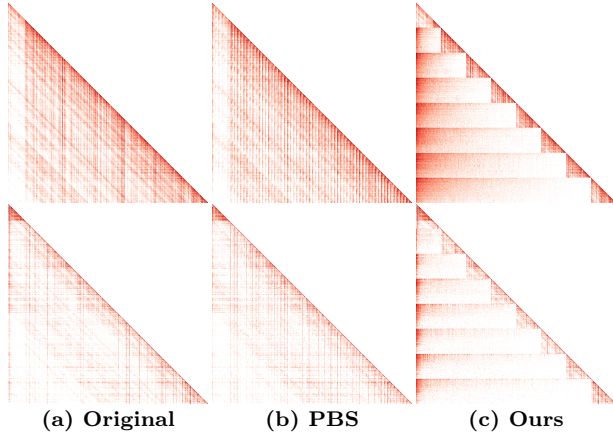
Figure 2 Attention heatmaps under different permutation strategies. (a) Original: The heatmap exhibits abundant line-level (stripe-like) structures. (b) PBS: Following PBS’s local K/V permutation strategy, the heatmap still contains substantial redundancy and fails to consistently emphasize salient horizontal stripes. (c) Ours: Our global permutation scheme (Sec. 3.1) compacts attention mass into a progressive region from dense (upper-left) to increasingly diffuse. More qualitative heatmaps are provided in Appendix D.
