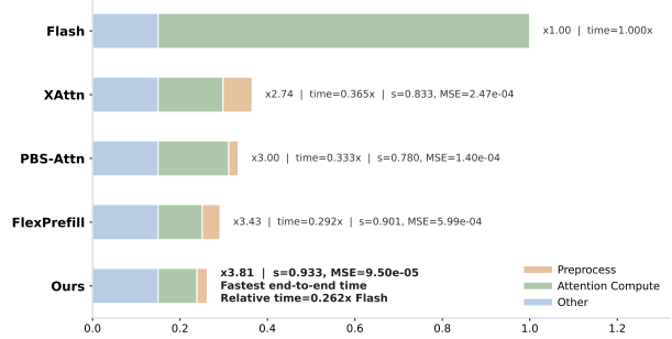
Figure 1 Speedup at 128K context length (Llama-3-8B) with sparsity–error trade-off. We report end-to-end latency speedup over FlashAttention and break down the major components, including sparse preprocessing time, attention compute time, and other overheads. We also show each method’s sparsity ratio and the corresponding mean squared error (MSE; lower is better), highlighting that our method achieves lower error at higher sparsity.
