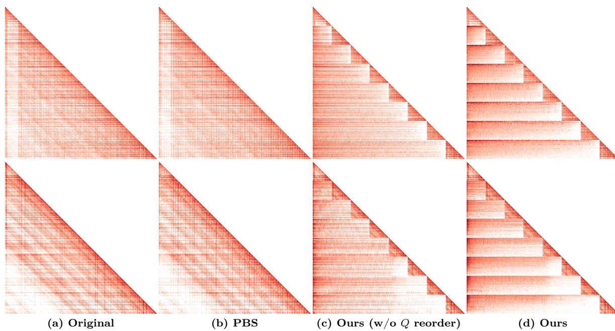
Figure 7 Additional attention heatmaps on Qwen3-8B under different reordering strategies.
