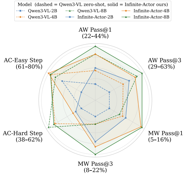
Figure 5: Performance comparison between zero-shot Qwen3-VL and Infinite-Actor agents across model scales (2B/4B/8B) on six evaluation metrics from Table 1: AW Pass@1 (AndroidWorld Pass@1), AW Pass@3, MW Pass@1 (MobileWorld Pass@1), MW Pass@3, AC-Easy Step SR (AC-Curated-Easy Step SR), and AC-Hard Step SR (AC-Curated-Hard Step SR). Infinite-Actor models consistently outperform their zero-shot counterparts on task-level benchmarks.
