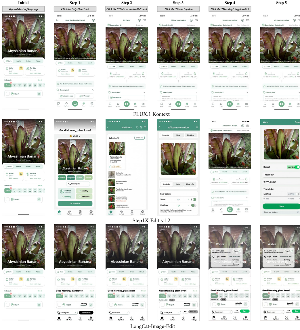
Figure 8: Qualitative comparison of multi-step rollout. (a) Part I shows outputs from FLUX.1 Kontext, Step1X-Edit-v1.2, and LongCat-Image-Edit for the five-step LeafSnap watering task; each column is a step. These baselines drift away from the intended UI state.
