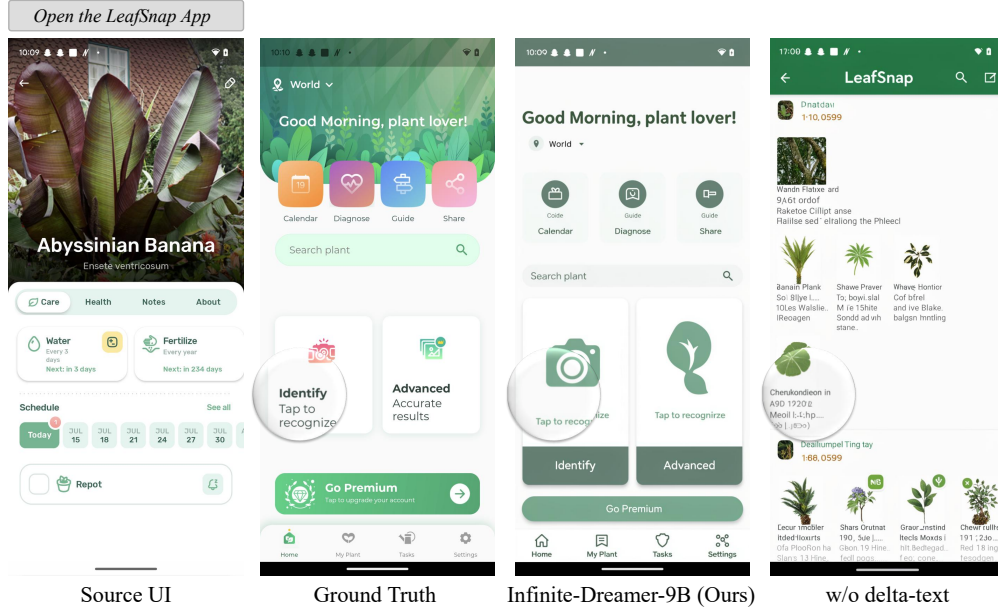
Figure 6: Qualitative effect of delta-text conditioning. Given the source UI (leftmost) and the delta-text action “Open LeafSnap App”, Infinite-Dreamer-9B (third) closely matches the ground-truth transition (second), whereas the variant without delta-text (rightmost, which only receives the trigger action/operation without any fine-grained descriptions of added or removed elements) collapses into an unrelated screenshot that diverges substantially from the intended target UI.
