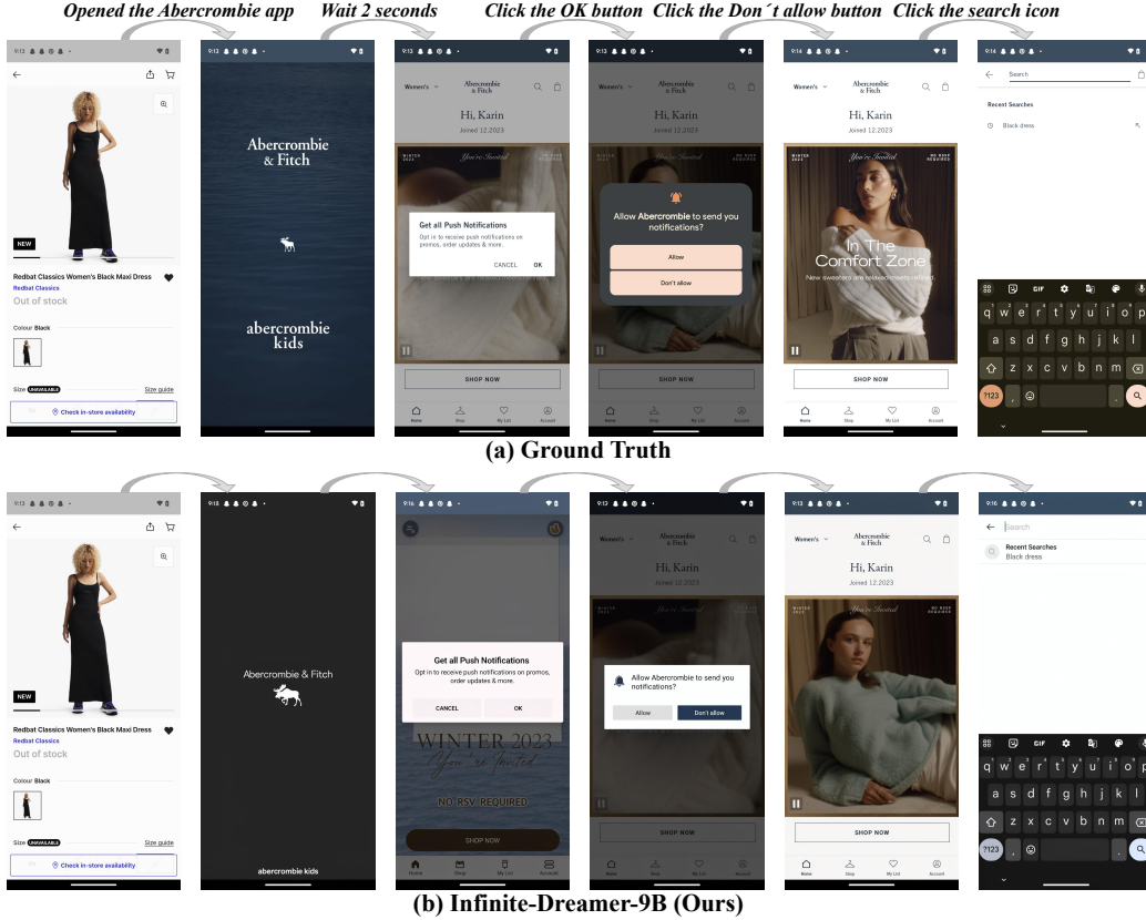
Figure 4: Qualitative synthesis comparison. (a) Ground Truth trajectory (top) versus (b) Infinite-Dreamer-9B (Ours) (bottom) over a 6-step GUI interaction sequence (from opening “Abercrombie” to clicking the search icon). Our model faithfully reproduces the real UI state transitions, maintaining layout accuracy, text fidelity, and visual coherence across all steps.
