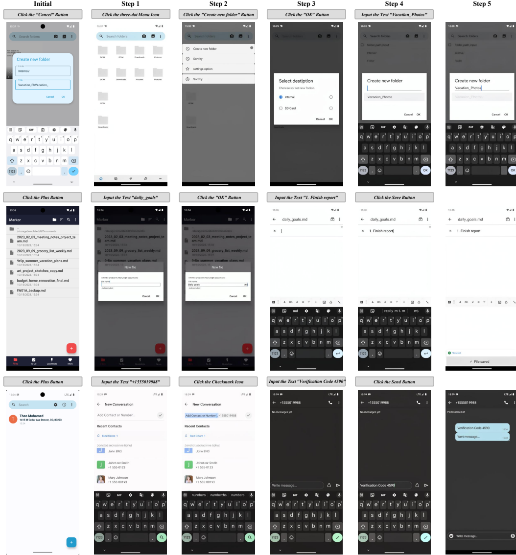
Figure 10: Multi-step imagination examples. Each row is an independent trajectory: starting from an Initial screenshot, Infinite-Dreamer autoregressively applies the delta-text action printed above each column (e.g., “Click the Create new folder Button”, “Input the Text daily_goals ”, “Click the Send Button”) to produce Step 1 through Step 5. The imagined screenshots keep the surrounding UI chrome stable while correctly rendering the widget or text that the action introduces.
