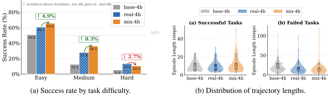
Figure 3: AndroidWorld analyses for base-4b, real-4b, and mix-4b.
