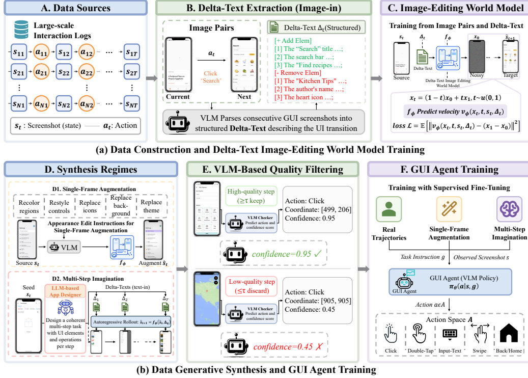
Figure 2: Overview of our proposed Infinite-Dreamer : (a) Data Construction and Delta-Text Image-Editing World Model Training. We extract structured delta-texts from real UI trajectories and fine-tune an instruction-guided image-editing model as a GUI world model; (b) Data Generative Synthesis and GUI Agent Training. The trained world model enables two synthesis regimes, namely single-frame augmentation and multi-step imagination, whose outputs are filtered by a VLM-based quality checker and used to train the GUI agent.
