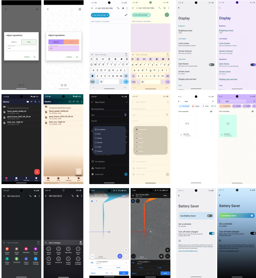
Figure 9: Single-frame augmentation examples. For each pair, the left column shows the source screenshot and the right column shows a visually distinct variant produced by Infinite-Dreamer. The pairs span multiple app categories and cover dark/light theme swap, accent-color and background recoloring, and icon/keyboard restyling, while widget positions and text content are held fixed.
