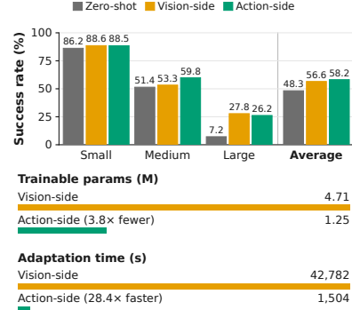
(b) Viewpoint-shift experiment results.
