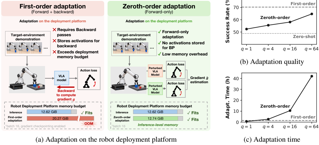
Figure 1: Zeroth-order adaptation enables on-robot adaptation within the inference memory budget. Unlike first-order adaptation, it requires only forward evaluations and avoids storing activations (a). Increasing the query budget q improves adaptation quality toward first-order performance, at the cost of increased adaptation time (b,c).
