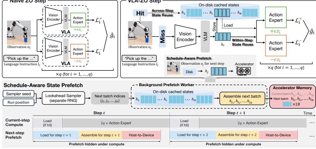
Figure 3: Overview of VLA-ZO.
