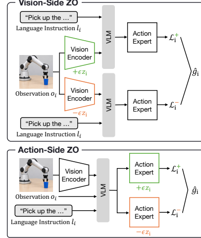
(a) ZO adaptation placement.
