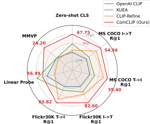
Figure 1: Multi-dimensional comparison on ViT-L/14 (values from Table 1). Relative to the original OpenAI CLIP, ComCLIP improves all four evaluation dimensions (zero-shot classification, retrieval, linear probing, MMVP), whereas prior post-training methods exhibit characteristic trade-offs. Each axis is min-max normalized per metric; ComCLIP’s MMVP is the 3-seed mean (Sec. 4.3).
