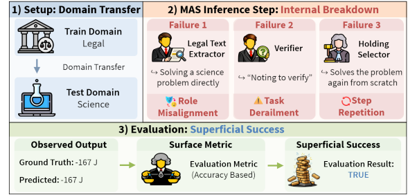
Figure 1: Example of superficial success vs. internal breakdown under domain transfer. When an adaptive MAS trained on the legal domain is applied to science, the agents make multiple errors during collaboration, yet the final answer remains correct due to the strength of individual LLMs—illustrating illusory coordination.
