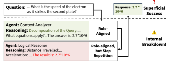
(b) Trained on common sense, tested on science domain
