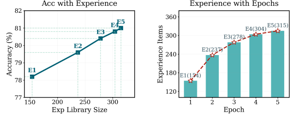
Figure 7: The size of the experience library varies with the number of mining epochs. The analysis experiments are conducted on the Qwen3-8B model and the MedQA dataset.
