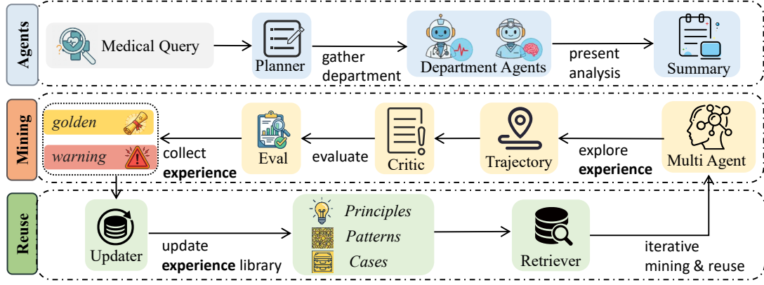
Figure 2: Our proposed EMR diagram. Agents correspond to Section 3.1 and represent the multi-agent collaborative system. Mining corresponds to Section 3.2 and focuses on analyzing multi-agent collaboration trajectories to mine experiential knowledge. Reuse corresponds to Section 3.3, where extracted experiences are integrated into an experience library and reused to guide subsequent tasks, enabling iterative mining and reuse.
