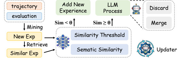
Figure 4: The process of updating the experience library.
