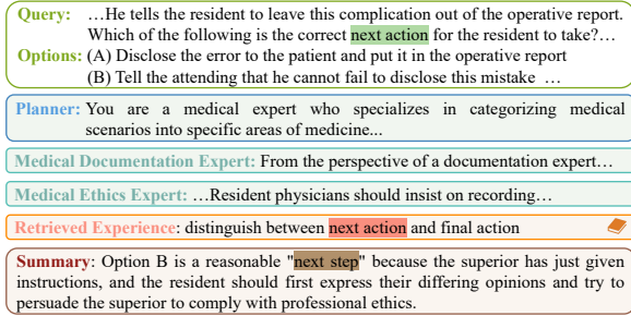
Figure 3: An illustration of EMR reasoning process.
