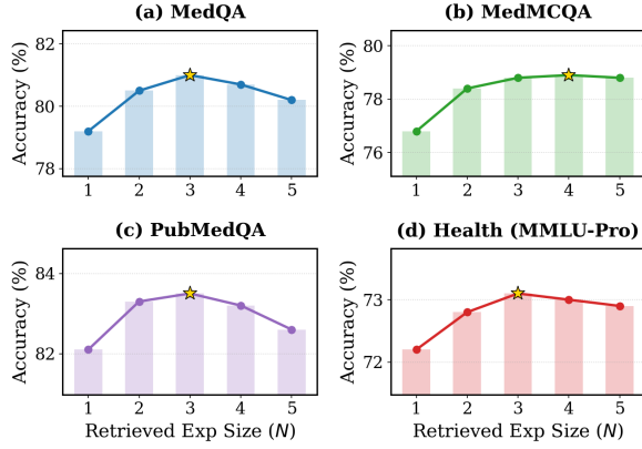
Figure 6: The impact of the number of retrieved experiences on performance. The ablation experiments are conducted using the Qwen3-8B model on the MedQA, MedMCQA, PubMedQA, and Health (MMLU-Pro) datasets.
