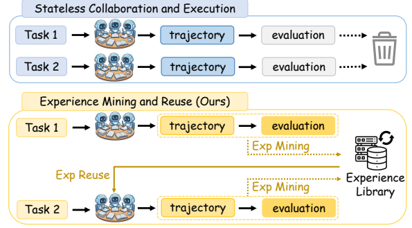
Figure 1: Illustration of the experience mining and reuse mechanism in EMR versus traditional instance-independent reasoning.
