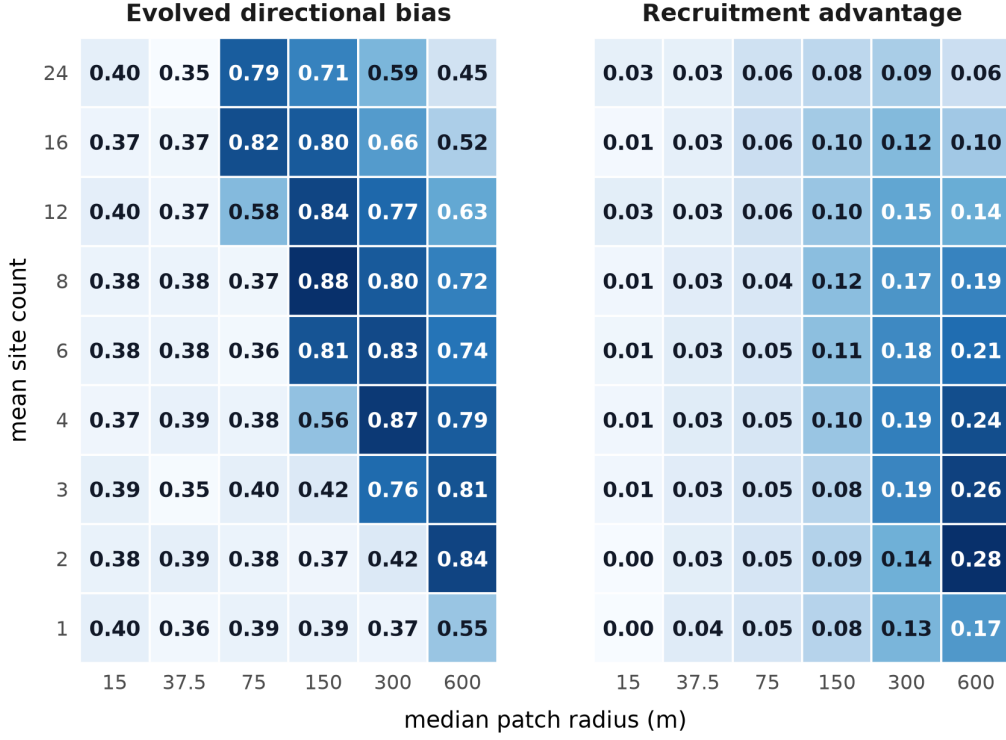
Figure 5: Evolved DIRECTIONAL BIAS (left) and recruitment advantage (right) on a flat comb across the grid of Poisson mean site count against median patch radius, 50 seeds per cell. Recruitment advantage is the follower–searcher success difference, and shading is normalized within each panel.
